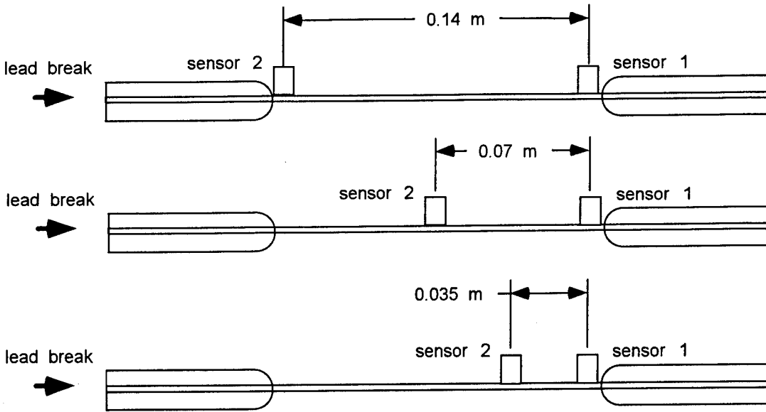
Figure 6.1, Distance Resolution Test, Carbon Fiber Sample
