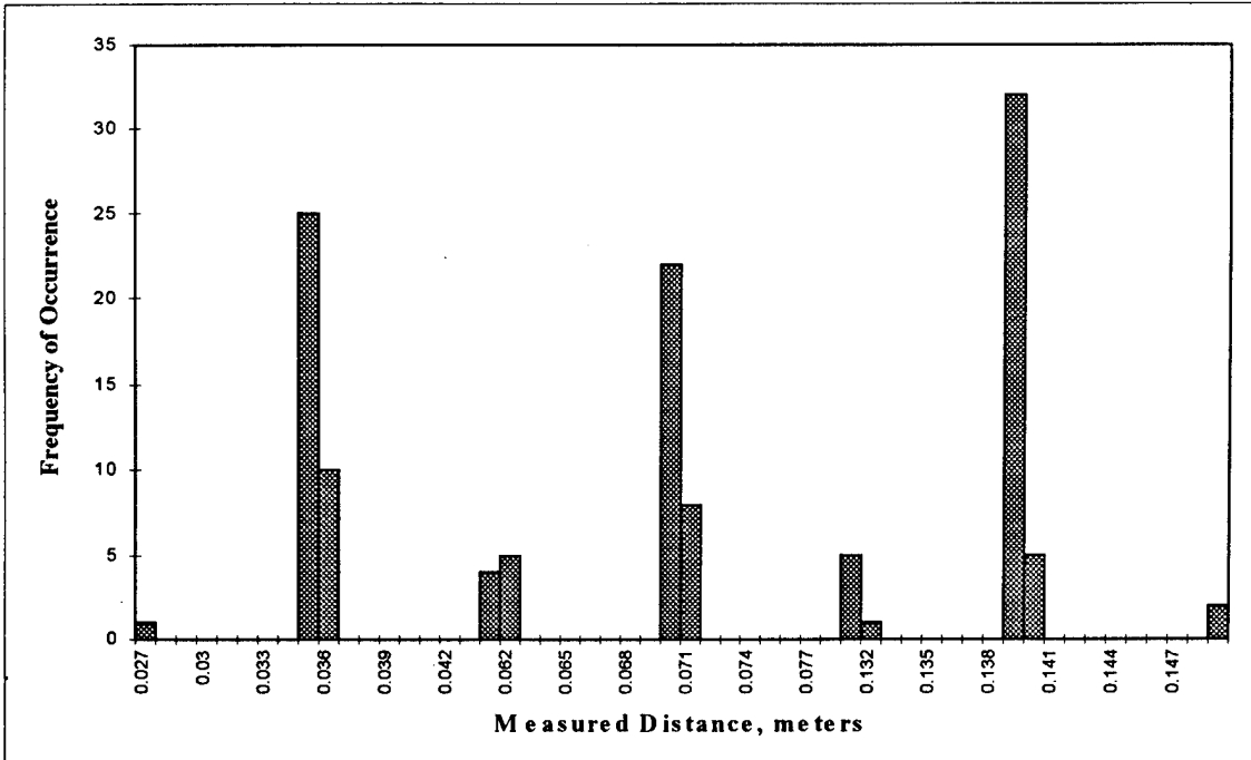
Figure 6.5, Carbon Fiber Threshold Crossing, 8,700 m/s
