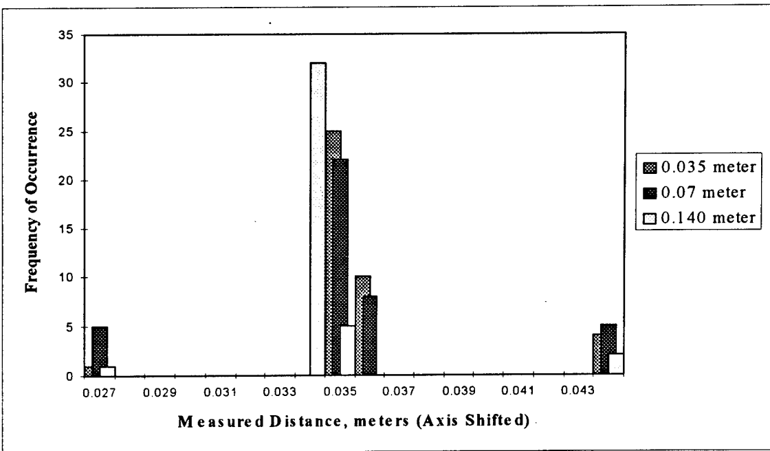
Figure B.4, Carbon Fiber, Threshold Crossing, 8,700 meters / second, (Standardized)
