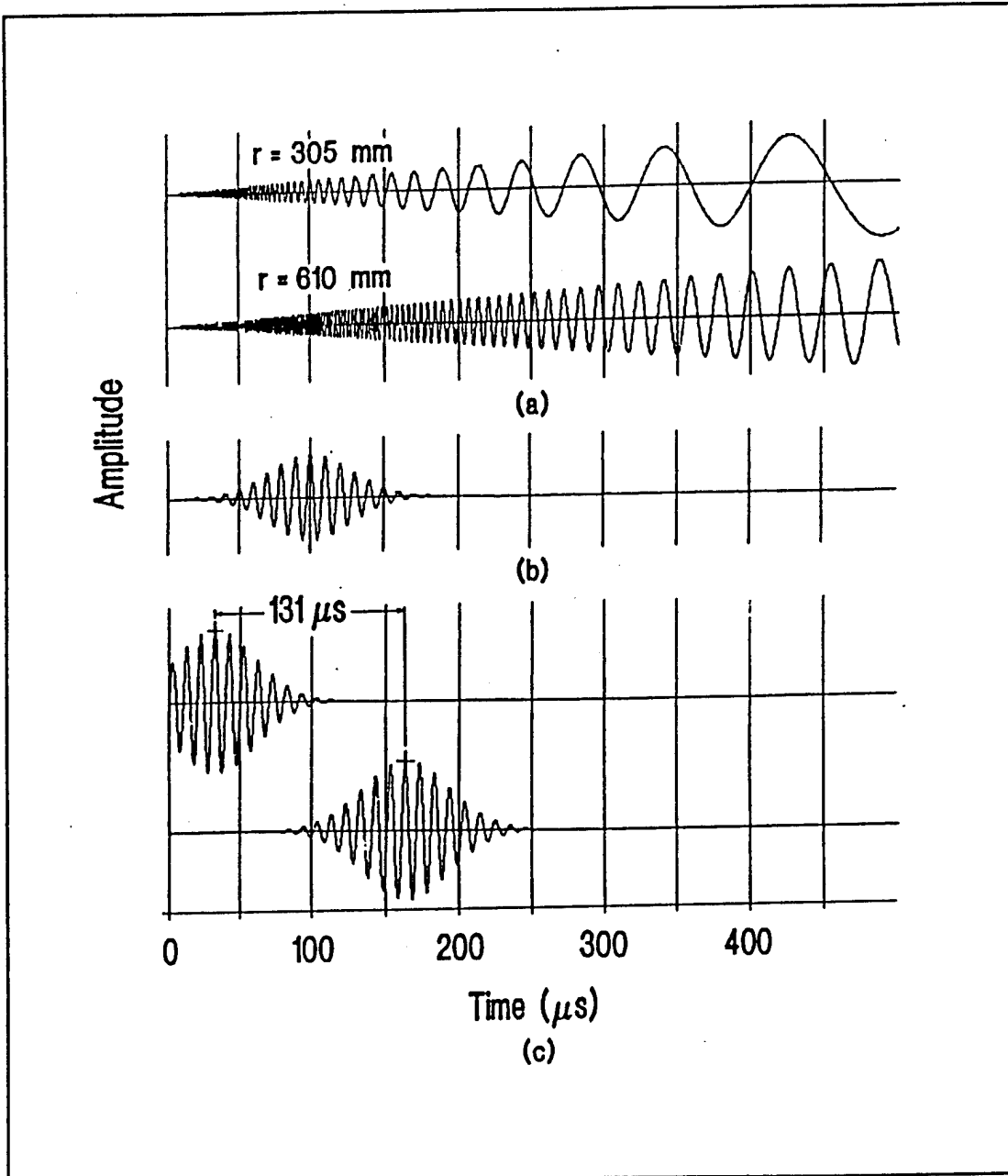
Figure 3.2, Cross Correlation Analysis ( from Ziola, 1991)
