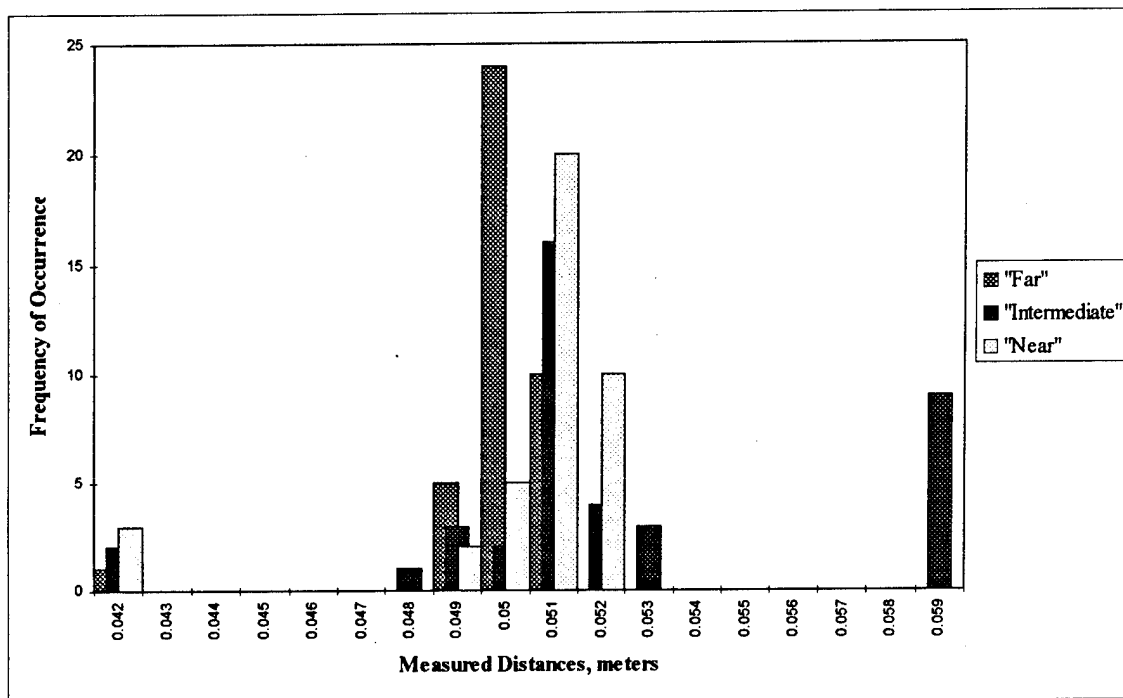
Figure 5.9, 3/8" Steel Rod, Threshold Crossing, 5,300 m/s
