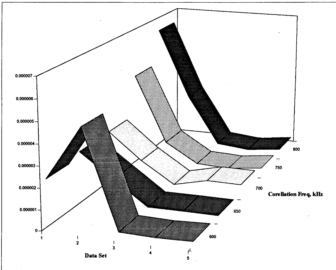
Figure B.2, Standard Deviation
