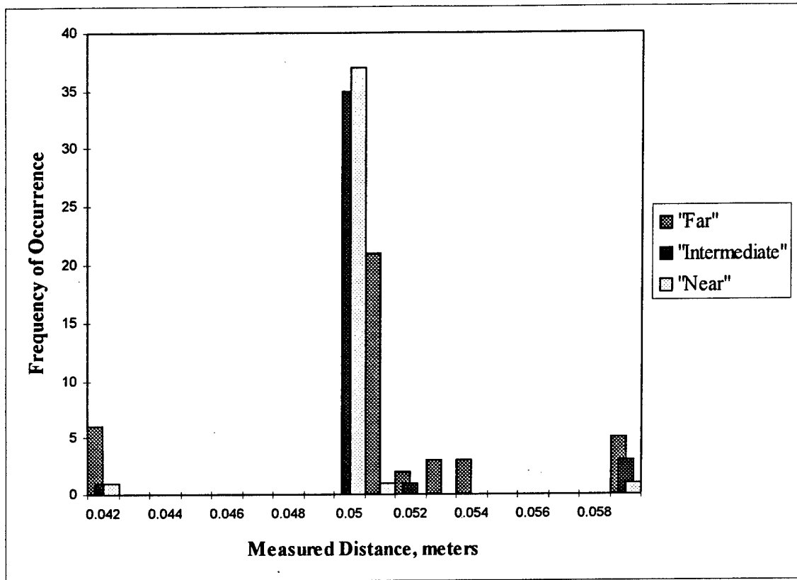
Figure 5.11, 1/8" Steel Rod, Threshold Crossing, 5,145.6 m/s
