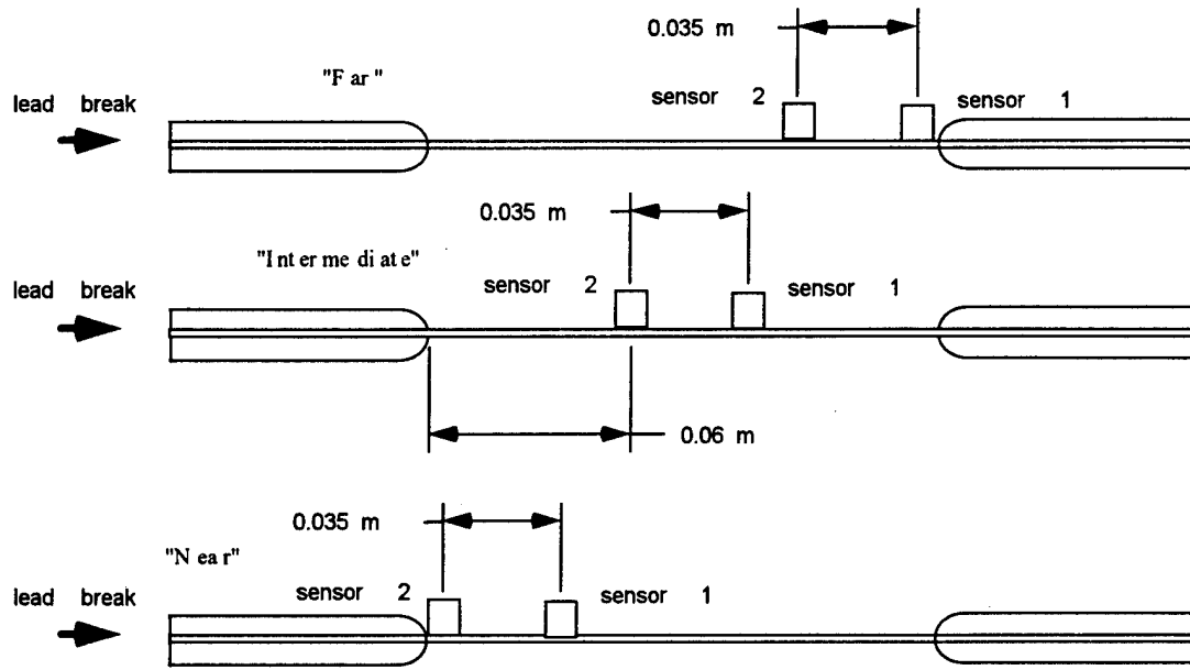
Figure 6.7, Dispersion Test Configuration, Carbon Fiber Sample
