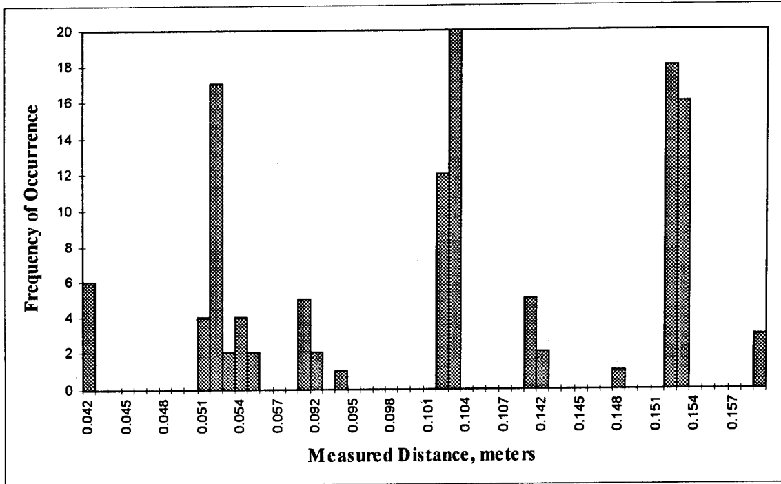
Figure 5.4, 1/8" dia Steel Rod, Threshold Crossing, 5,300 m/s
