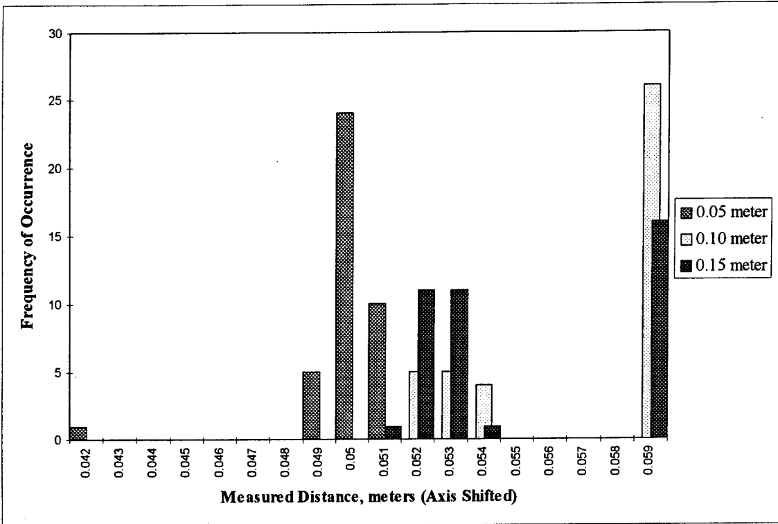
Figure 5.3, 3/8" dia Steel Rod, Threshold Crossing, 5,300 m/s (Standardized)
