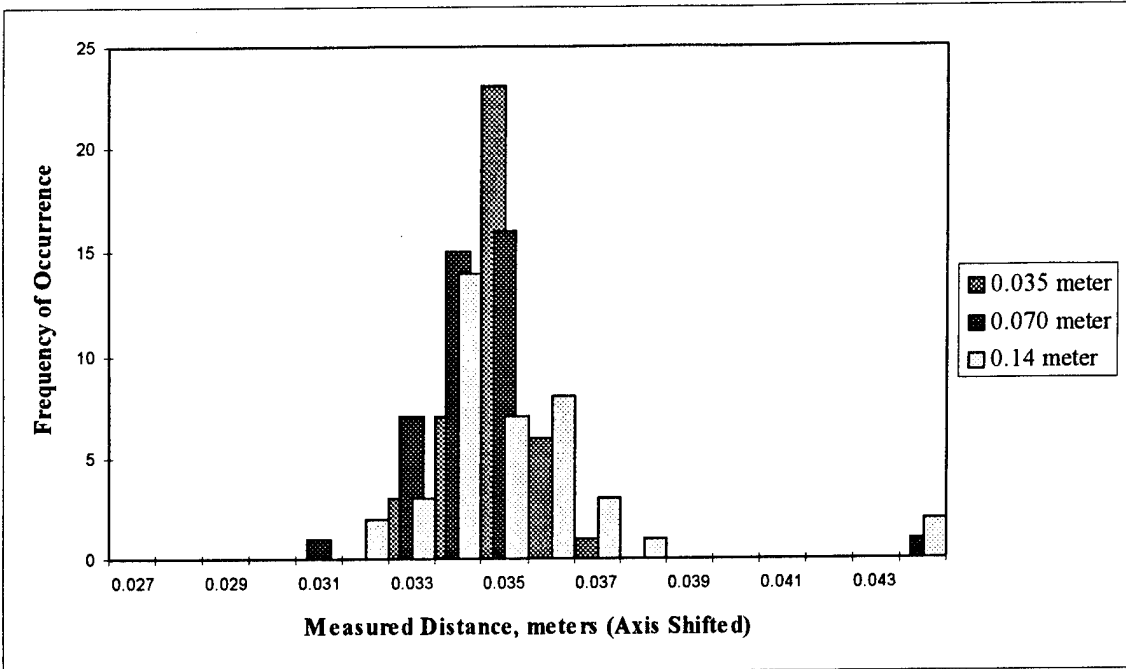
Figure B.3, Carbon Fiber, Gauss Cross Correlation @700 kHz, 8,700 m/s (Standardized)
