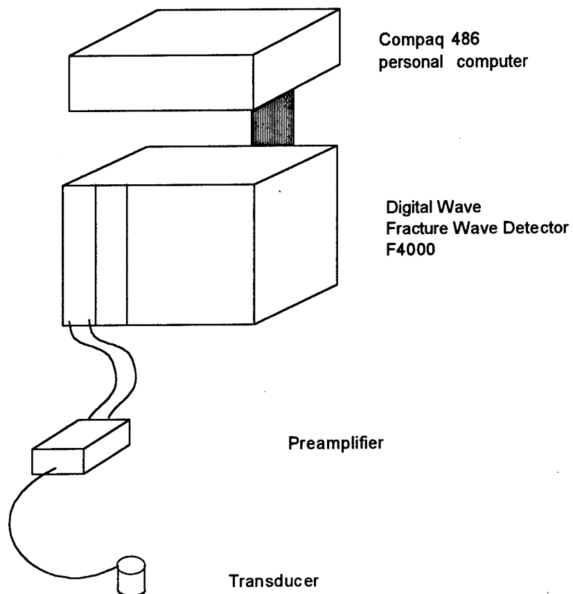
Figure A.1, Basic Componentry and Layout of Acoustic Emission Equipment
