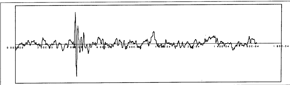
Figure 6.2, Example Waveform in Carbon Fiber, Measured at Center of Strand
