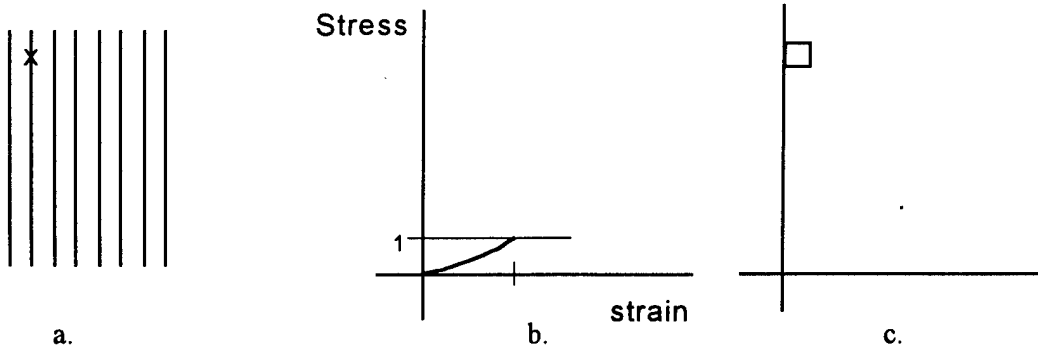
Figure 1.1, Composite Fiber Model
