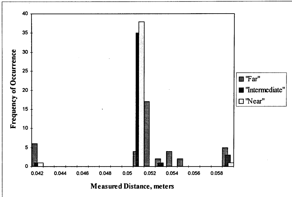
Figure 5.10, 1/8" Steel Rod, Threshold Crossing, 5,300 m/s
