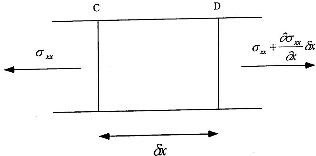
Figure 2.2 Forces Acting on a Rod in Longitudinal Stress(after Kolsky, 1963)
