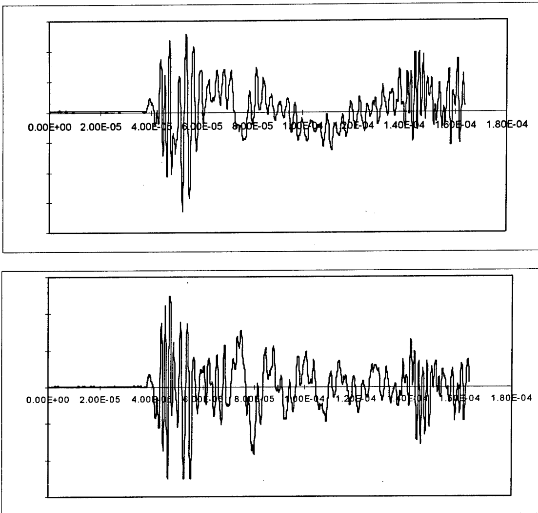
Figure 4.2, Unfiltered (top) and Filtered Waveforms, 0.05 meter from source event
