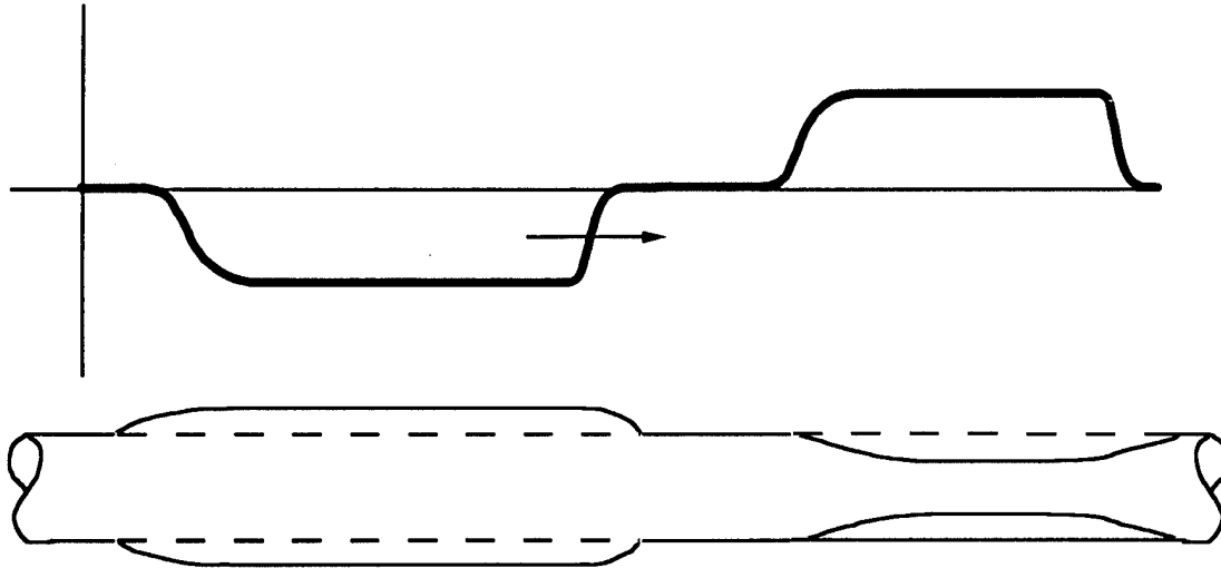
Figure 4.5, Poisson Effect from Longitudinal Stress Pulses(from Graff, 1991)
