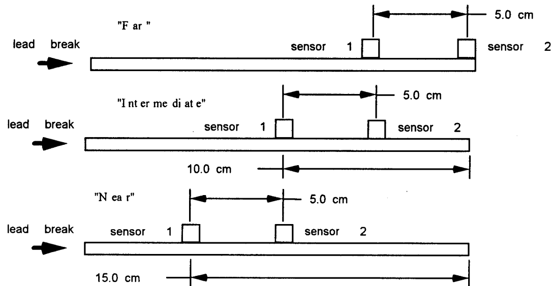
Figure 5.8, Dispersion Tests
