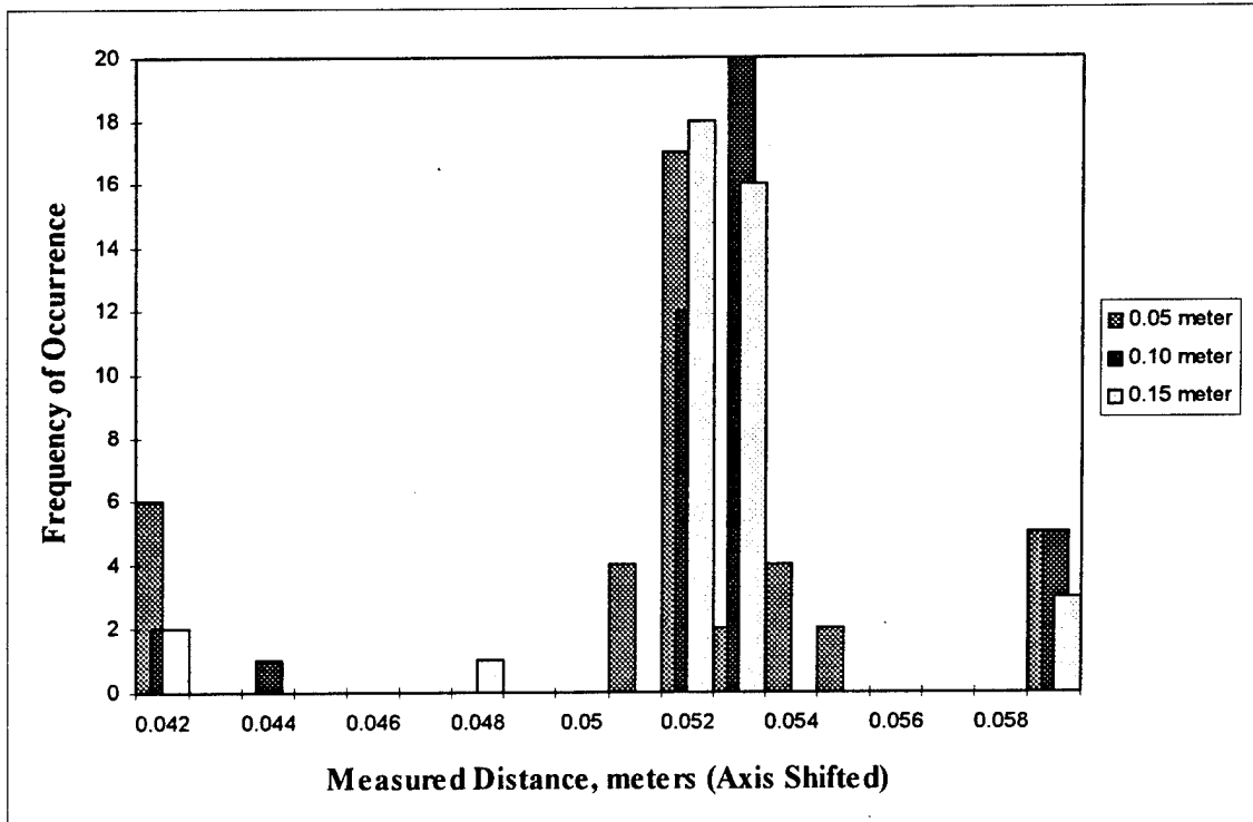
Figure 5.5, 1/8" dia Steel Rod, Threshold Crossing, 5,300 m/s (Standardized)
