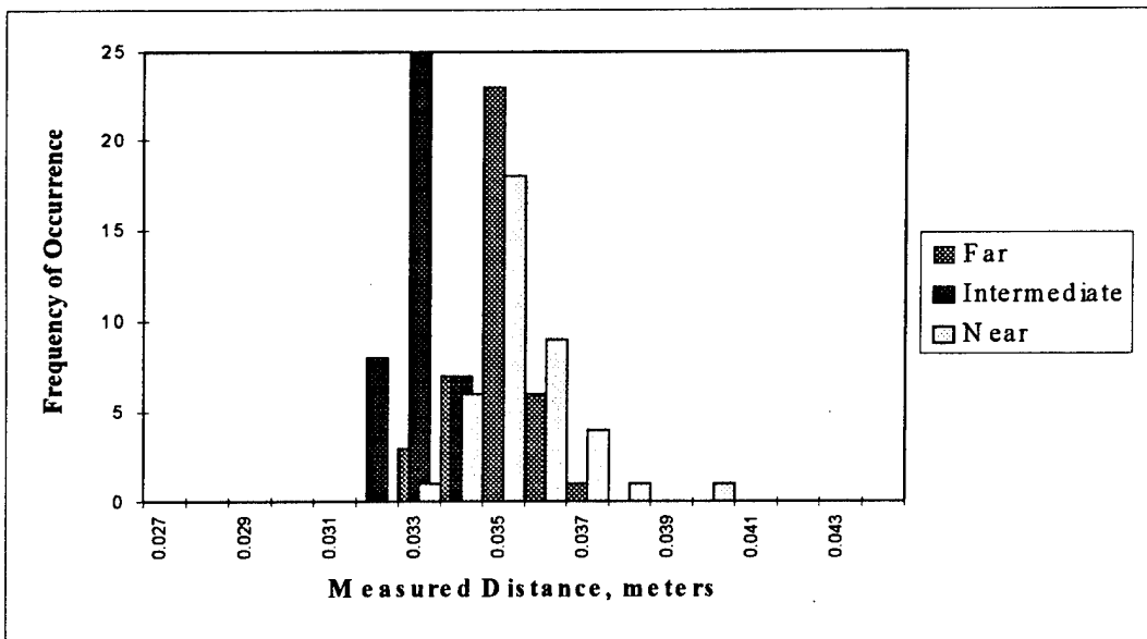
Figure 6.9, Gaussian Cross Correlation 8,700 m/s @ 700 kHz
