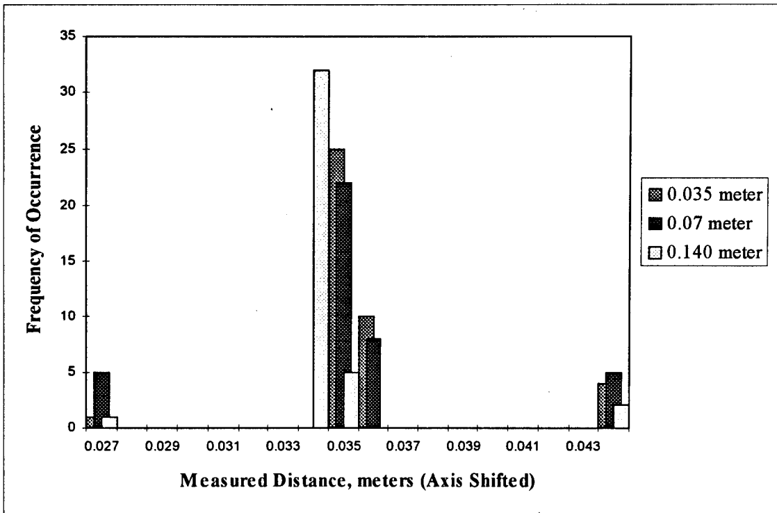
Figure 6.6, Carbon Fiber, Threshold Crossing 8,700 m/s (Standardized)
