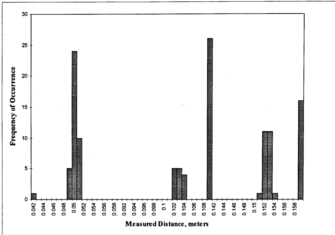
Figure 5.2, 3/8" dia. Steel Rod, Threshold Crossing, 5,300 m/s
