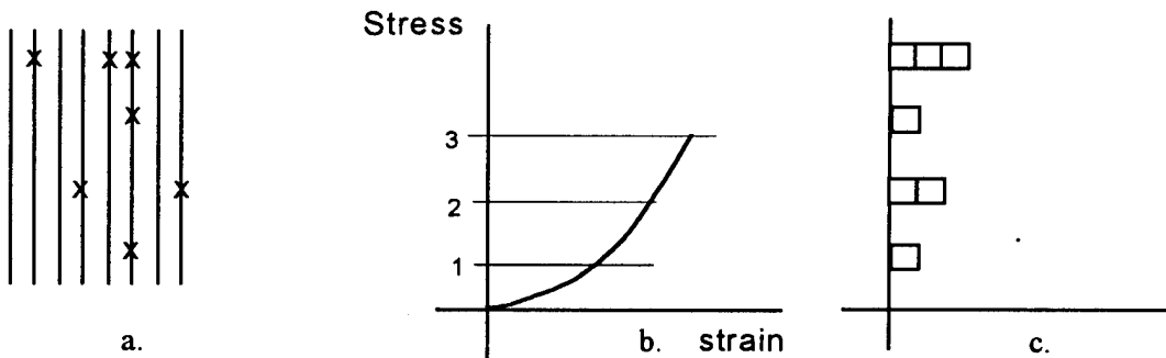
Figure 1.3, Composite Fiber Model
