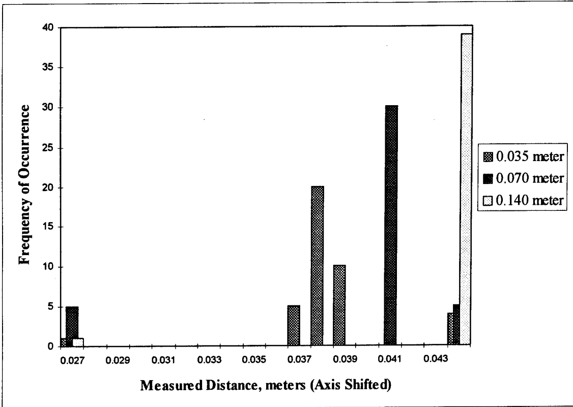
Figure 6.4, Carbon Fiber Distance Resolution 10,000 m/s (Standardized)
