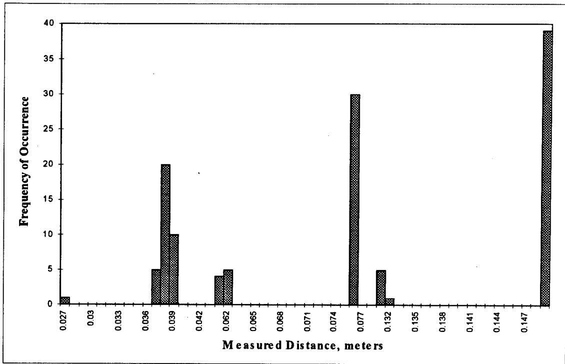
Figure 6.3, Carbon Fiber Distance Resolution, 10,000 m/s
