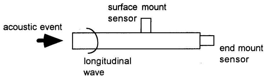
Figure 4.4, Detection of Extensional Waves
