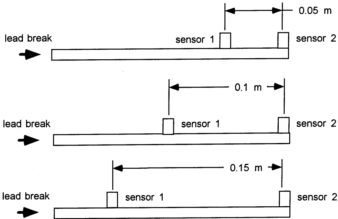
Figure 5.1, Resolution and Repeatability Tests
