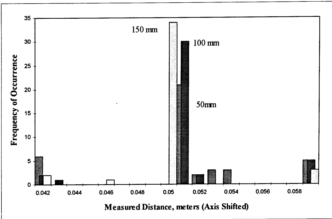
Figure 5.7, 1/8" Steel Rod, Threshold Crossing, 5,145.6 m/s (Standardized)
