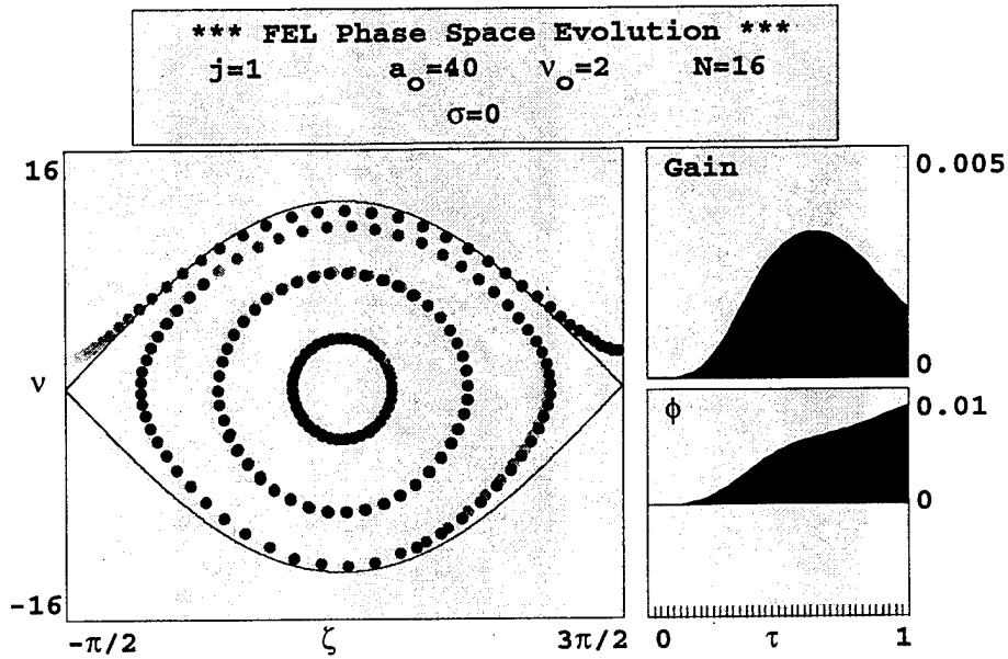
Figure 11. Phase-space evolution showing trapped-particle instability in an untapered undulator.
