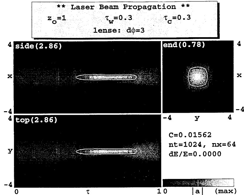
Figure 3. Propagation path with a converging lens.
