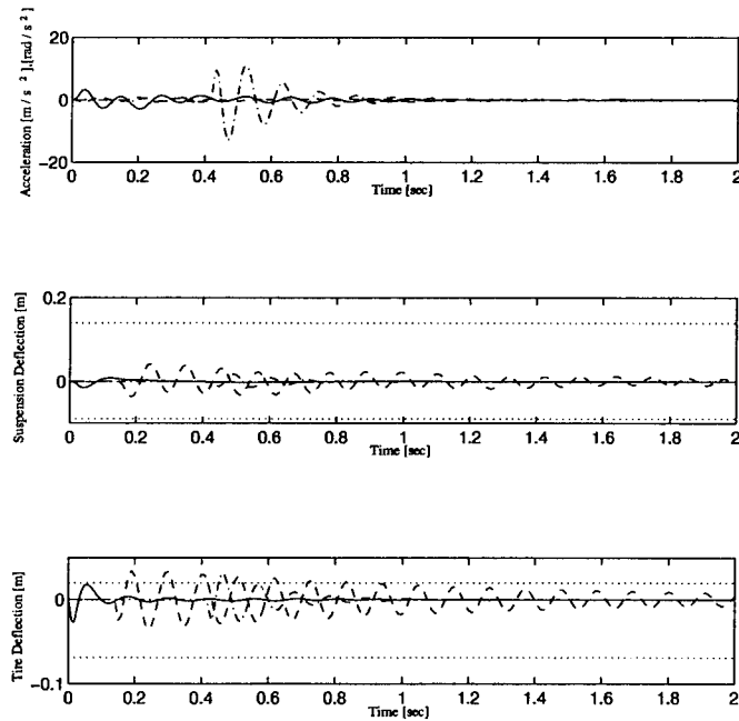
Figure E.3: Ten DOF Open-Loop - Empty Configuration - Small Rounded Pulse Input
