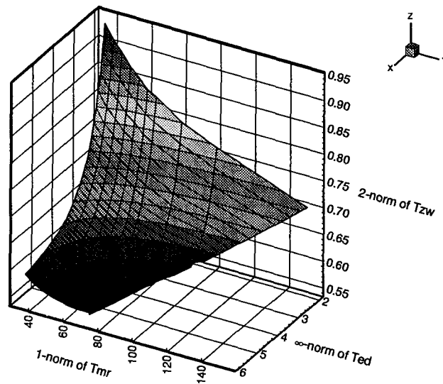
Figure 3.4: Edgeworth-Pareto Surface
