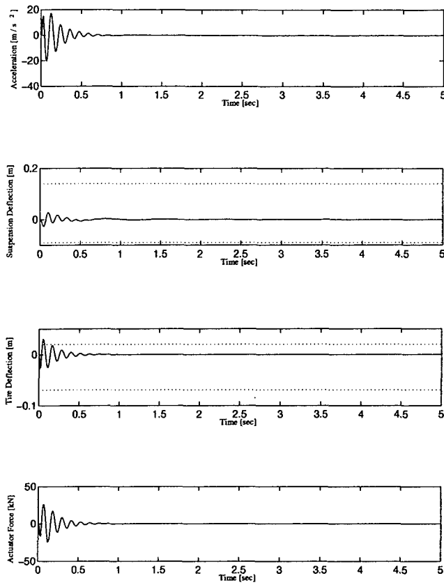
Figure G.2: Mixed-Design 2 - Empty Configuration - Tiny Rounded Pulse Input
