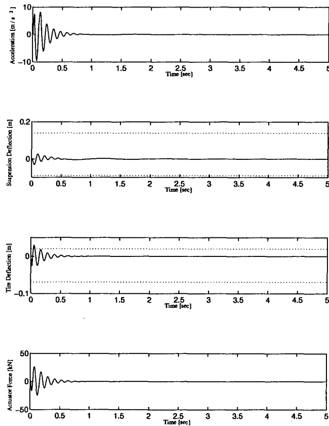
Figure 8.37: Mixed-Design 2 - Medium Configuration - Small Rounded Pulse Input
