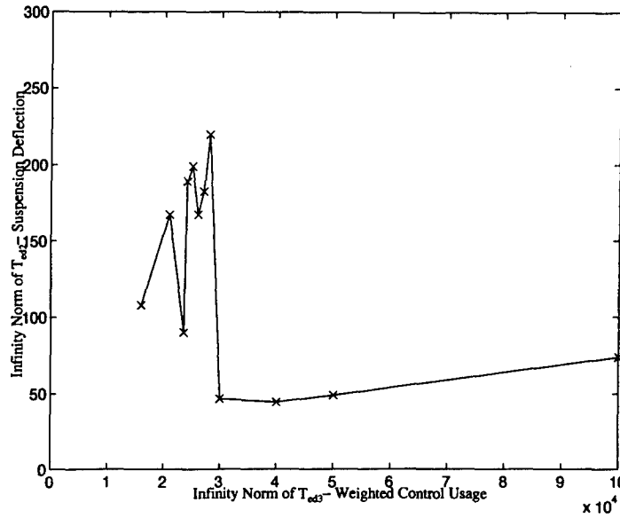
Figure 7.16: \|T_{ed2}\|_{\infty} versus \|T_{ed3}\|_{\infty} , Expanded
