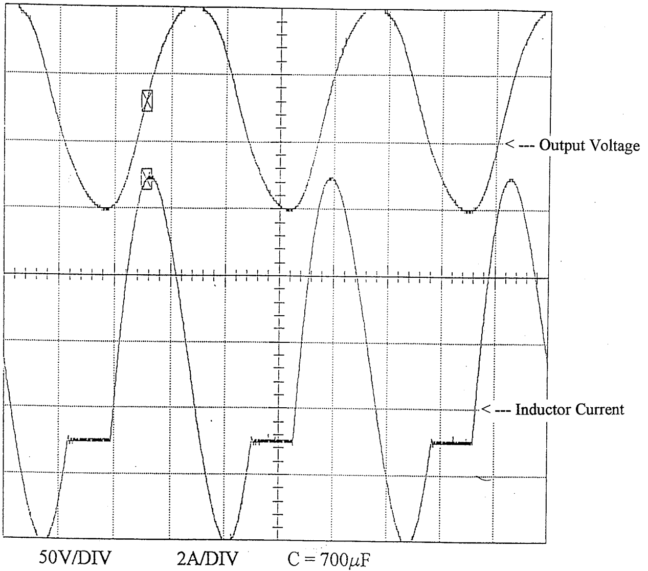
Figure 5.4 Oscilloscope Waveforms of Load Capacitance Variation ( C = 700\mu\text{F} )
