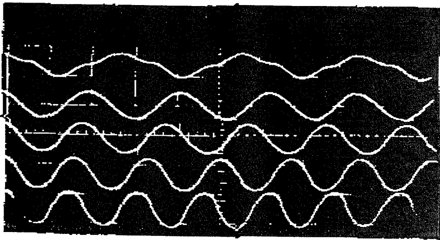
Figure 2.6 Output voltage waveforms for different ratios of resonant to triggering frequency ( f/f_0 ); reading from top: 2, 1.5, 1.35, 1.2, and 1.1. [Ref. 1]
