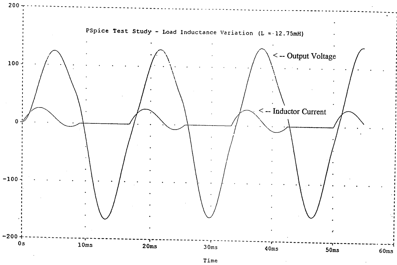
Figure 5.8 PSpice Simulation of Load Inductance Variation (L = 12.75mH)
