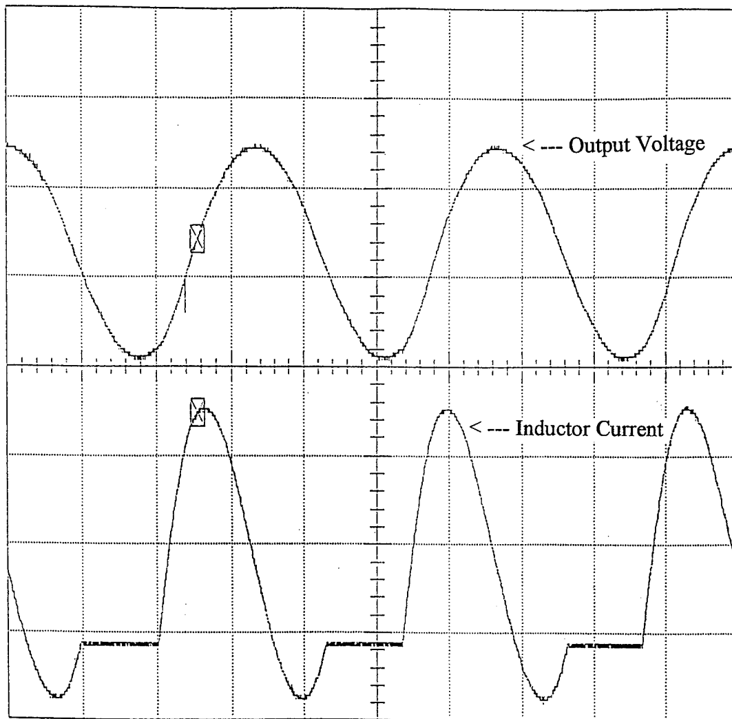
Figure 5.3 Oscilloscope Waveforms of Load Resistance Variation ( R = 23.2\Omega )
