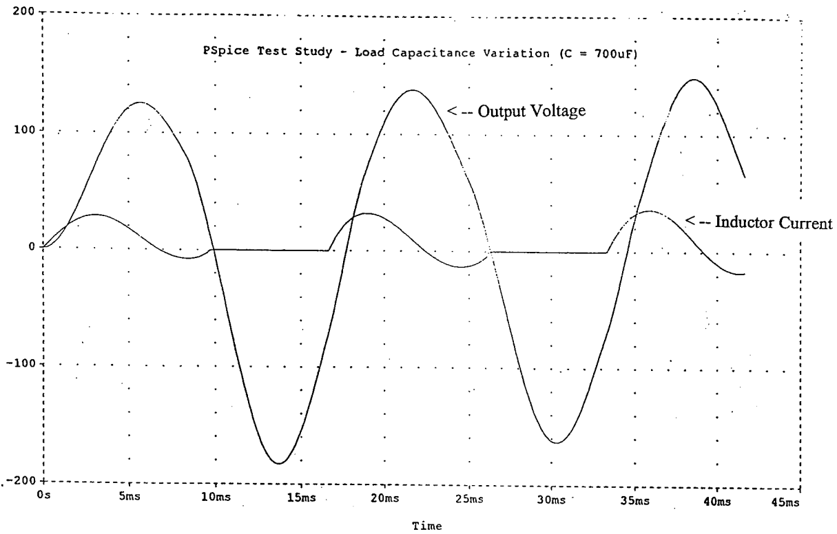
Figure 5.7 PSPICE Simulation of Load Capacitance Variation ( C = 700\mu\text{F} )
