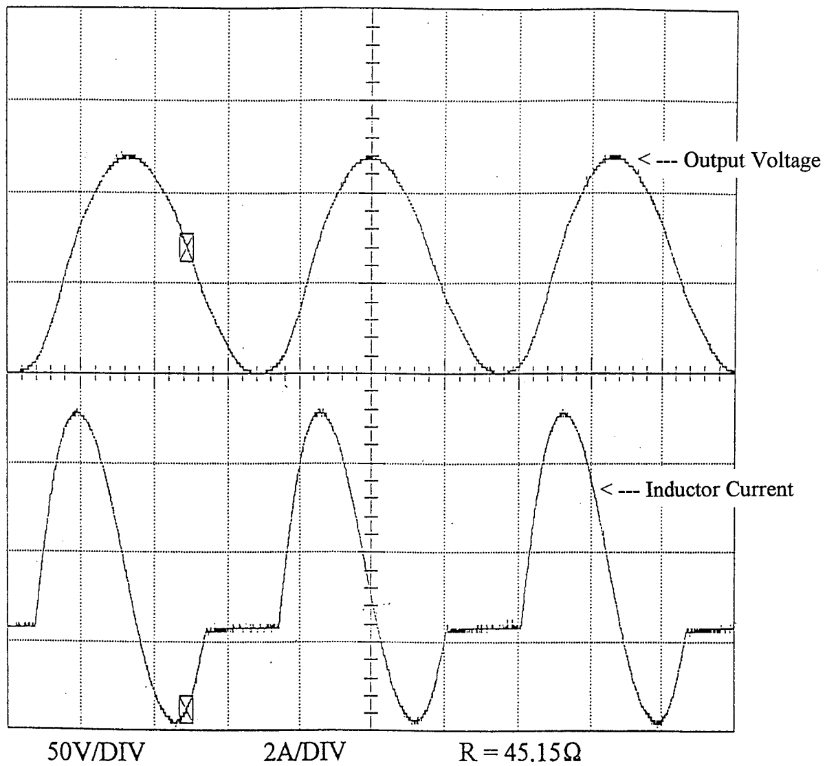
Figure 4.5 Output Waveforms of Center-Tapped Supply in the Laboratory at 60 Hz
