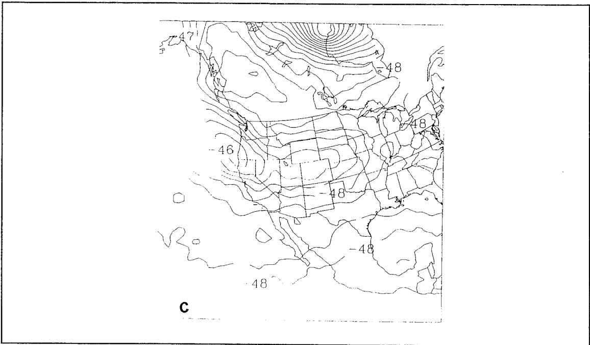
Figure 4.10. Full resolution (110 km) channel 3 MSU brightness temperature (contour interval is 0.5°C) analyses from NOAA-12 and NOAA-14 valid at (a) 0200 UTC 12 May 1995, (b) 1600 UTC 12 May 1995, and (c) 0200 UTC 13 May 1995.
