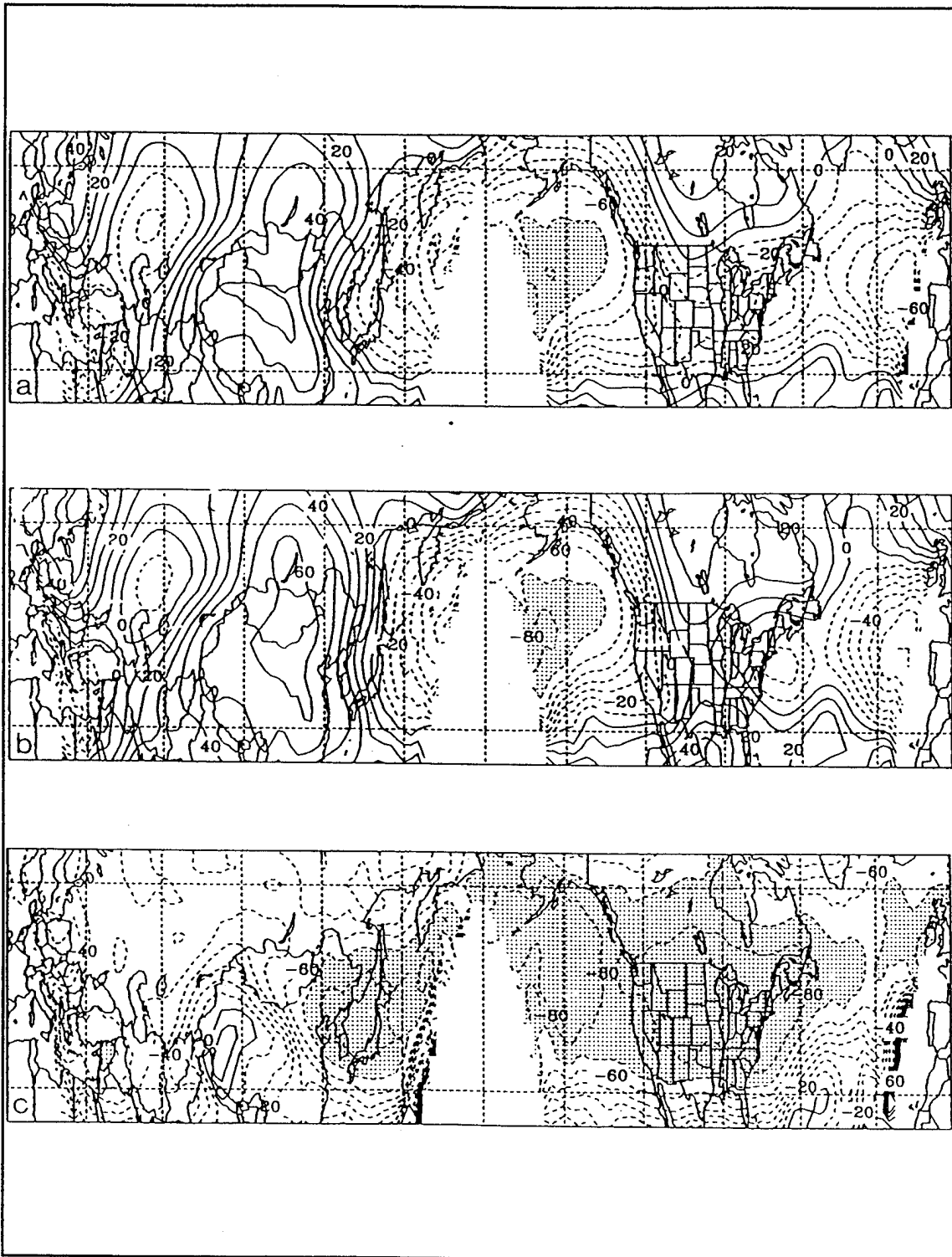
Figure 2.4. Analysis of (a) unfiltered, (b) 14 day low-pass filtered, and (c) \leq 5 day high-pass filtered six-month temporal correlation coefficients (solid, contour interval 10^{-2} ) between the channel 3 MSU and 500-mb heights. Light (dark) stippling represents correlations \geq 0.70 ( \geq 0.90 ). From Parke (1994).
