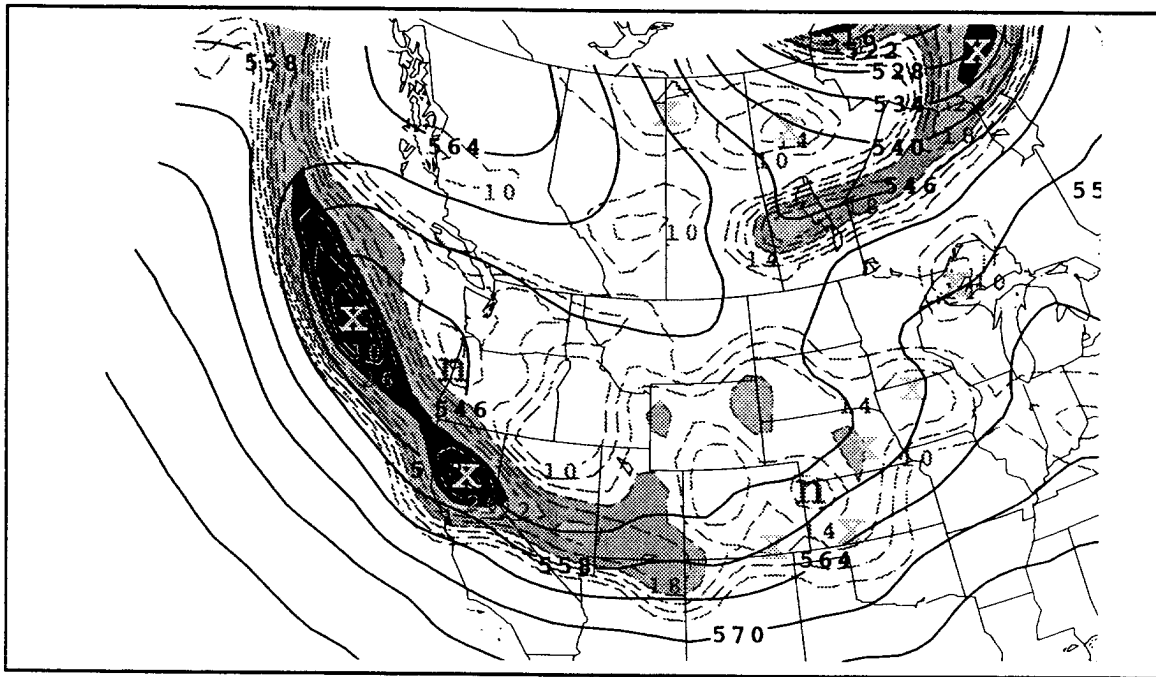
Figure 4.3. Same as Fig. 4.1 except for analysis verifying at 0000 UTC 13 May 1995.
