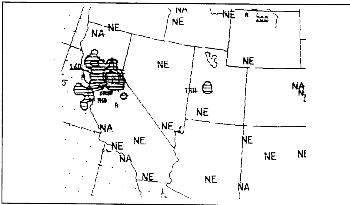
Figure 4.4. NWS national radar summary valid 1735 UTC 12 May 1995.
