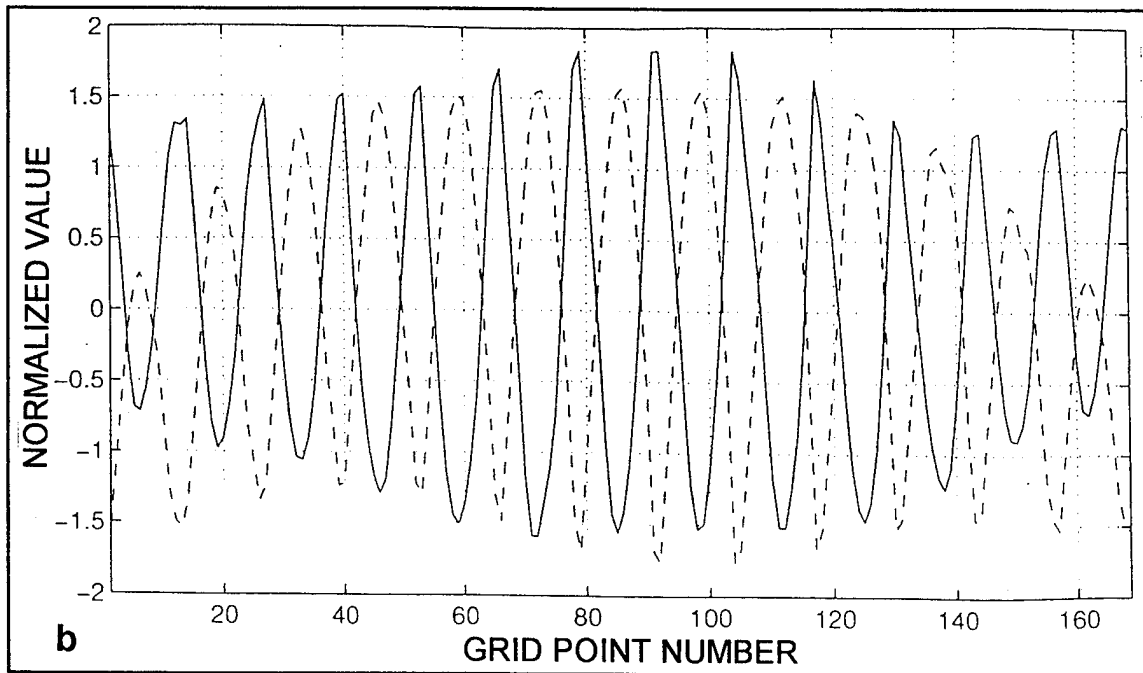
Figure 3.3. Normalized values of channel 3 MSU brightness temperature (solid lines) and 500-mb height (dashed lines) at each individual grid point in sub-domain 6 for the detrended 0000 UTC 22 January 1994 fields. Latitude method is depicted in (a), longitude method in (b).
