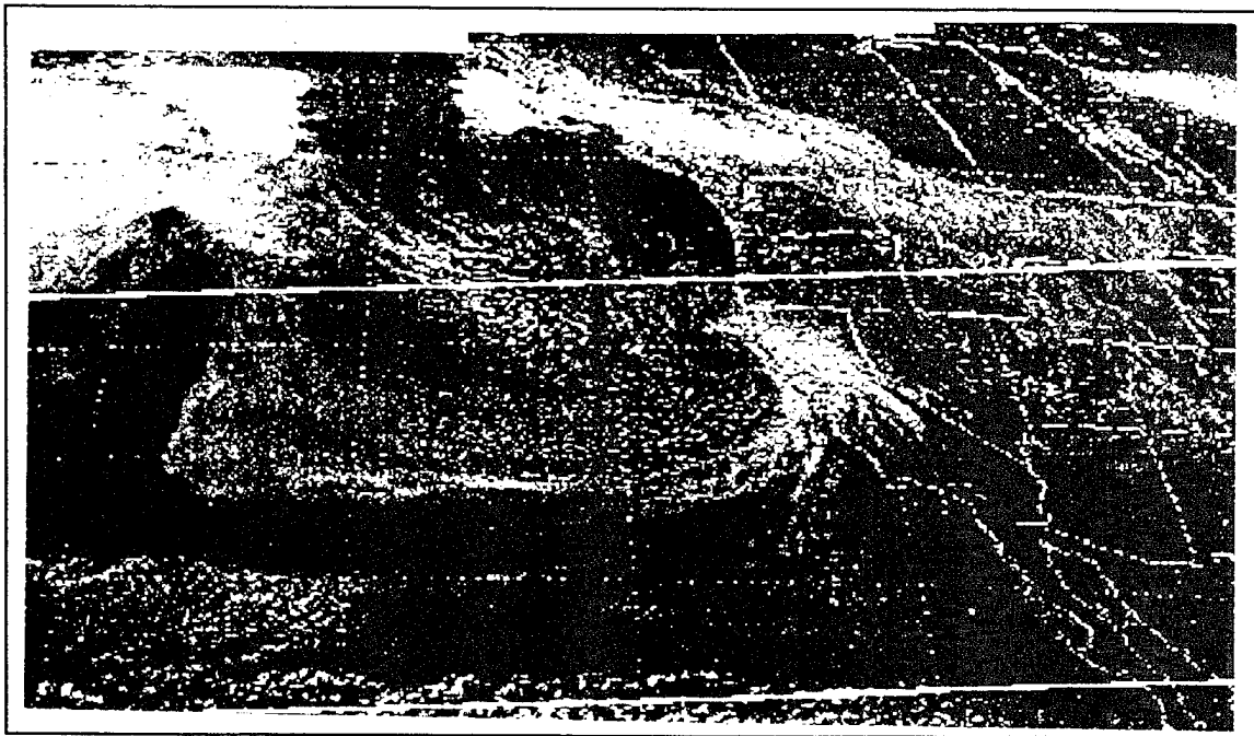
Figure 4.9. 2300 UTC 12 May 1995 visible satellite image.
