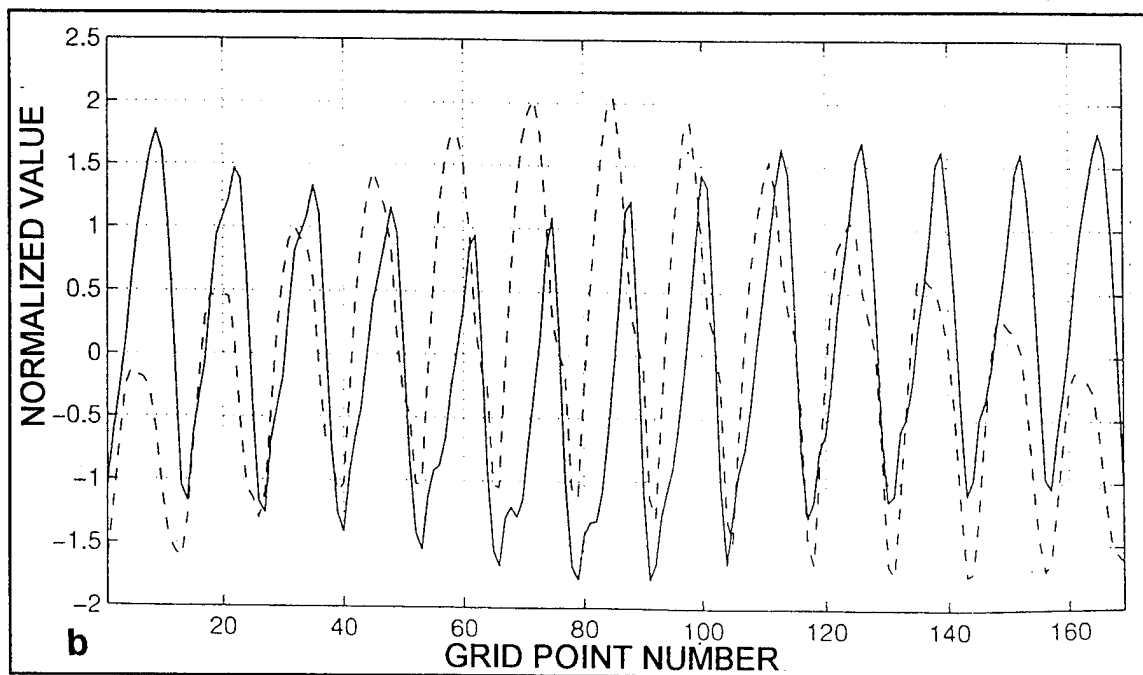
Figure 3.7. Normalized values for channel 3 MSU brightness temperature (solid lines) and 500-mb height (dashed lines) at each individual grid point in sub-domain 6 for the detrended 0000 UTC 16 February 1994 fields. Latitude method is depicted in (a), longitude method in (b).
