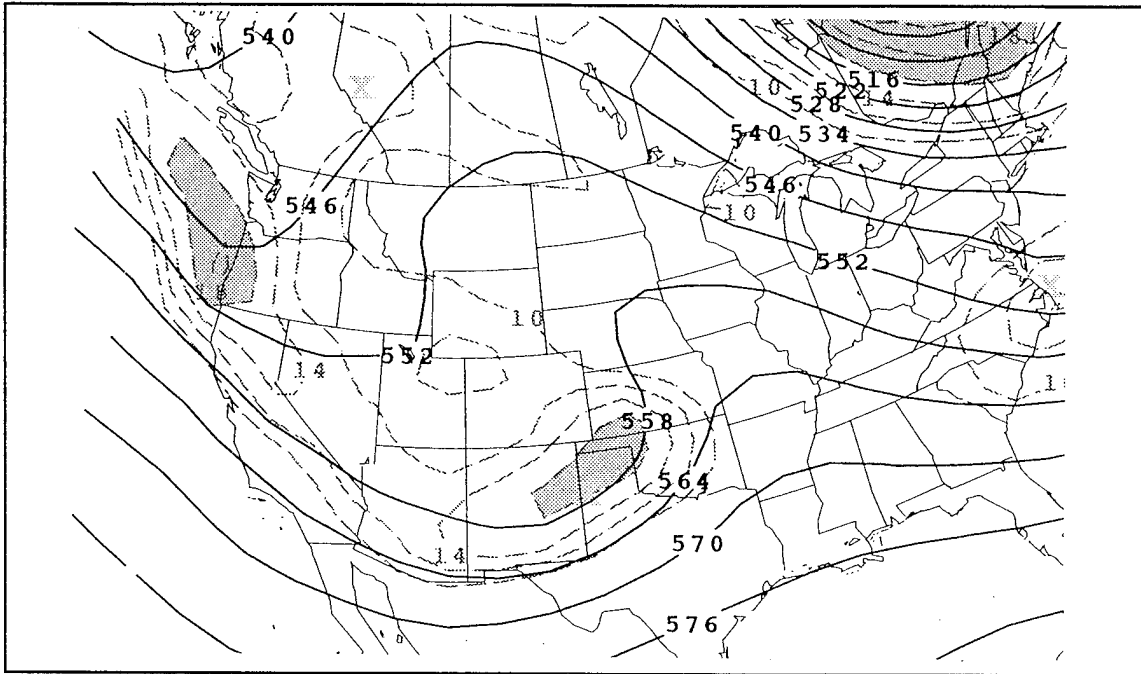
Figure 4.15. Same as Fig. 4.13 except for 24-h forecast verifying at 0000 UTC 27 January 1995.
