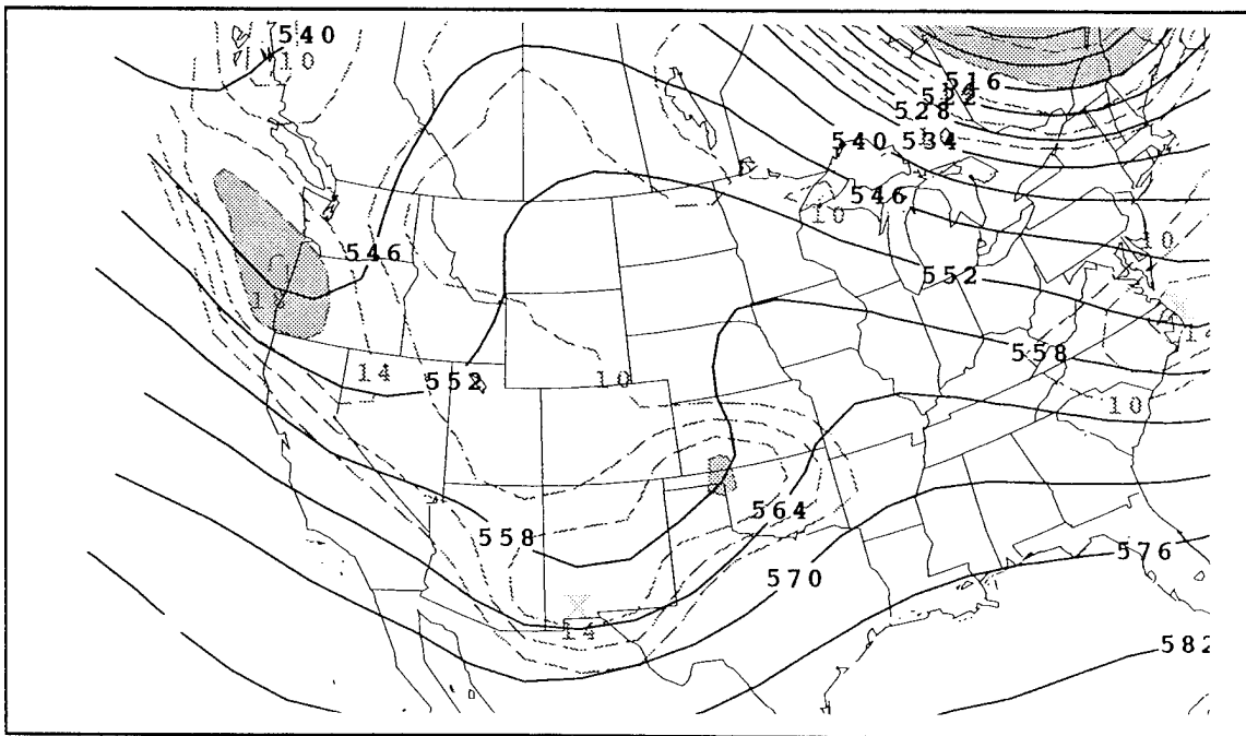
Figure 4.16. Same as Fig. 4.13 except for 12-h forecast verifying at 0000 UTC 27 January 1995.
