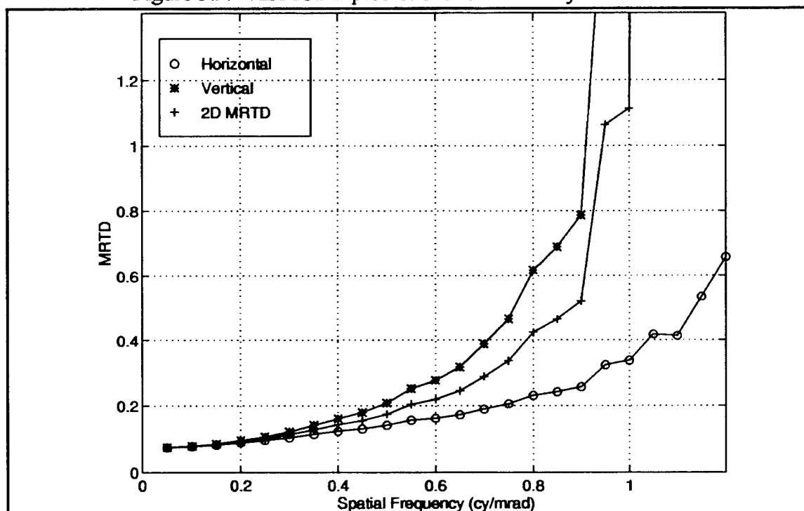
Figure 5.10. VISMODII predictions for Mitsubishi system MRTD
