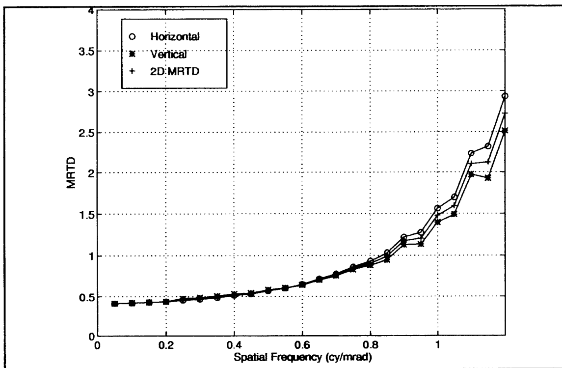
Figure 5.9. VISMODII predictions for Amber system MRTD
