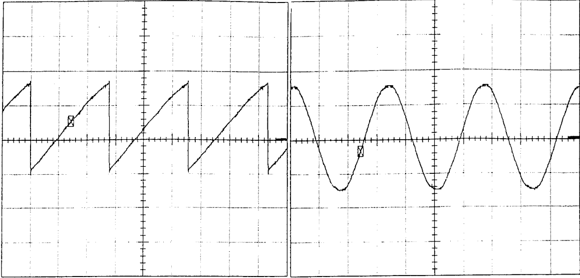
Figure 6.27 Source Phase Voltage, V_s (100V/div) vs. Time (5ms/div); \alpha=159.6^\circ , T_L=4 lbf-in
