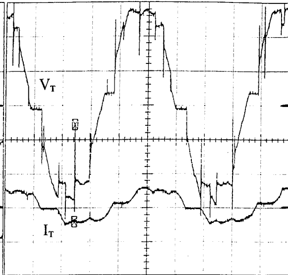
Figure 6.16 Transformer Voltage, V_T (50V/div) and Transformer Current, I_T (1A/div) vs. Time (5ms/div); \alpha=179.3^\circ , T_L=4 lbf-in
