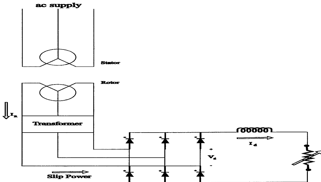
Figure 5.2 Diode Bridge with Variable Load Resistance
