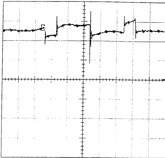
Figure 6.17 Diode Bridge Voltage, V_d (50V/div) vs. Time (1ms/div); \alpha=179.3^\circ , T_L=4 lbf-in
