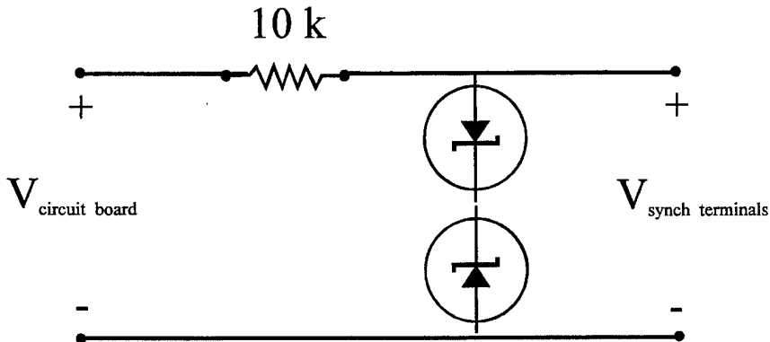
Figure 8.1 dSPACE Protection Circuit
