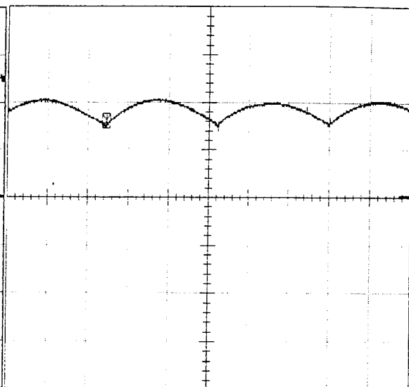
Figure 6.18 DC Link Current, I_d (0.2A/div) vs. Time (1ms/div); \alpha=179.3^\circ , T_L=4 lbf-in
