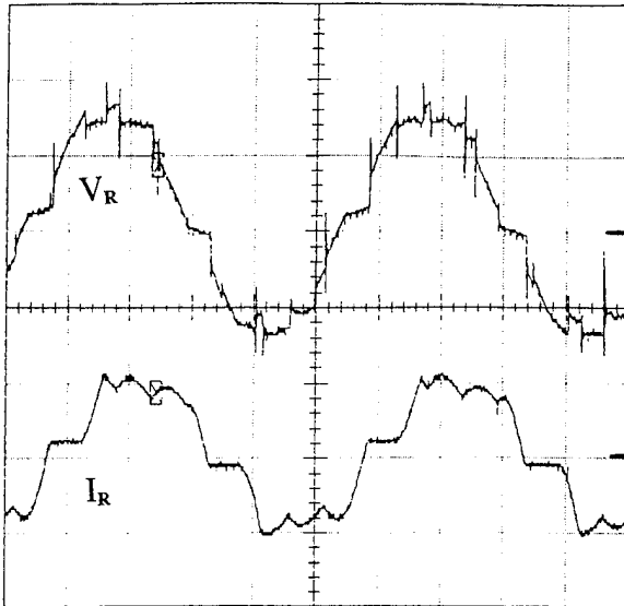
Figure 6.15 Rotor Voltage, V_R (50V/div) and Rotor Current, I_R (1A/div) vs. Time (5ms/div); \alpha=179.3^\circ , T_L=4 lbf-in
