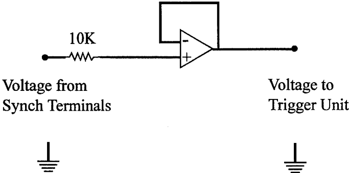
Figure 8.2 dSPACE Protection Circuit
