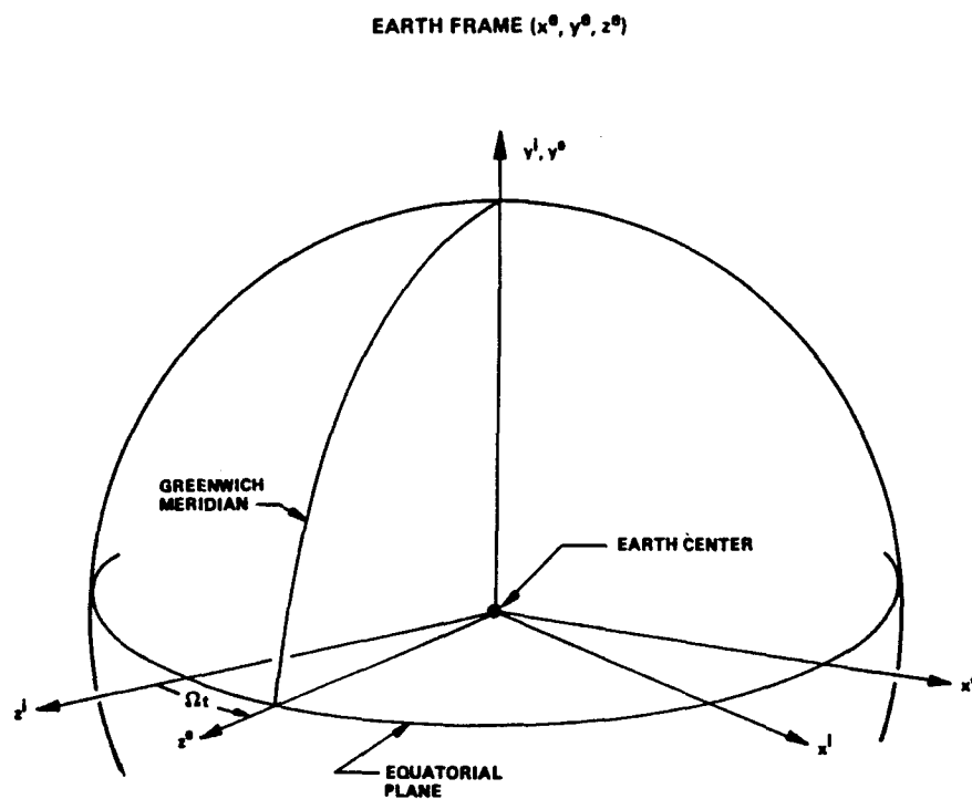
Figure 2 - 4. Earth Frame
