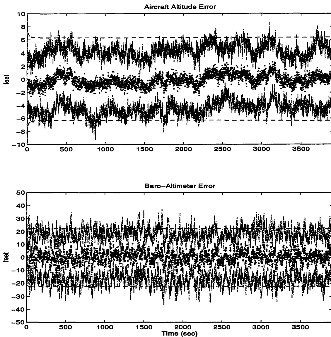
Figure B.14 Aircraft Altitude and Baro-Altimeter Error
