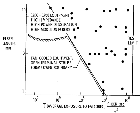
Figure 19. Average exposure to failure for vulnerable equipment.
