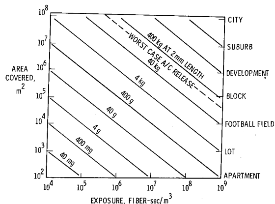
Figure 13. Parametric plot of carbon fiber area coverage.
