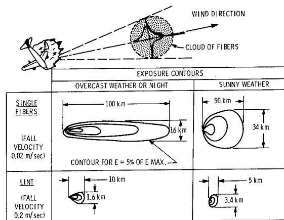
Figure 12. Weather conditions and fiber dispersion.
