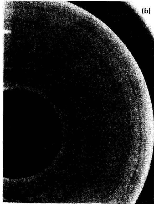
Figure 7. (a) Bidirectionally reinforced woven S2-glass cloth/epoxy laminated disk (AVCO design). (b) Radiograph of AVCO disk showing weave pattern and resin flow direction during molding process.
