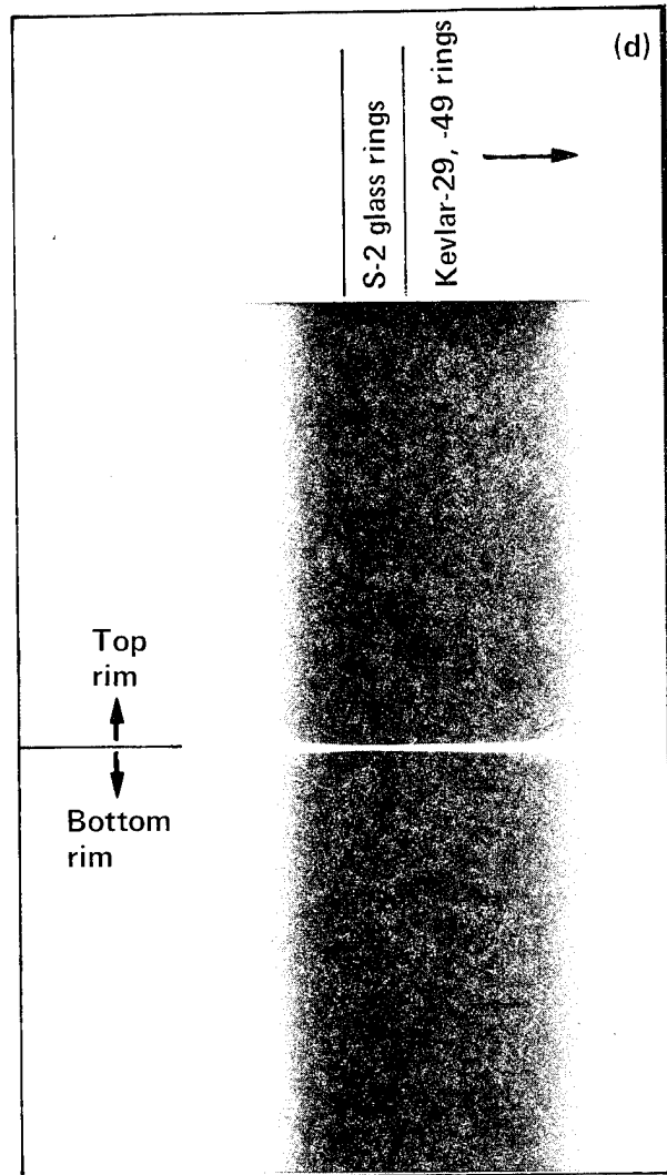
Figure 4. (a) Kevlar-49, Kevlar-29, and S2-glass/epoxy ring rim with graphite/epoxy cruciform hub flywheel (Garrett AiResearch design). (b) Radiograph of Garrett AiResearch flywheel showing density variations between Kevlar-49, Kevlar-29, and S2-glass. Arrow indicates site of separation between rings. (c) Tangential radiograph at site 1 of (b) indicates no separation. (d) Tangential radiograph at site 2 of (b) shows location and depth of separation.
