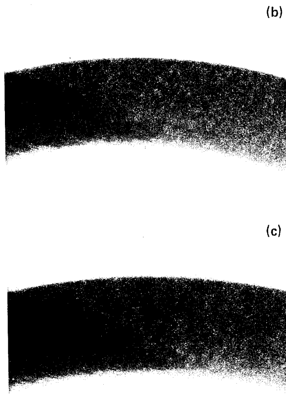
Figure 2. (a) Kevlar-49 S2-glass/epoxy rim with tension-balanced Kevlar-29 spokes (Brobeck design). (b) Radiograph of Brobeck flywheel showing high-density step (arrow) in S2-glass ring. (c) Radiograph of second Brobeck flywheel that did not show high-density step as in (b). Variation between flywheels is likely to be result of manufacturing-process control.
