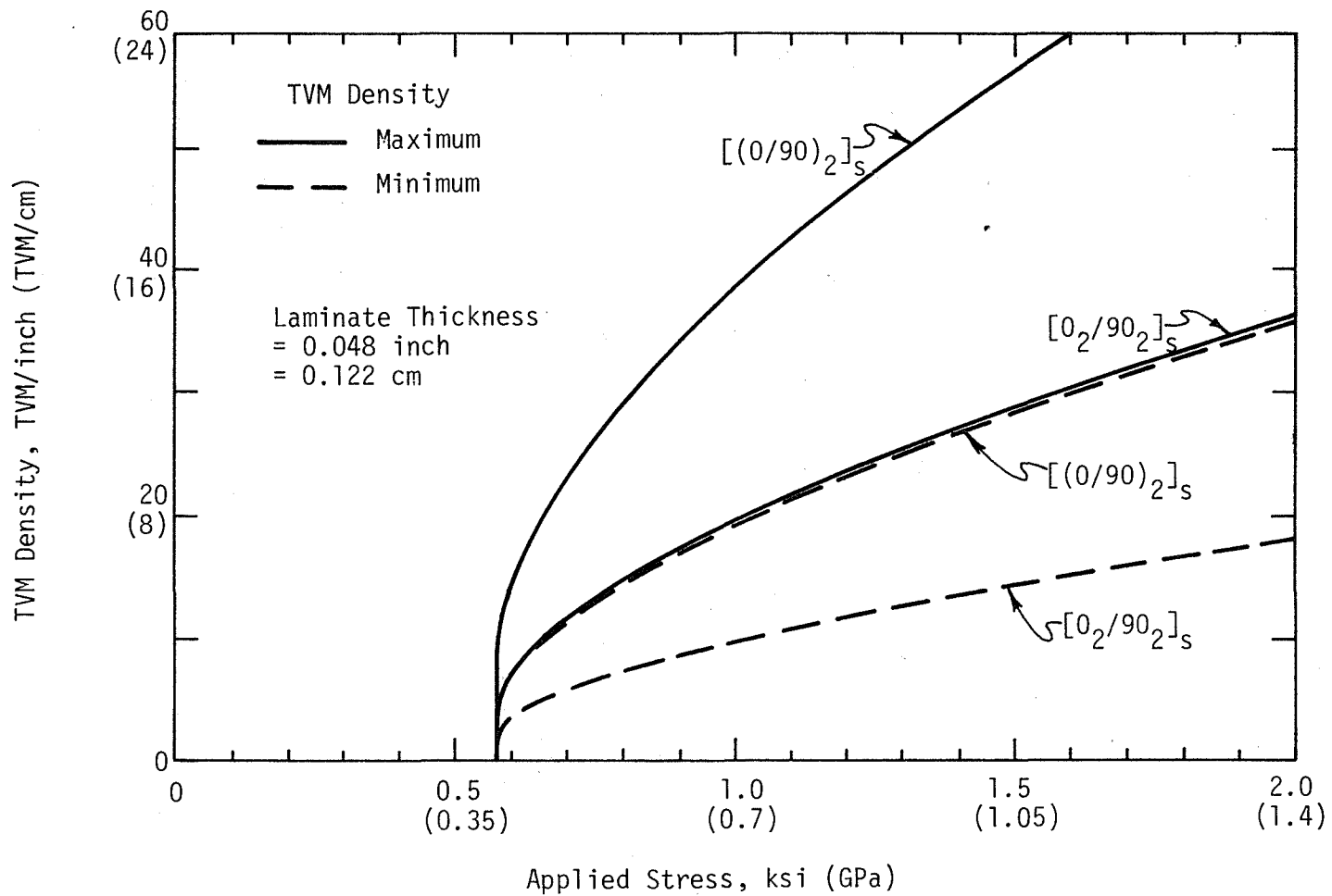
Fig. 44. Effect of Stacking Sequence on TVM Density in Cross-Plied Laminates.
