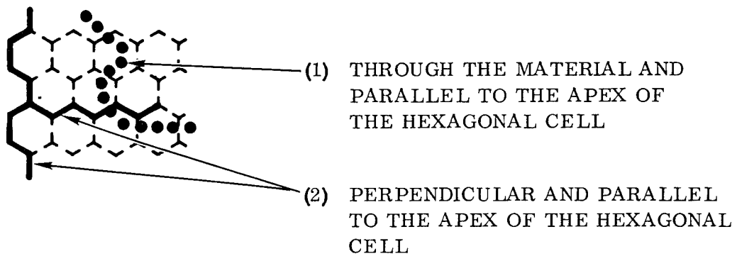
Figure 3. Failure Modes in Plate Thermal Cycle Tests
