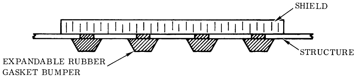
Figure 38. Illustration of "Expandable Bumper Gasket" Fastening
