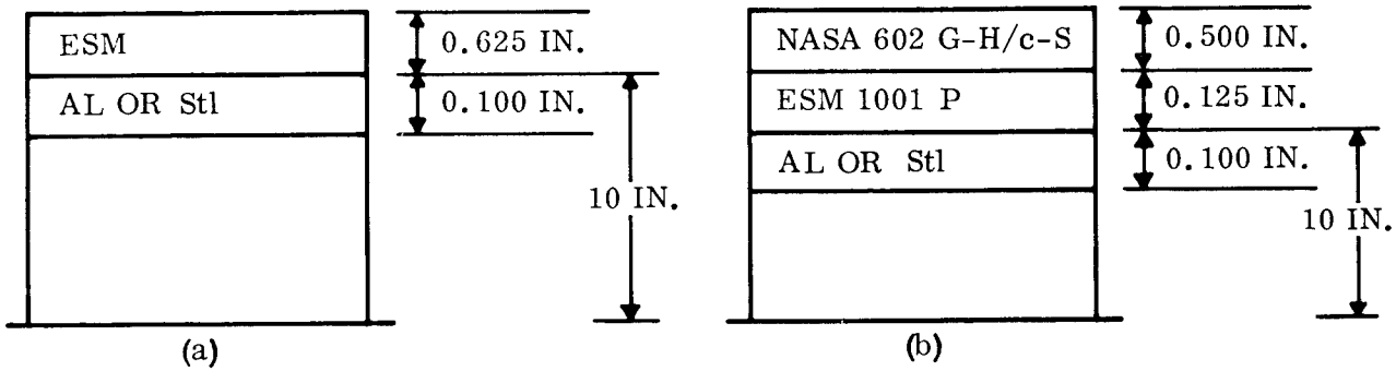
Figure 23. Structural Analysis Configuration
