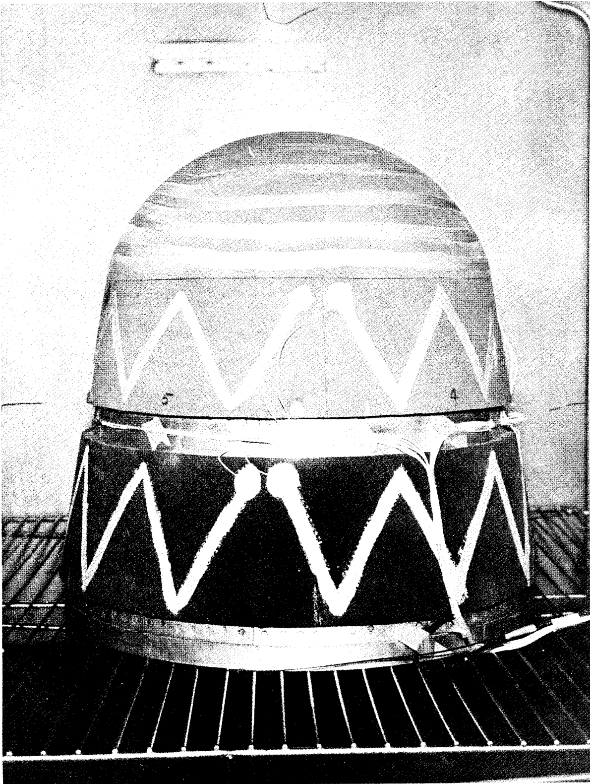
Figure 28. Instrumented Thermal Cycle Unit
