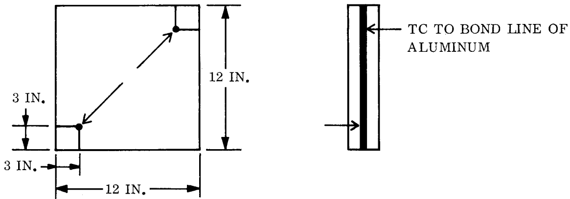
Figure 2. Thermocouple Placement - Plate Thermal Cycle Test Sample
