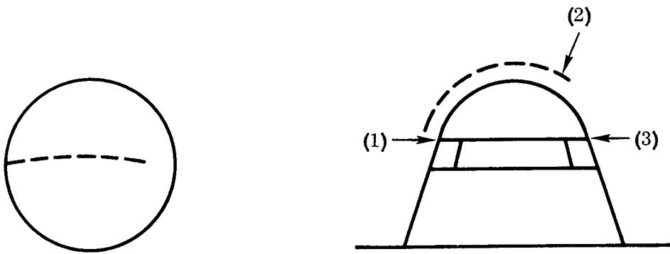
Figure 30. Location of Cracks in Thermal Cycle Unit
