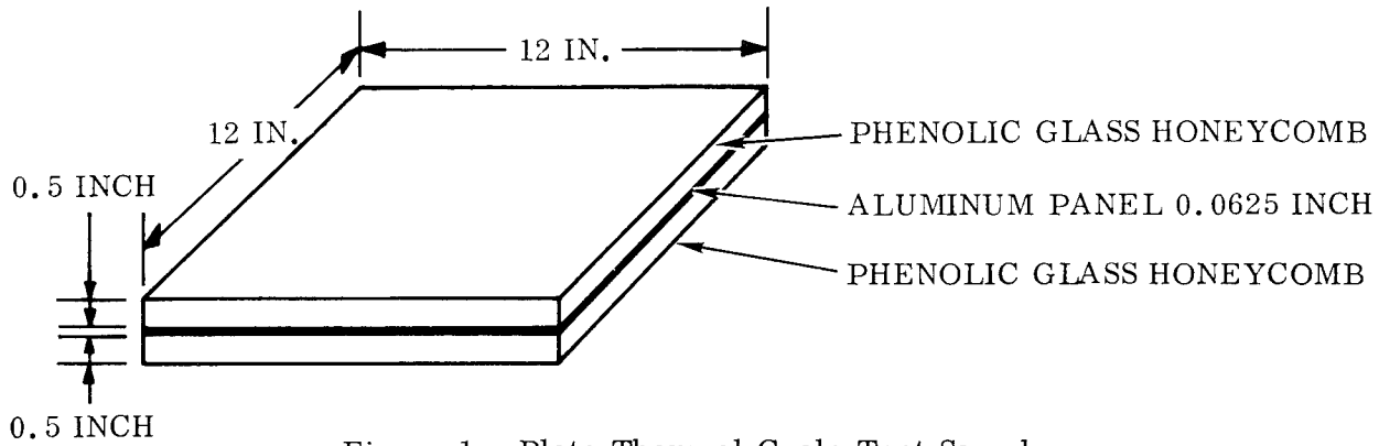
Figure 1. Plate Thermal Cycle Test Sample
