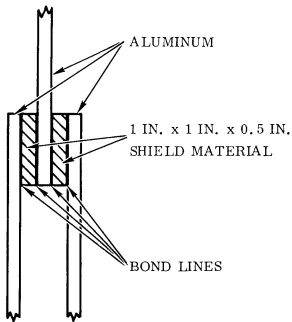
Figure 39. Bond-Shear Test Sample Configuration
