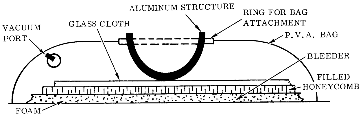
Figure 26. Scale-Up Fabrication of NASA 602 G-H/c-S - ESM 1001 P Composite
