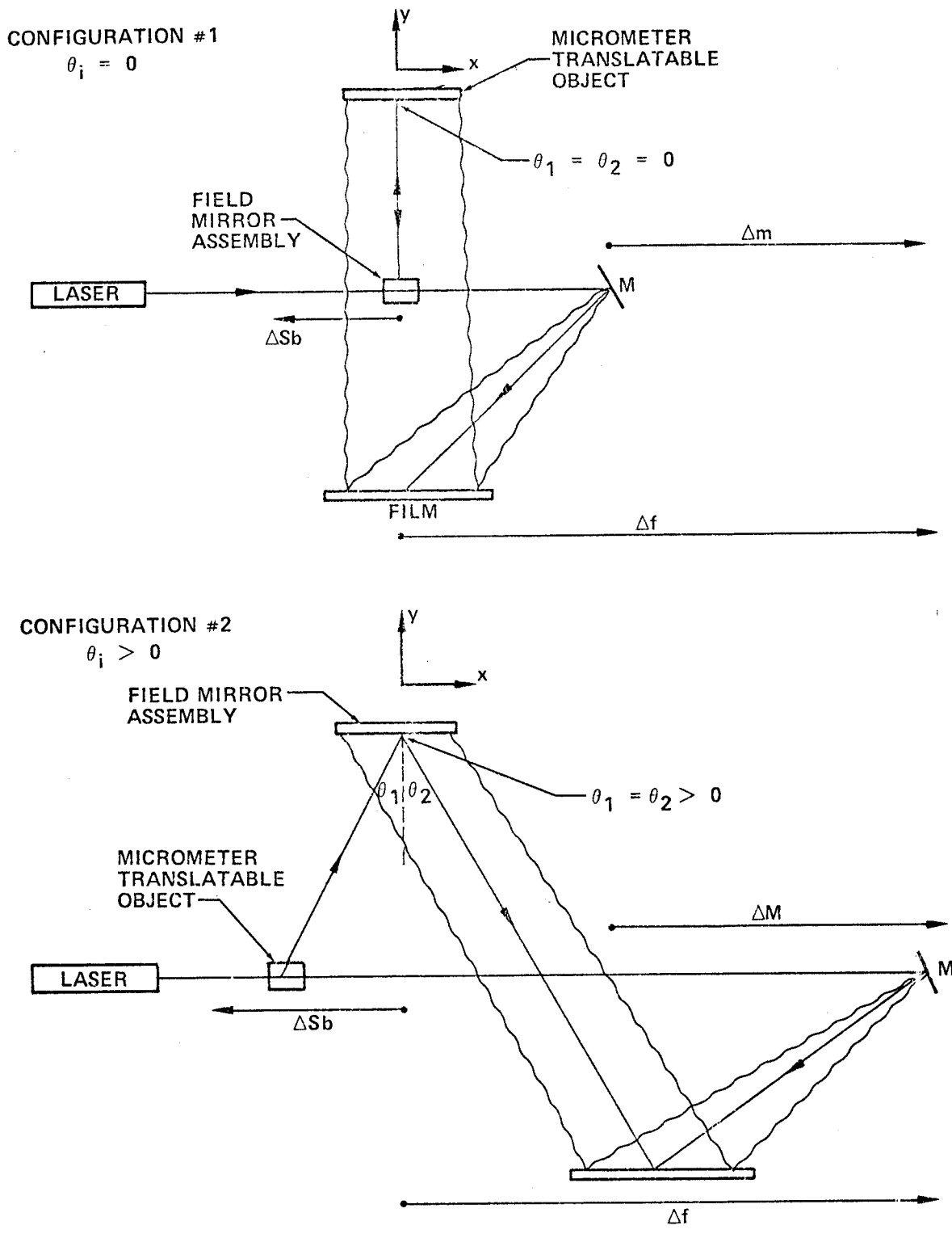
Figure 1. Composite Mobile Holographic Nondestructive Test System.
