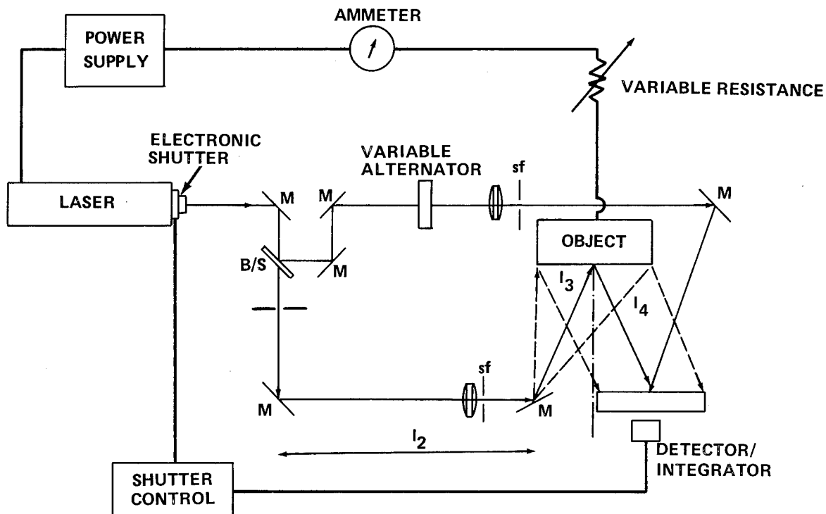
Figure 2. HNDR system diagram.
