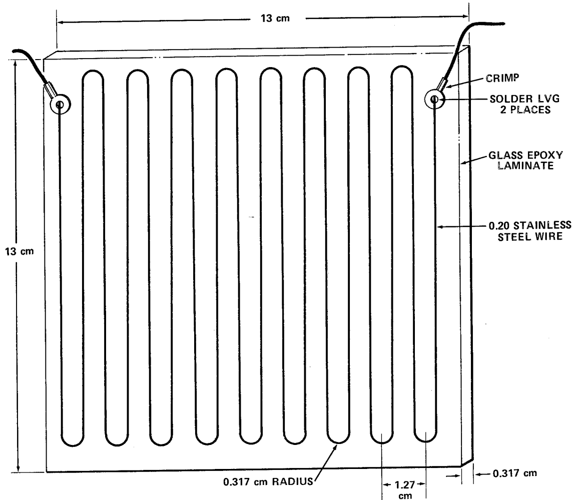
Figure 6. Design diagram of a glass laminate heater.
