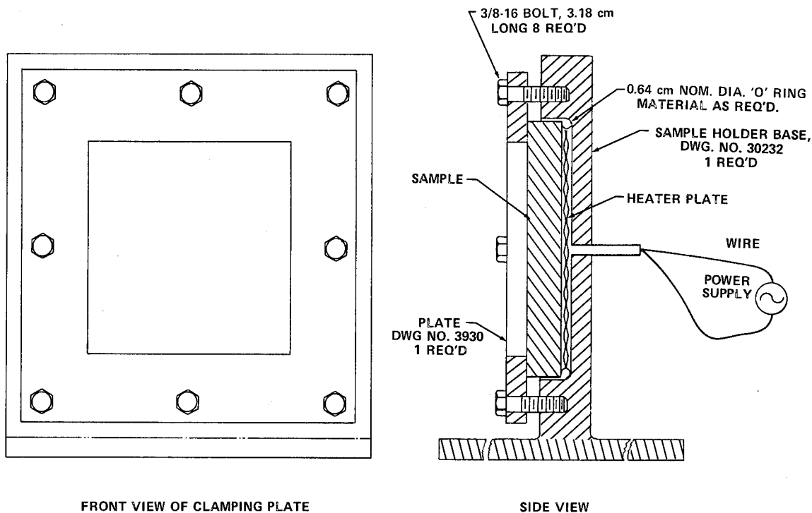
Figure 5. Design diagram of sample holder assembly and the heater plate connection in the thermal loading system.
