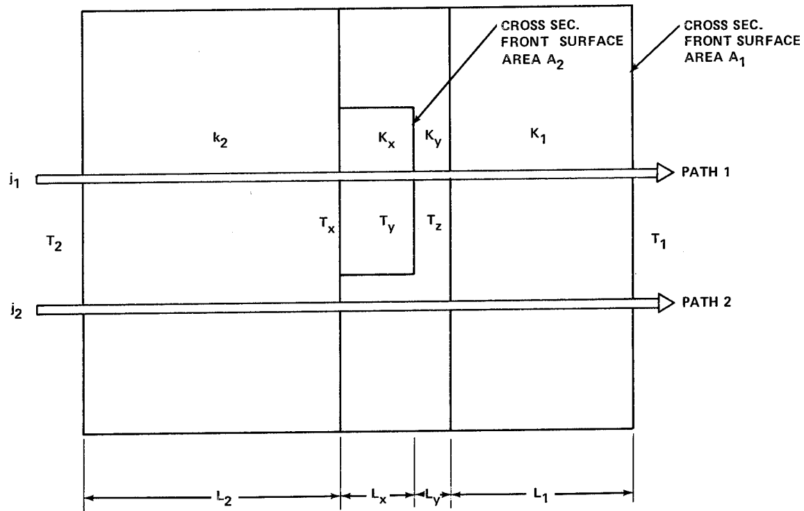
Figure 8. Cross section of the test plate.
