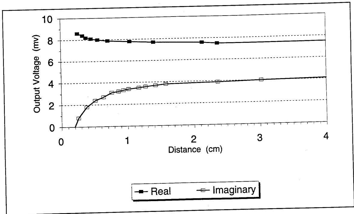
Figure 17. Voltmeter recordings versus distance from bottom
