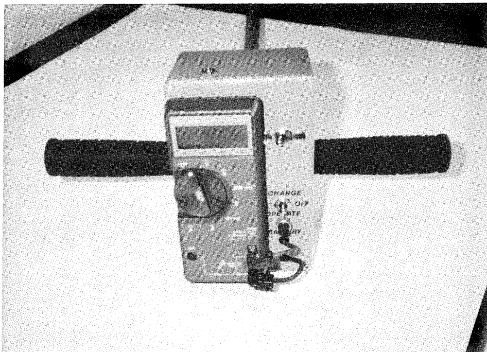
Figure 12. DCSR reflectometer box
