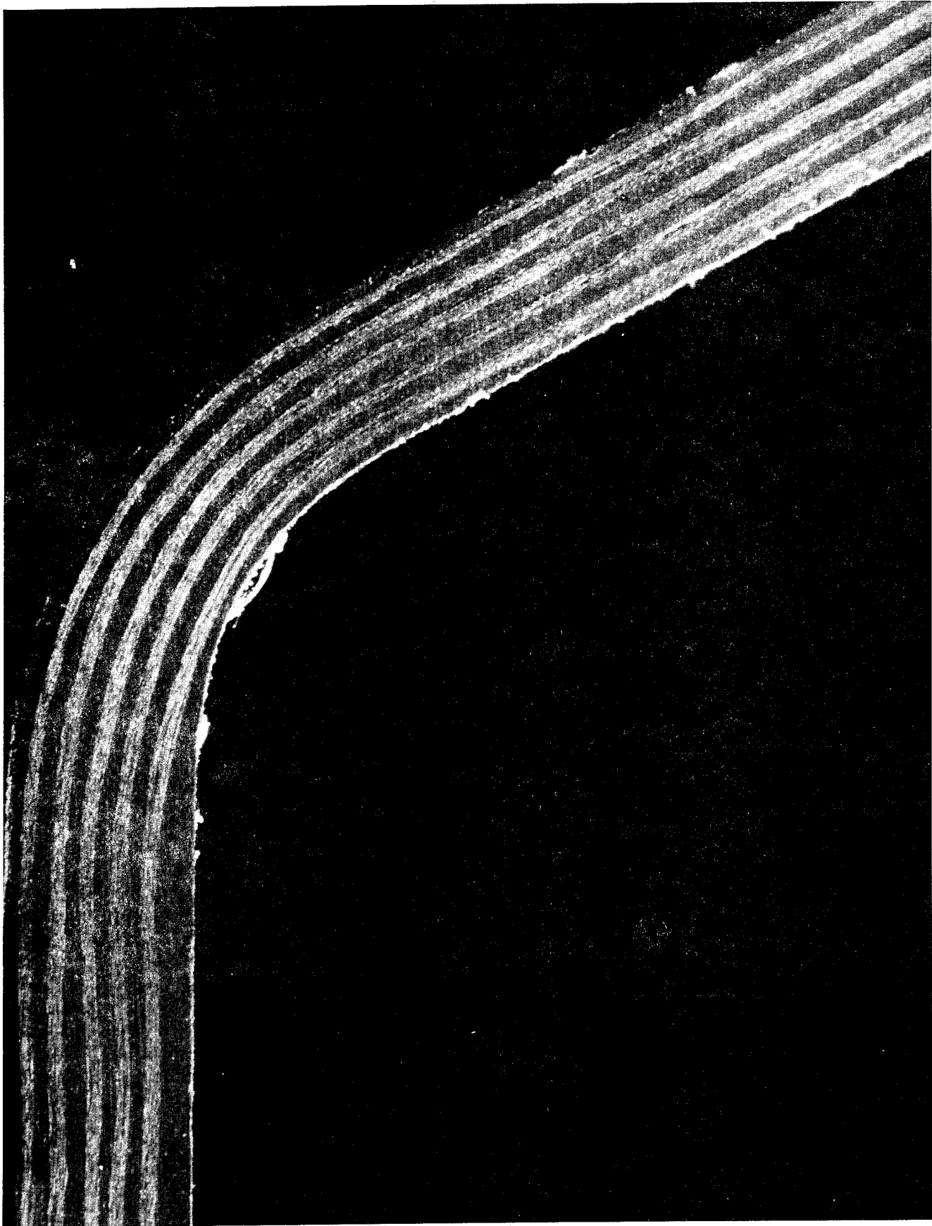
FIGURE 51 ENLARGEMENT OF CORNER RADII OF A 3004-AS POST-FORMED CORRUGATED PANEL
