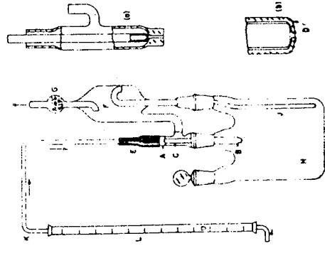
FIG. 1 Ozone Absorbing Device (Syringe Jet).
