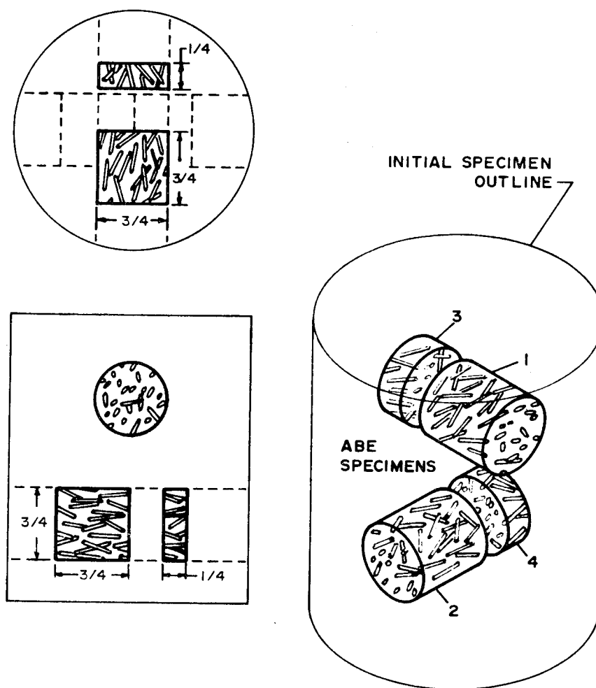
Figure 30. Anisotropic Specimens.
