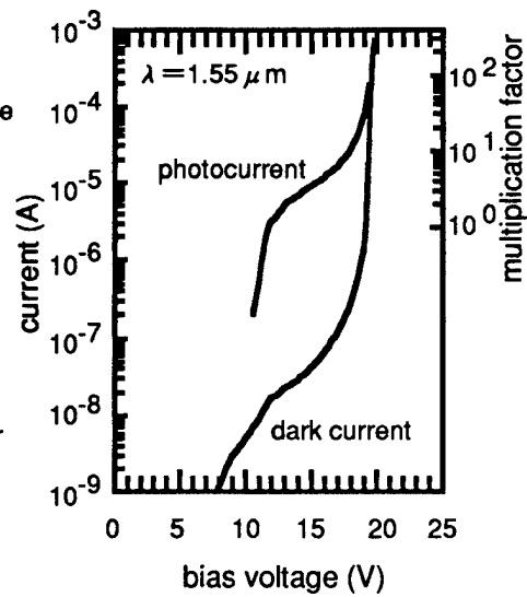
Fig. 2 Dark current, photocurrent, and multiplication factor of a WG-SL-APD at a wavelength of 1.55 \mu\text{m} .
