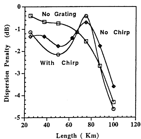
Fig. 4 Shows the calculated results of external modulated
