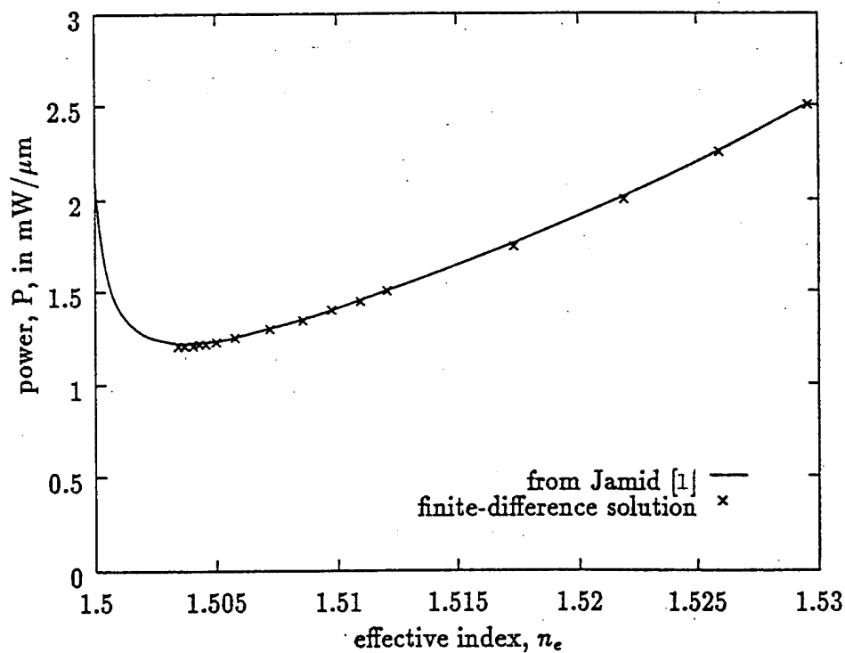
Fig. 2. Dispersion Graph for Self-guiding Nonlinear Waveguide
