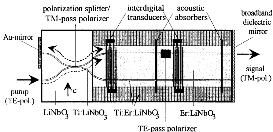
Fig. 1: Schematic diagram of the Er-diffusion doped acoustically tunable \text{Ti:LiNbO}_3 -waveguide laser; c: optical axis of \text{LiNbO}_3 . The total length of the laser is 54.7 mm.
