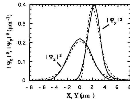
Fig.6 Normalized (unit power) width and depth intensity profiles for W=6\mu\text{m} ; measured (solid) and computed (dashed).
