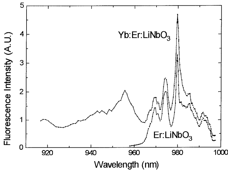
Fig. 2. Excitation spectra of the 1531nm fluorescence pumped at the 980nm transition band of Er single-doped and Yb:Er co-doped \text{LiNbO}_3 crystals at \sigma -polarization.
