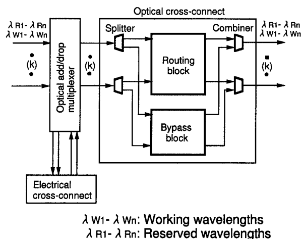
Fig. 3 Cross-connect architecture for failure recovery
