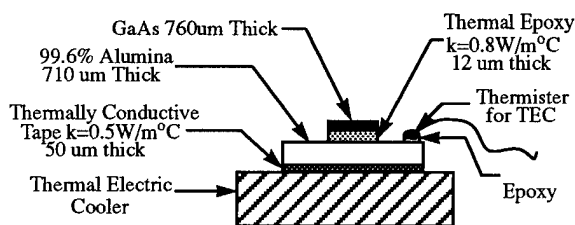
Figure 3 Thermal Model for FEA
