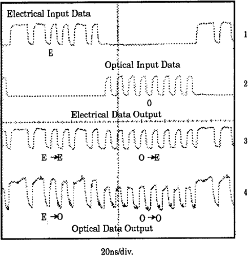
Fig. 3. Experimental demonstration of the switching and multiplexing of input electrical and optical data packets, and their conversion into a single optical or electrical output data stream at 200 Mb/s.
