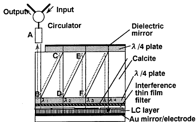
(a) Reflection-type multi-channel selection filter.
