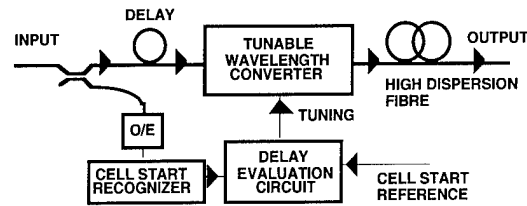
Fig. 4: Schematic of the fine synchronizer.
