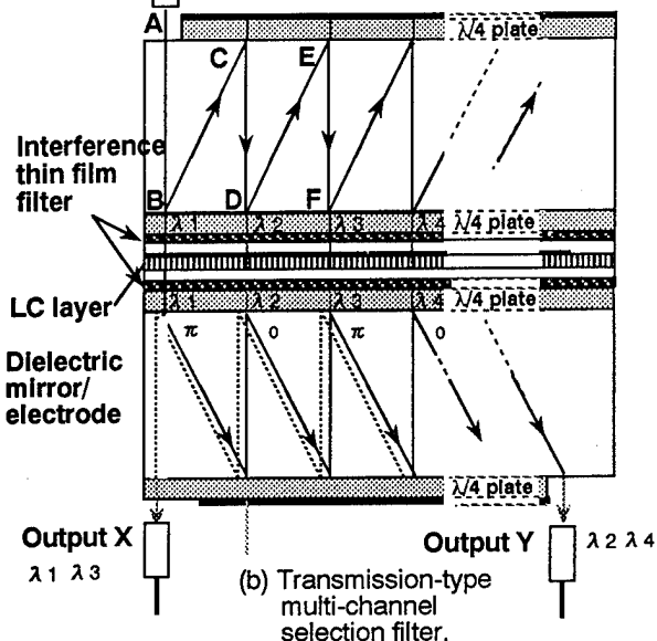
(b) Transmission-type multi-channel selection filter.
