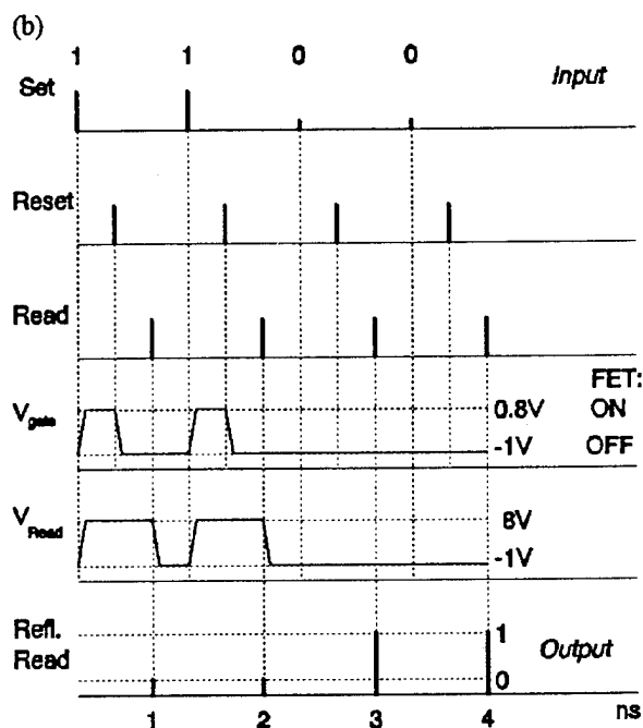
Fig.1. (a) POET circuit schematic. (b) Input and output pulse sequence.
