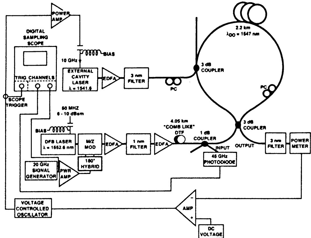
Figure 1. Experimental set-up.
