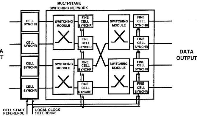
Fig. 2: Large size switching node with a multi-stage structure.
