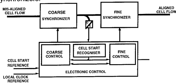
Fig. 3: Schematic of the optical synchronizer.
