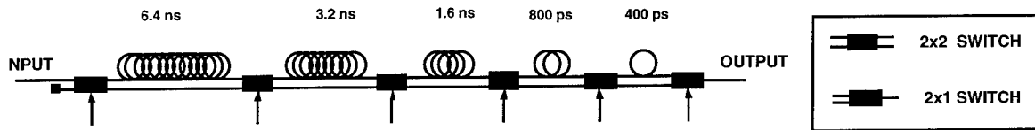
Fig. 5: Schematic of the coarse synchronizer.
