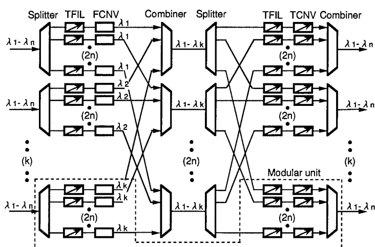
(b) Link modular expandable switch structure
