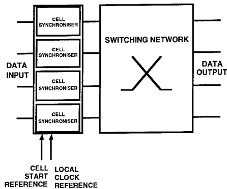
Fig. 1: Optical packet switched node with synchronizers.
