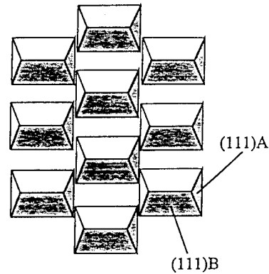
Fig.2: Formation of 2DVGs by the growth of dot structures which have (111)A and (111)B-facets on pattern substrates. A 2DVG is formed among for dot structures.
