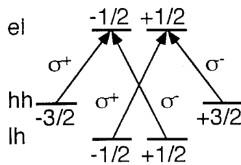
Fig. 1: Level scheme with transition rules.
