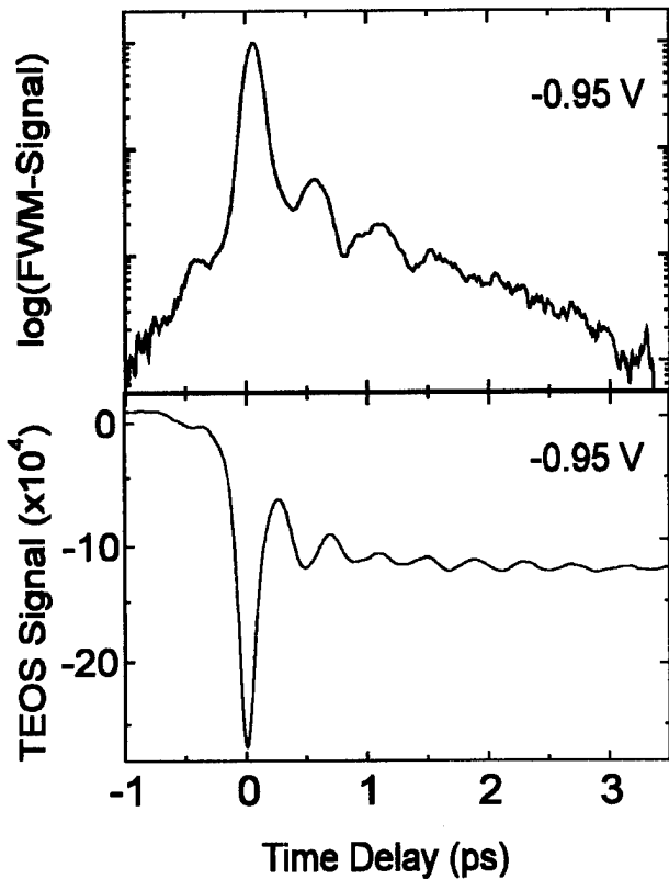
Fig.1: Simultaneously recorded TEOS (linear plot) and FWM (logarithmic plot) signals at an applied voltage of -0.95 V.
