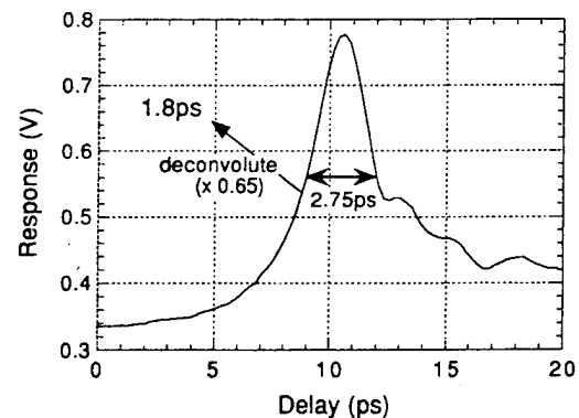
Fig. 3 Pulse shape of photogenerated pulse. Actual pulse width and PCSS response should be shorter than 1.8ps.
