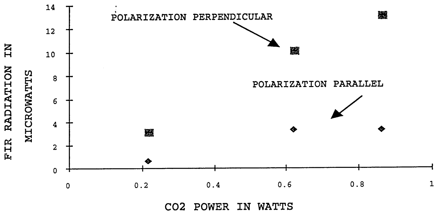
Figure 3. FIR Radiation Output .US. A Co2 Laser
