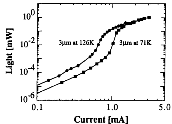
Fig 3. Light versus current for 3 \mu\text{m} diameter devices at heat-sink temperatures of 126 K (optimal detuning) and 77 K.
