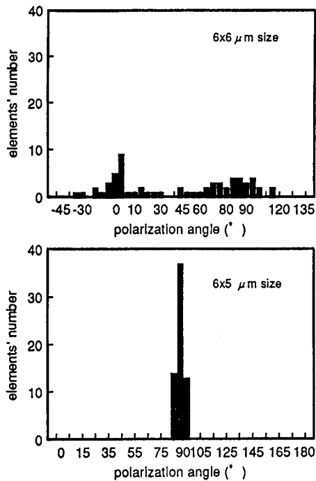
Fig.3: Polarization angle distribution of (a) the 6x6 μm size polarization uncontrolled VCSEL and (b) the 6x5 μm polarization controlled array. The deviation angle is only 2.9° for the 6x5 μm array.
