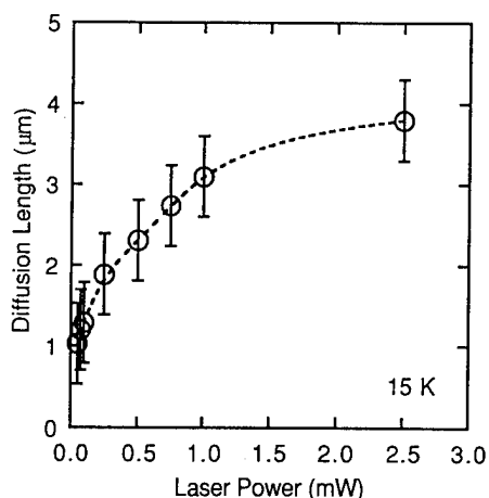
Fig. 3. Diffusion length of excitons in the 15-nm wire structure as a function of excitation laser power.
