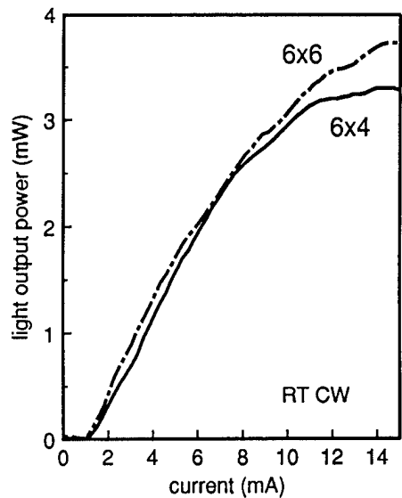
Fig.4: L-I characteristics of the 6x4 μm polarization controlled VCSEL and the 6x6 μm polarization uncontrolled VCSEL. The difference in the higher current range is probably caused by heating, and be reduced when a heat sink is used.
