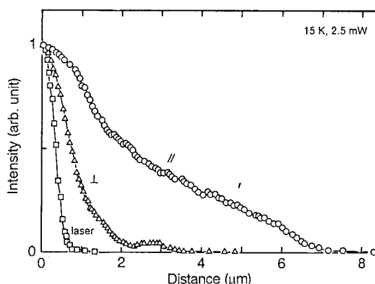
Fig. 2. Intensity profiles of the photoluminescence parallel and perpendicular to the 15-nm wire structure, where laser beam profile is also plotted for comparison.
