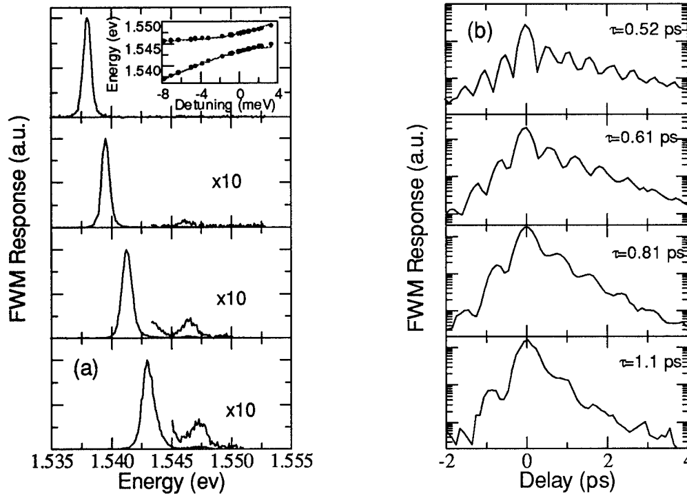
Fig. 2 (a) FWM spectra at zero delay with various exciton-cavity detunings. The inset shows the position of the normal modes in reflectivity spectra as a function of the detuning. (b) FWM signal as a function of the delay between the two incident pulses. The data are obtained at the peak of the corresponding cavity-like resonance in Fig. 2a. \tau is the period of the oscillation.
