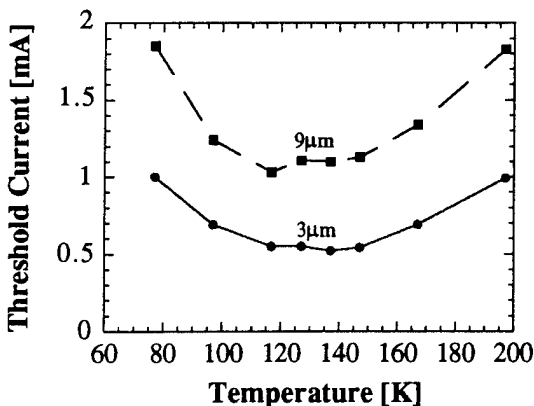
Fig 2. Threshold current versus heat-sink temperature for 3 \mu\text{m} and 9 \mu\text{m} post diameter structures.
