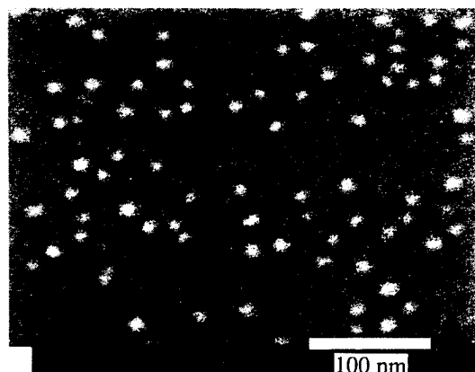
Fig.1: InGaAs quantum dots formed by MOCVD using Stranski-Krastanow mode
