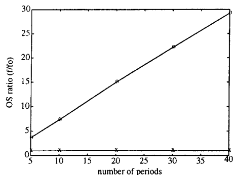
Figure 4: Oscillator strength ratio ( f/f_0 ) vs. number of periods for a barrier width of 50 Å. f denotes the case where the Coulomb attraction is considered and f_0 the case where the Coulomb attraction is neglected. (a) no external bias (b) external bias applied.
