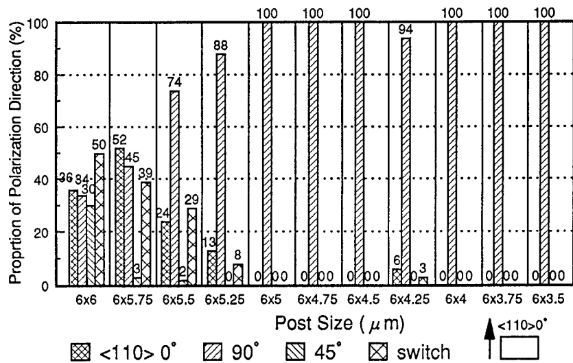
Fig.2: Proportion of polarization direction of 8x8 matrix array (64 VCSELs) vs. post size from 6x6 μm to 6x3.5 μm. Polarization was completely controlled for 6x5 μm - 6x3.5 μm sizes. Probably, the post structure was broken for 6 % of the 6x4.25 μm size array, which does not have 100 % polarization pinning.
