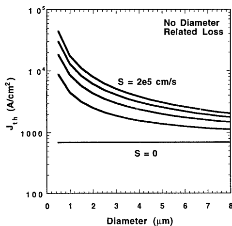
Figure 3: Modelled threshold currents with no size limiting optical loss.
