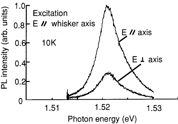
Fig. 5 Polarization dependence of the GaAs whisker photoluminescence under excitation whose polarization is parallel to the whisker axis. The measurement temperature is 10 K.
