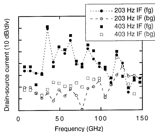
Figure 3. Relative foreground (fg) and background (bg) source-drain current response of coupled quantum dot sample to picosecond pulses at different offset (intermediate) frequencies (IF) and 512 averages. Dotted lines are guides to the eye.
