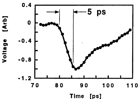
Figure 6. Probing of nonlinear transmission line.
