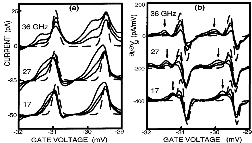
Fig. 3. (a) Current I versus gate voltage V_g on gate 1 at three different frequencies. Dashed curve is without microwaves and solid curves are for increasing power. (b) Derivatives \partial I / \partial V_g of the curves shown in (a). Arrows indicate the photon-induced maxima. Different data sets are offset for clarity.
