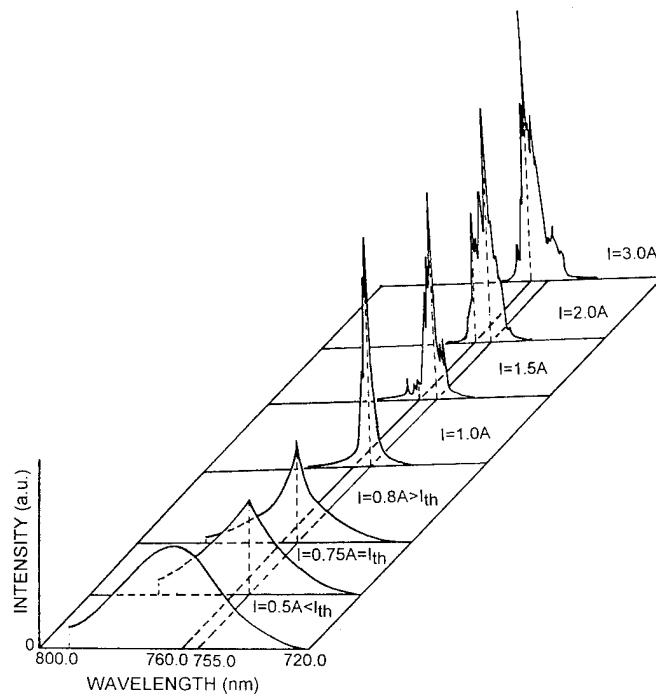
Fig. 3. Room temperature lasing spectra.
