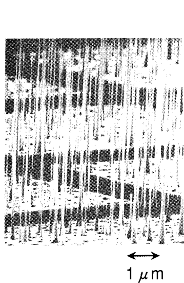
Fig. 1 Typical GaAs whiskers whose growth positions are randomly distributed on the substrate.
