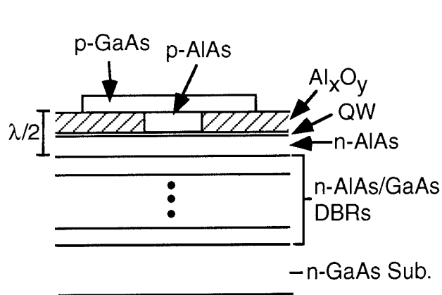
Figure 1: Schematic cross-section of half-wave VCSEL.
