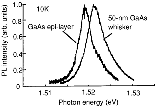
Fig. 4 Photoluminescence spectra for 50-nm GaAs whiskers at 10 K. The result from an undoped MOVPE GaAs epi-layer is also shown as a reference.
