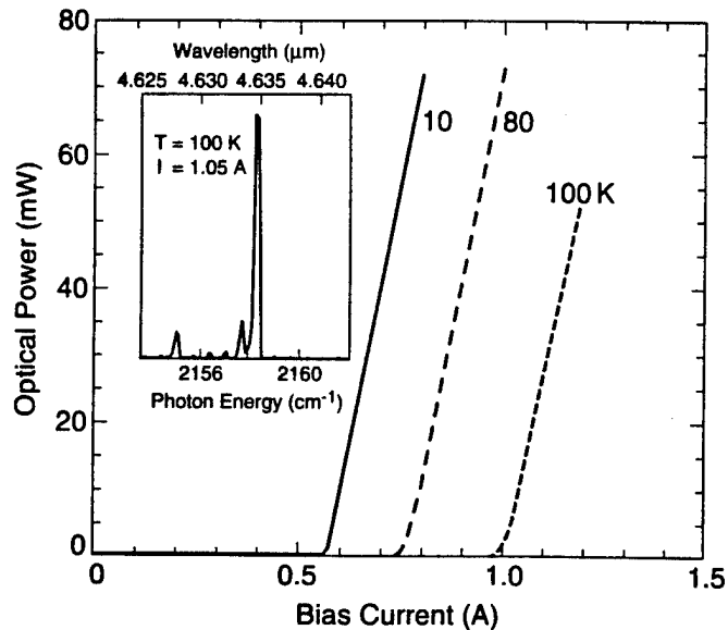
Figure 4. Peak optical output power from a single facet vs. drive current at various heat sink temperatures for the quantum cascade laser with vertical transition. The device is 2.4 \text{ mm} long. Inset: high-resolution spectra of the sample above threshold.
