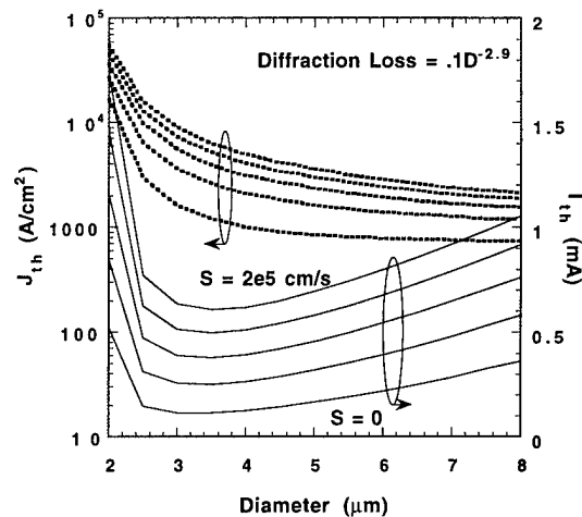
Figure 2: Modelled threshold currents with no waveguide loss.
