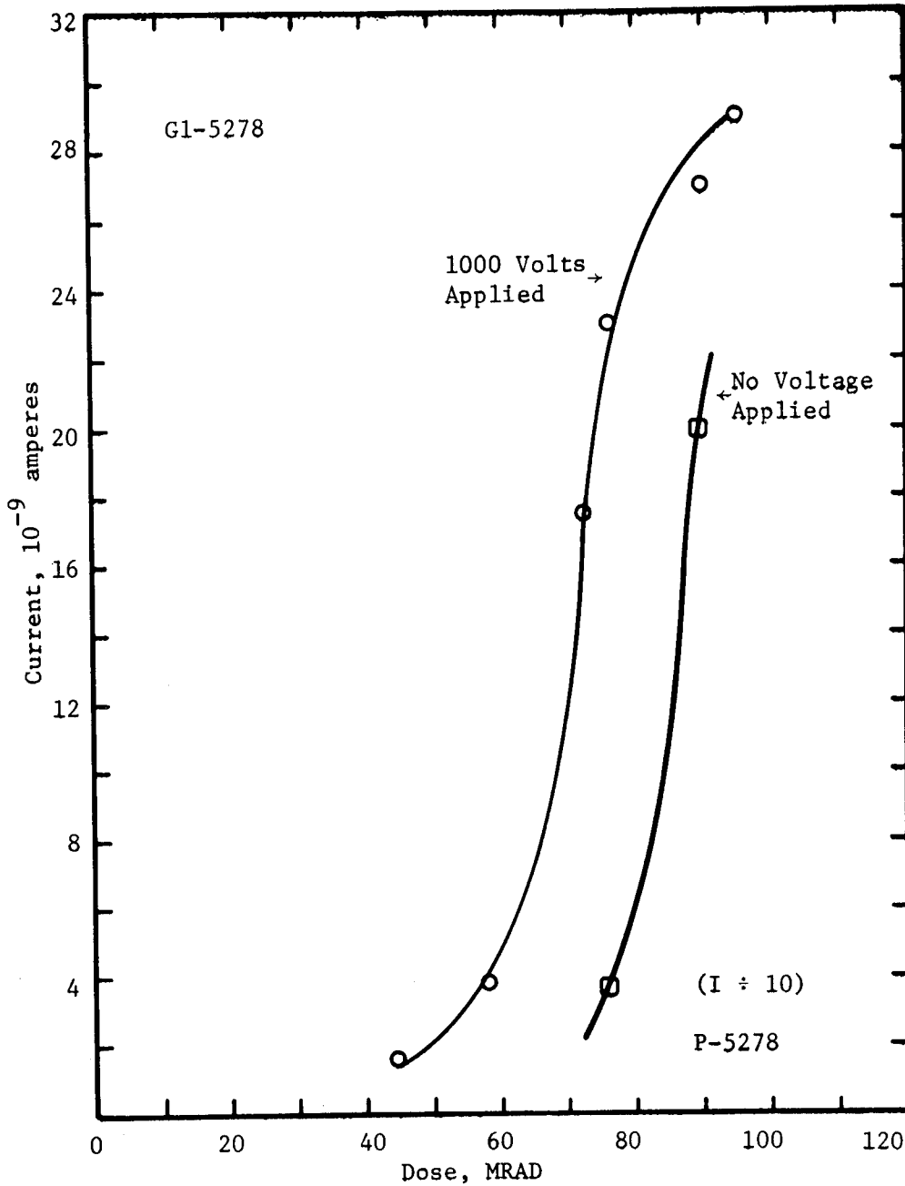
Figure 12. CURRENT IN 10 MIL PET AS A FUNCTION OF THE ACCUMULATED \gamma -DOSE. Applied voltage = 1000 volts, area = 3.88 cm 2 , 830 Å aluminum electrodes, dose rate = 0.19 Mrad hr -1 , ○...1000 volts applied during irradiation, □...no voltage applied during irradiation.
