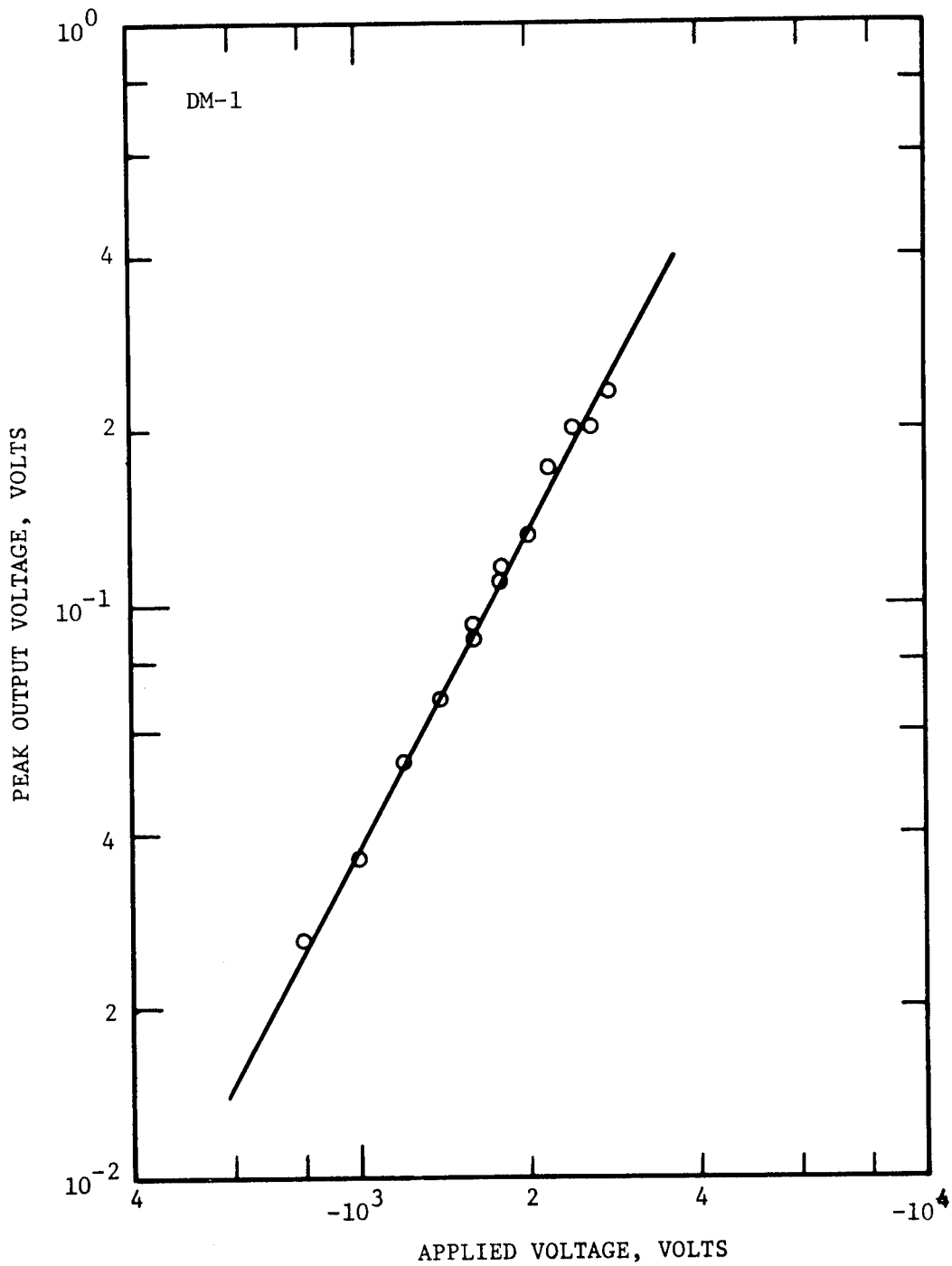
Figure 31. PEAK OUTPUT VOLTAGE VERSUS APPLIED VOLTAGE FOR A-AXIS OF DIMETHYLTEREPHTHALATE. 300 Å silver electrodes with silver paste guard ring, thickness = 0.45 cm, area = 0.37 cm 2 , R = 7 x 10 5 ohms.
