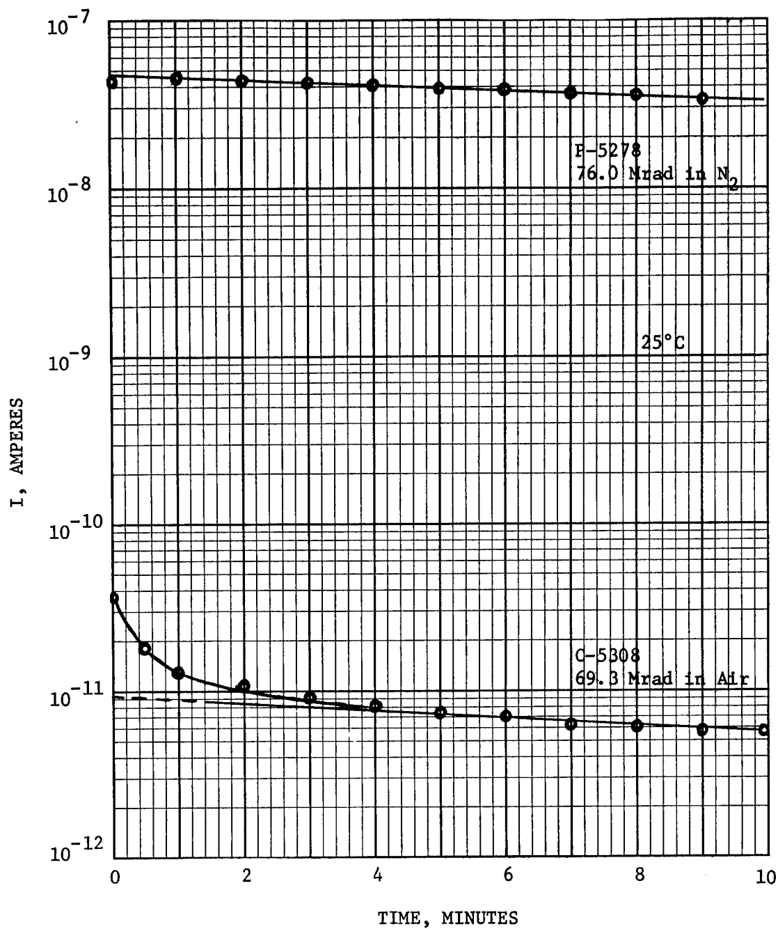
Figure 14. COMPARISON OF FIRST ORDER CURRENT DECAY OF 10 MIL PET IRRADIATED IN N_2 AND IN AIR. No voltage applied during irradiation, applied voltage during measurement = 1000 volts.
