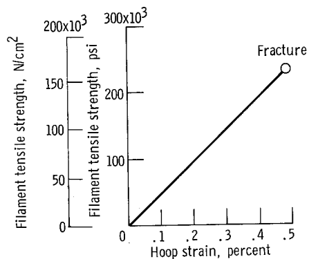
Figure 4. - Stress-strain diagram for single-cycle test of Thornel-50 epoxy resin cylinder. Filament tensile modulus, 48.8 \times 10^6 psi ( 33.5 \times 10^6 N/cm 2 ).
