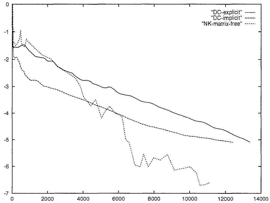
Figure 4: Steady-state residual versus CPU time (in seconds) for steady transonic flow at convergence for the 8 \times 8 decompositions, employing the block Jacobi algorithm combined with defect-correction procedures with explicit (DC-explicit) and implicit (DC-implicit) boundary conditions, and with Newton-Krylov matrix-free (NK-matrix-free) methods on the fine mesh.
