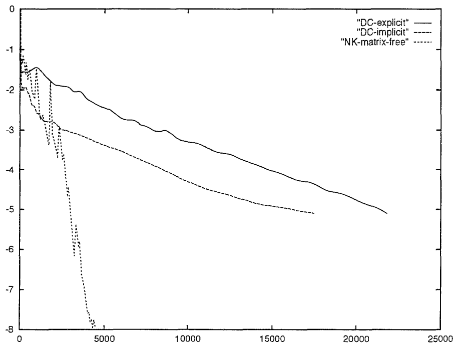
Figure 2: Steady-state residual versus CPU time (in seconds) for steady transonic flow at convergence for the 8 \times 8 decompositions, employing the additive Schwarz algorithm combined with defect-correction procedures with explicit (DC-explicit) and implicit (DC-implicit) boundary conditions, and with Newton-Krylov matrix-free (NK-matrix-free) methods on the coarse mesh.
