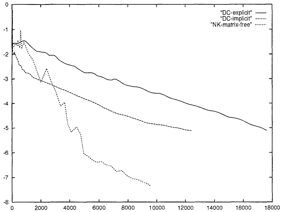
Figure 6: Steady-state residual versus CPU time (in seconds) for steady transonic flow at convergence for the 8 \times 8 decompositions, employing the multiplicative Schwarz algorithm combined with defect-correction procedures with explicit (DC-explicit) and implicit (DC-implicit) boundary conditions, and with Newton-Krylov matrix-free (NK-matrix-free) methods on the fine mesh.
