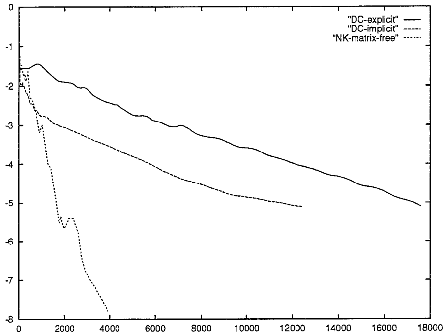
Figure 3: Steady-state residual versus CPU time (in seconds) for steady transonic flow at convergence for the 8 \times 8 decompositions, employing the multiplicative Schwarz algorithm combined with defect-correction procedures with explicit (DC-explicit) and implicit (DC-implicit) boundary conditions, and with Newton-Krylov matrix-free (NK-matrix-free) methods on the coarse mesh.
