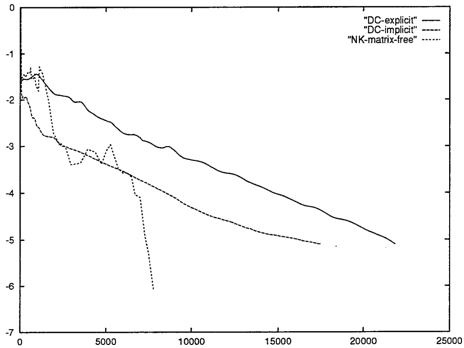
Figure 5: Steady-state residual versus CPU time (in seconds) for steady transonic flow at convergence for the 8 \times 8 decompositions, employing the additive Schwarz algorithm combined with defect-correction procedures with explicit (DC-explicit) and implicit (DC-implicit) boundary conditions, and with Newton-Krylov matrix-free (NK-matrix-free) methods on the fine mesh.
