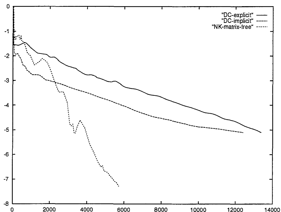
Figure 1: Steady-state residual versus CPU time (in seconds) for steady transonic flow at convergence for the 8 \times 8 decompositions, employing the block Jacobi algorithm combined with defect-correction procedures with explicit (DC-explicit) and implicit (DC-implicit) boundary conditions, and with Newton-Krylov matrix-free (NK-matrix-free) methods on the coarse mesh.
