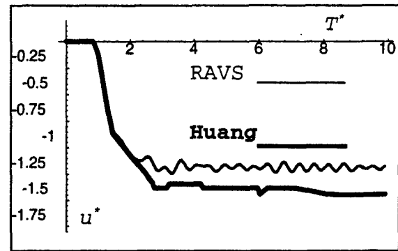
Figure 9. Nondimensional velocity vs. time, \theta=\pi , q=0 , M=4.4189 .
