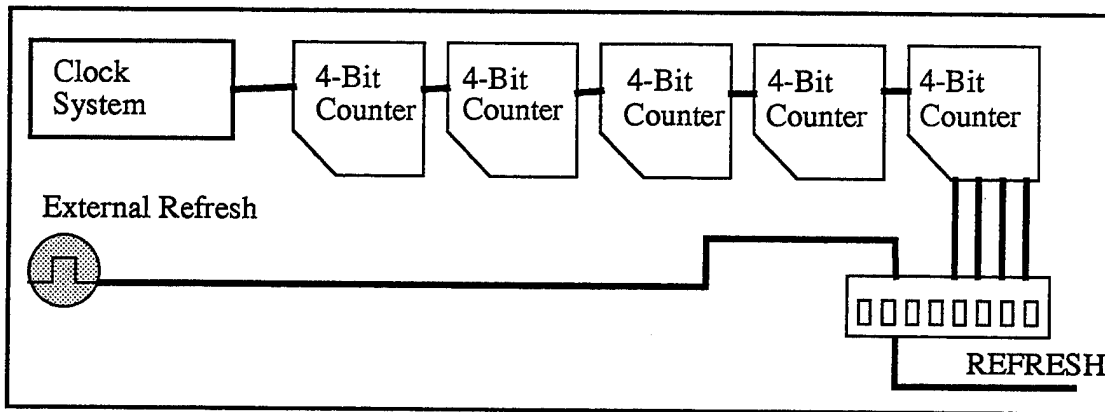
Figure 3.8. Refresh System.
