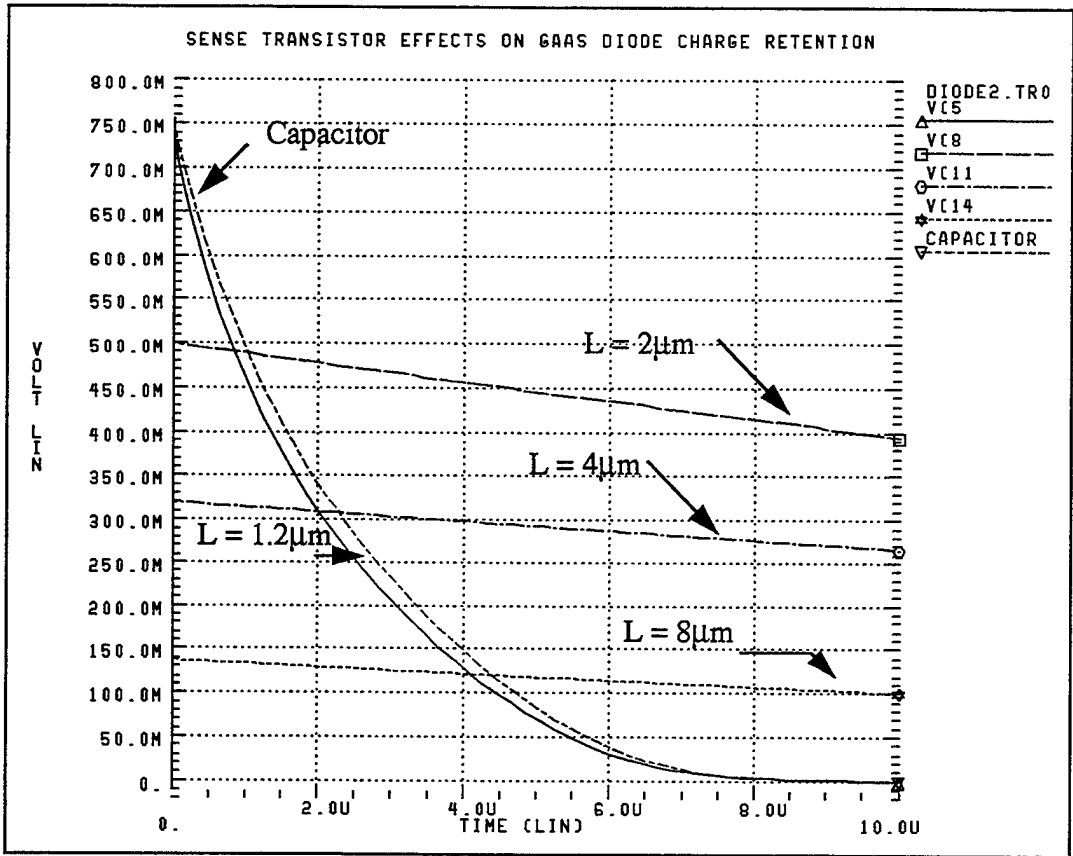
Figure 5.6. Sense Transistor Effect on Charge Retention.
