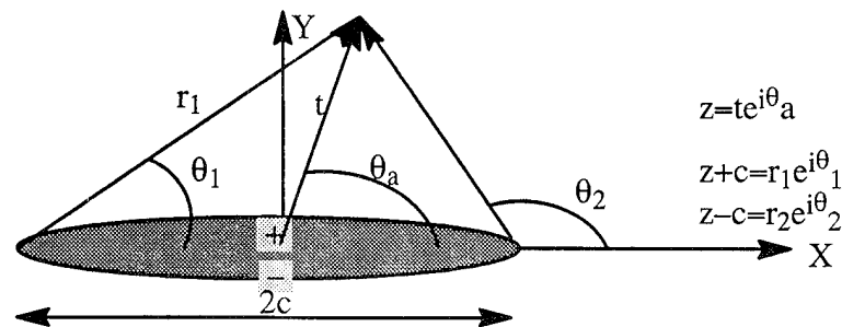
Figure C.3. Geometry for the Function X(z)
