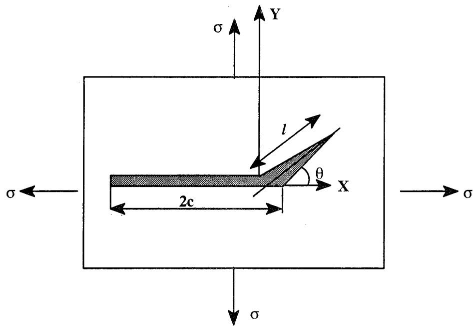
Figure 15. Loading Condition 1
