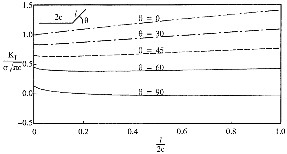
Figure 29. Variation of Normalized K_I with Normalized Kink Length l ( k = 0 , E_1/E_2 = 10 , \theta_m = 90^\circ )
