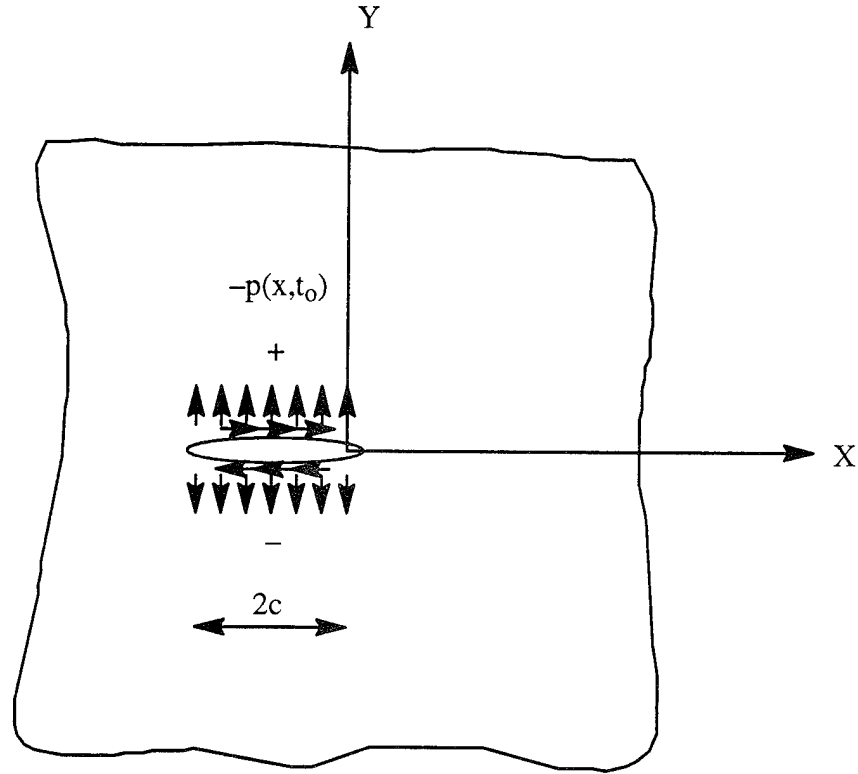
Figure A.2. Geometry of Pressurized Main Crack
