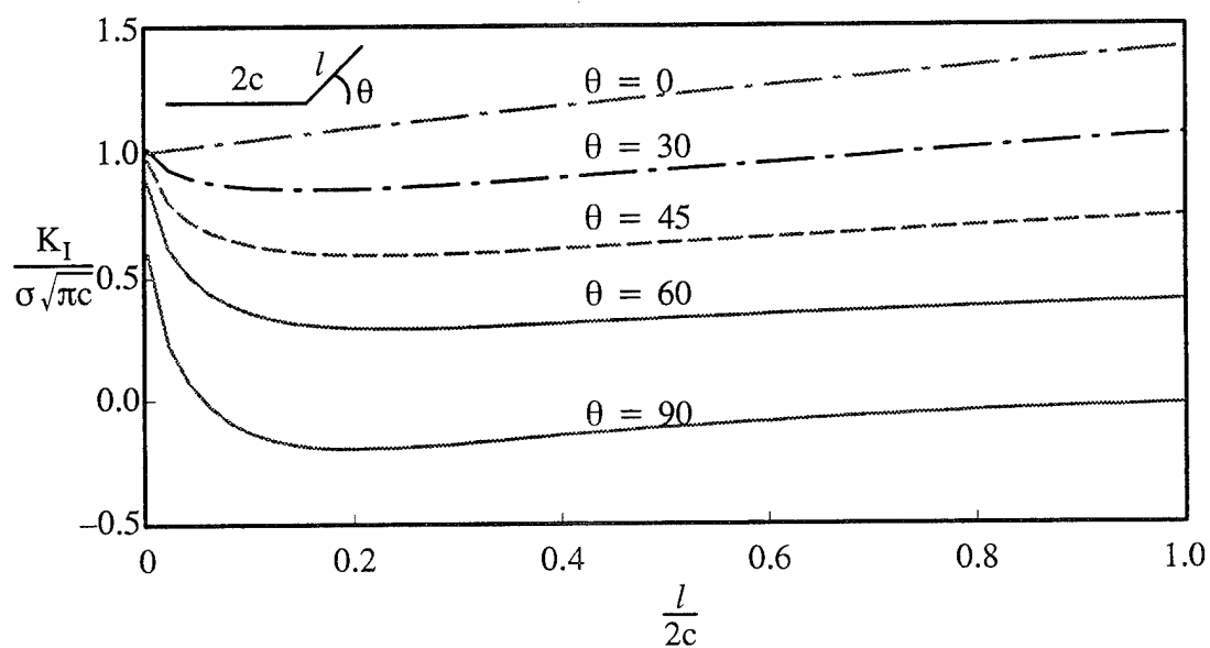
Figure 31. Variation of Normalized K_I with Normalized Kink Length l ( k = 0 , E_1/E_2 = 10.0 , \theta_m = 0 )
