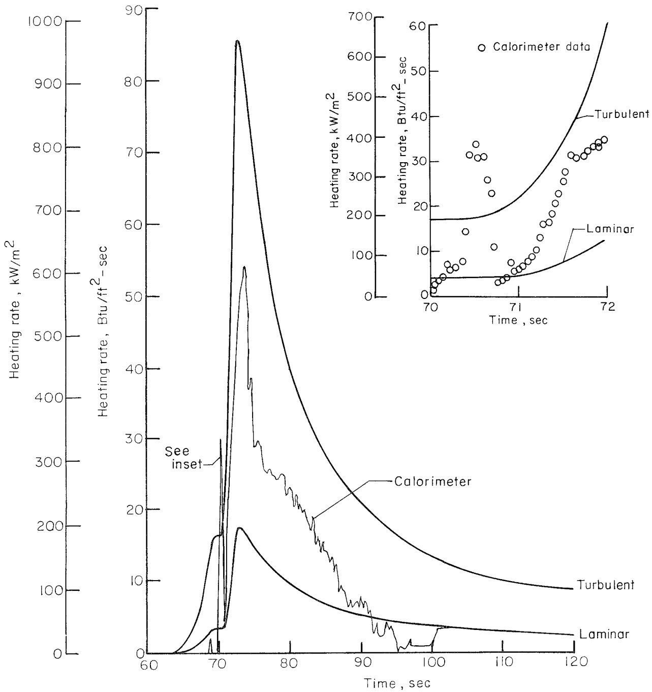
Figure 23.- Computed laminar and turbulent heating rates superimposed on heating rates for calorimeter C-1 at cylinder station 1.
