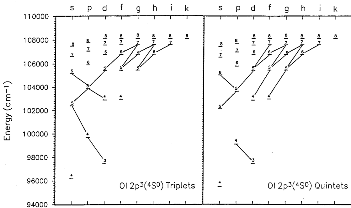
Figure 5. Energy level diagram illustrating the major transitions observed in the line emission spectrum from 3.5 to 13.0 \mu\text{m} .
