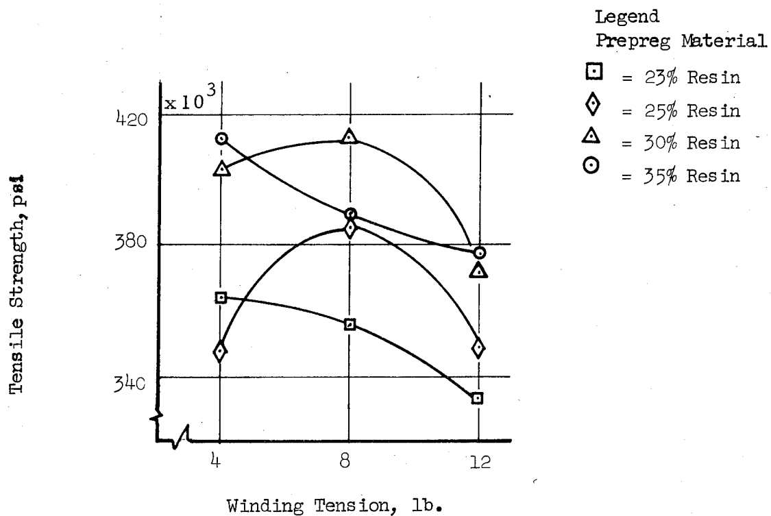
FIGURE 10: Normalized Fiber Properties of Gemon L/12-End S-Glass NOL Rings as a Function of Winding Tension
