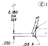
DETAIL B (W) SCALE: 10/1
