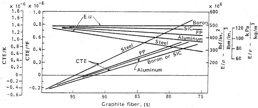
Figure 6. - Effect of replacing VSB-32 fiber with other selected fibers in a unidirectional layup.
