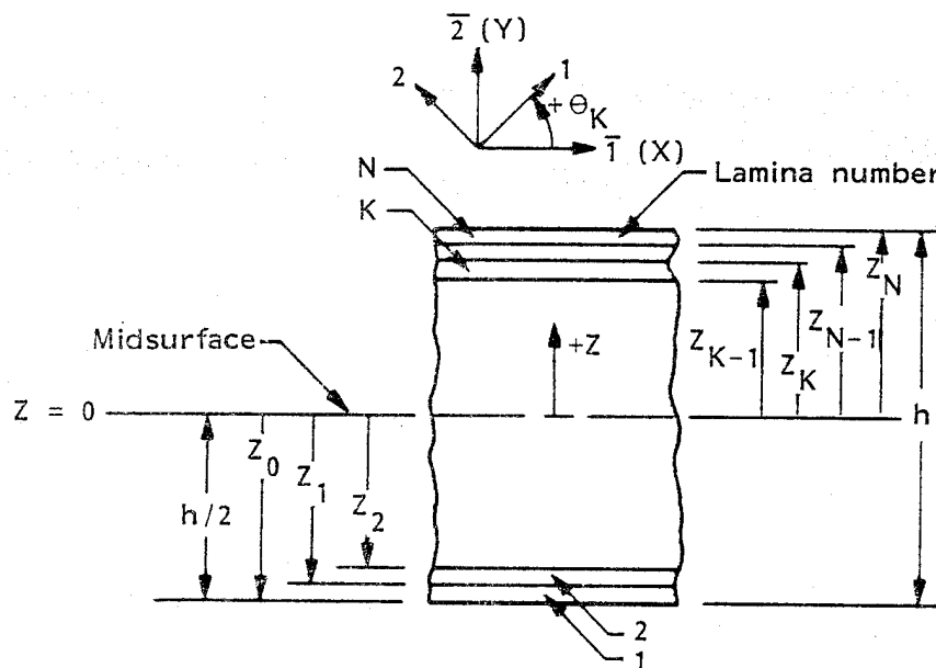
Figure 3. - Geometric representation of a laminate.
