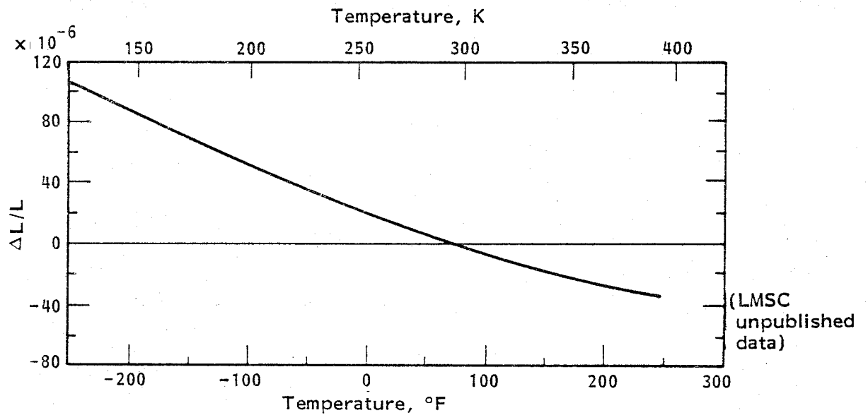
Figure 22. - Thermal expansion of unidirectional HMS/3501-5A tape (0° fiber direction).
