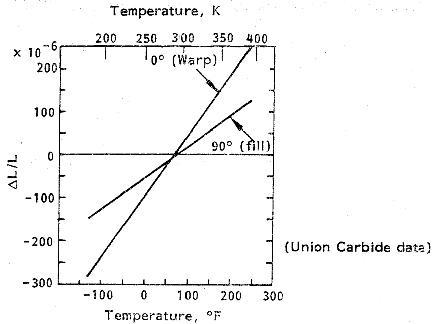
Figure 12. - Thermal expansion of Kevlar 49/X904B (120 style) fabric.
