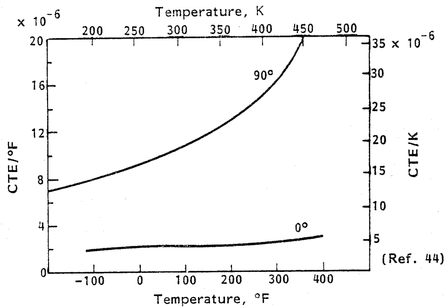
Figure 13. - Thermal expansion of unidirectional Boron/5505 tape.
