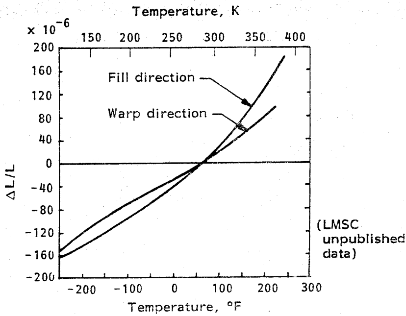
Figure 32. - Thermal expansion of HMS/E788 fabric.
