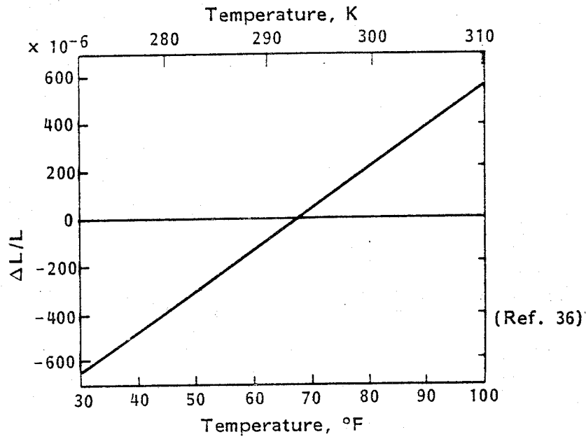
Figure 29. - Thermal expansion of HMS/759 unidirectional tape (90° direction).
