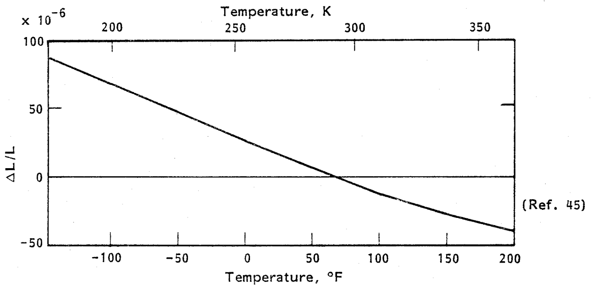
Figure 26. - Thermal expansion of HMS/CE339 unidirectional tape (0° fiber direction).
