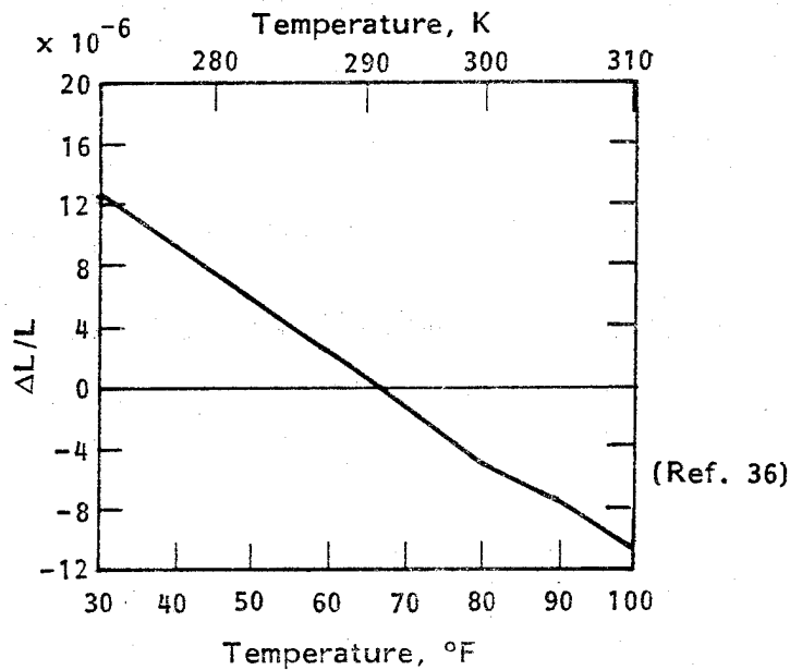
Figure 28. - Thermal expansion of HMS/759 unidirectional tape (0° direction).
