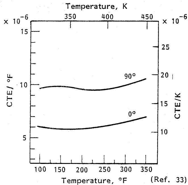
Figure 38. - Thermal expansion of 104 glass scrim cloth.
