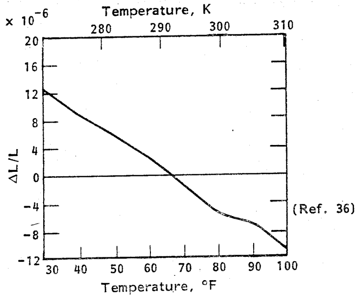
Figure 24. - Thermal expansion of HMS/3501 unidirectional tape (0° direction).
