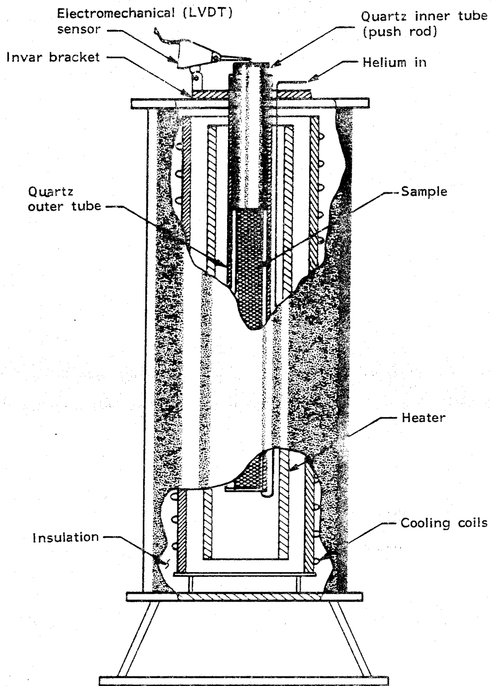
Figure 9. - Electromechanical dilatometer.
