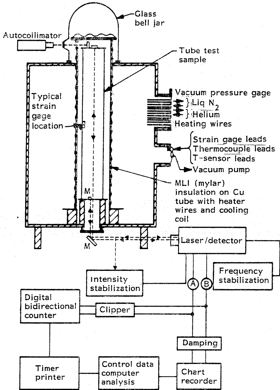
Figure 11. - Laser interferometer and dimensional stability test apparatus.
