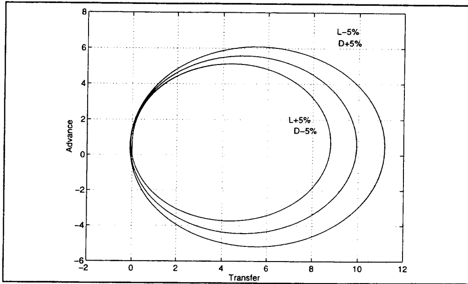
Figure 26 Advance vs. Transfer comparison with constant beam
