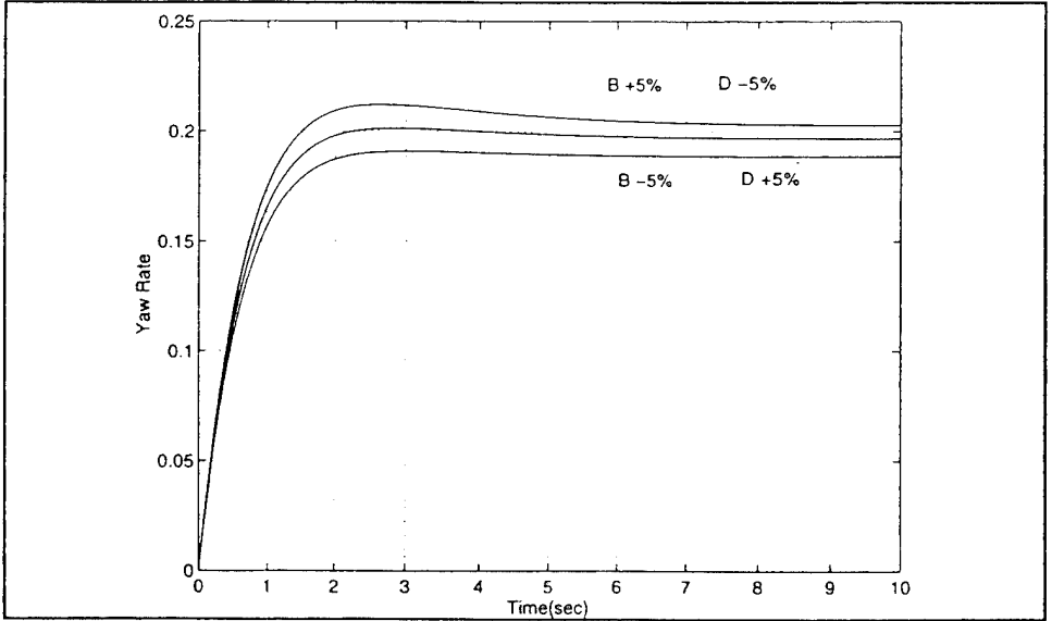
Figure 29 Yaw Rate vs. Time comparison with constant length
