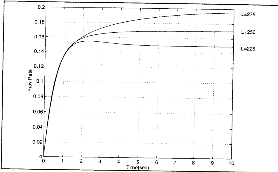
Figure 16 Yaw Rate vs. Time for Nonlinear Model at varying lengths
