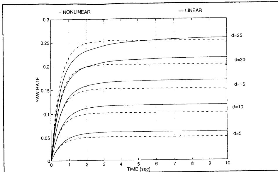
Figure 22 Yaw Rate vs. Time comparison between Nonlinear Model and Nomoto's Model at varying rudder angles
