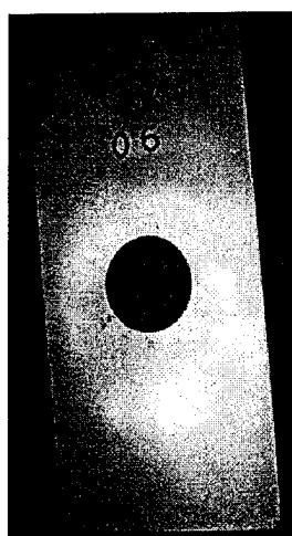
(a) (b) Figure 72. Small AL6XN stainless steel samples, 2.5x5.1 cm (1.0x2.0 in), exposed for 16 weeks: (a) aerated artificial seawater, (b) ozonated artificial seawater.
