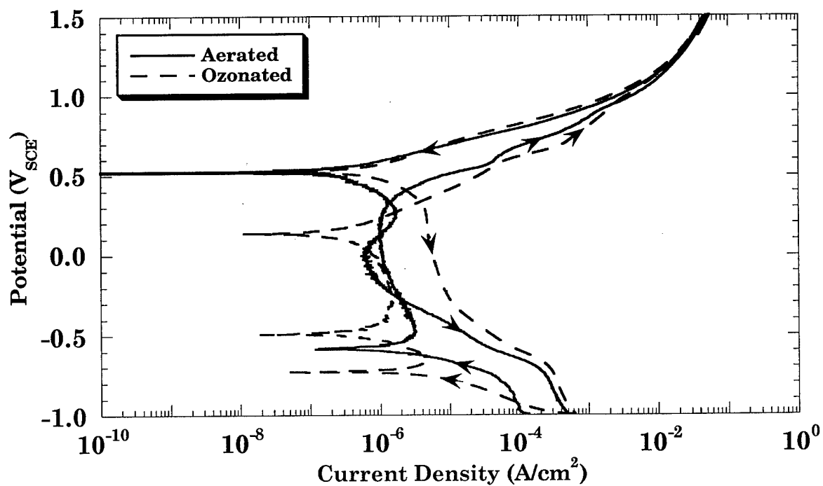
Figure 41. A comparison of the polarization curves of IN625 wires exposed to aerated or ozonated artificial seawater for 4 weeks.
