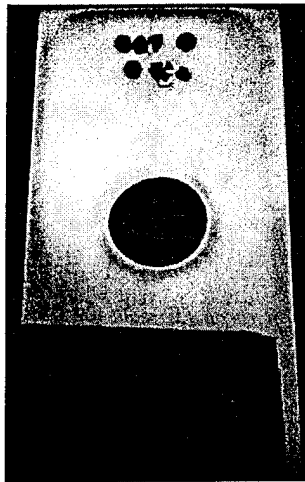
Figure 17. Small C276 crevice samples, 2.5x5.1 cm (1.0x2.0 in), exposed for 4 weeks: (a) aerated artificial seawater (b) ozonated artificial seawater.
