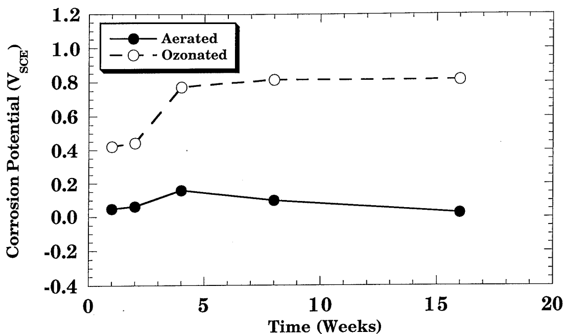
Figure 31. The steady state corrosion potential of C22 wire exposed to aerated or ozonated artificial seawater.
