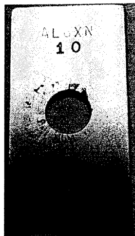
(a) (b) Figure 71. Small AL6XN stainless steel samples, 2.5x5.1 cm (1.0x2.0 in), exposed for 4 weeks: (a) aerated artificial seawater, (b) ozonated artificial seawater.
