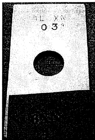
(a) (b) Figure 71. Small AL6XN stainless steel samples, 2.5x5.1 cm (1.0x2.0 in), exposed for 4 weeks: (a) aerated artificial seawater, (b) ozonated artificial seawater.
