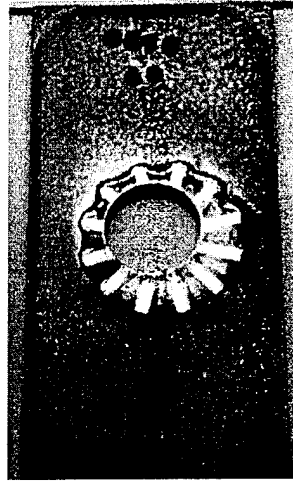
Figure 17. Small C276 crevice samples, 2.5x5.1 cm (1.0x2.0 in), exposed for 4 weeks: (a) aerated artificial seawater (b) ozonated artificial seawater.
