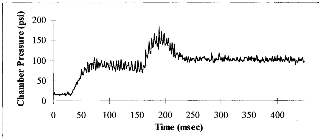
Figure 5.1 Pressure-Time Trace for Hybrid-Solid Fuel Ramjet Transition
