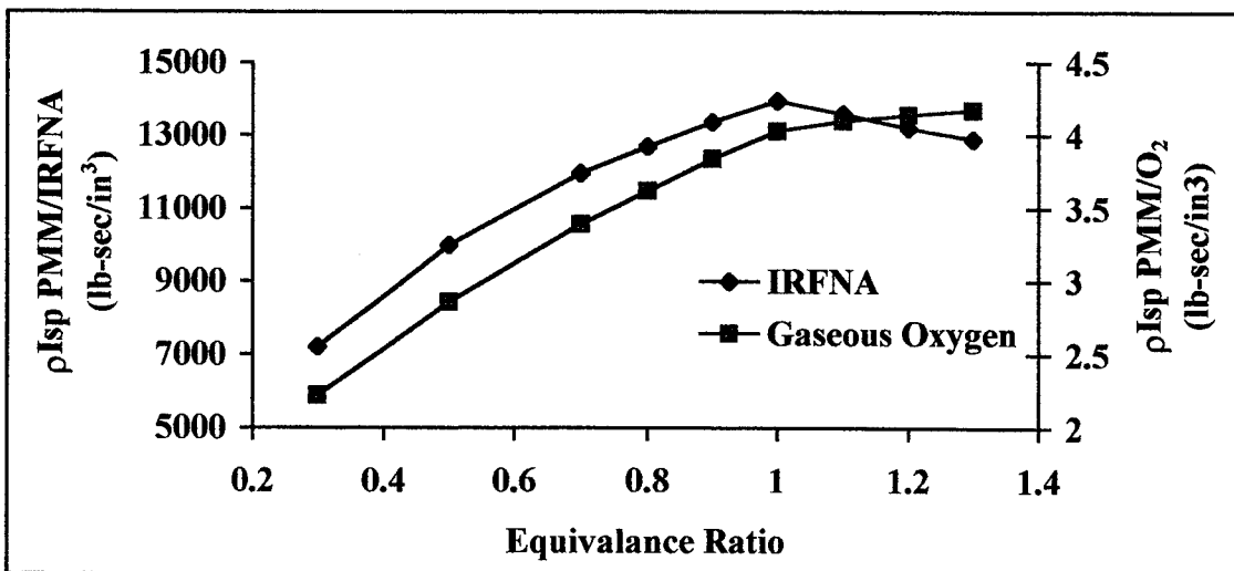
Figure 3.3 Density Specific Impulse vs. Equivalence Ratio
