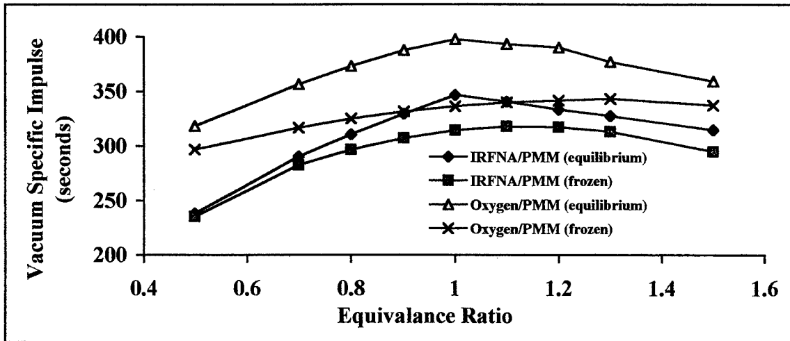
Figure 3.2 Specific Impulse vs. Equivalence Ratio
