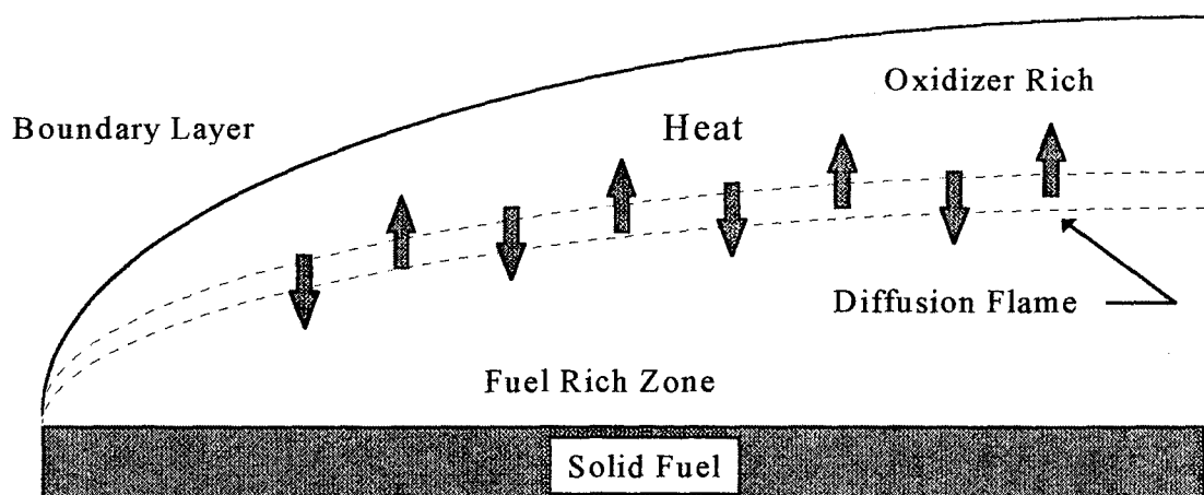
Figure 2.3 Hybrid Combustion Model
