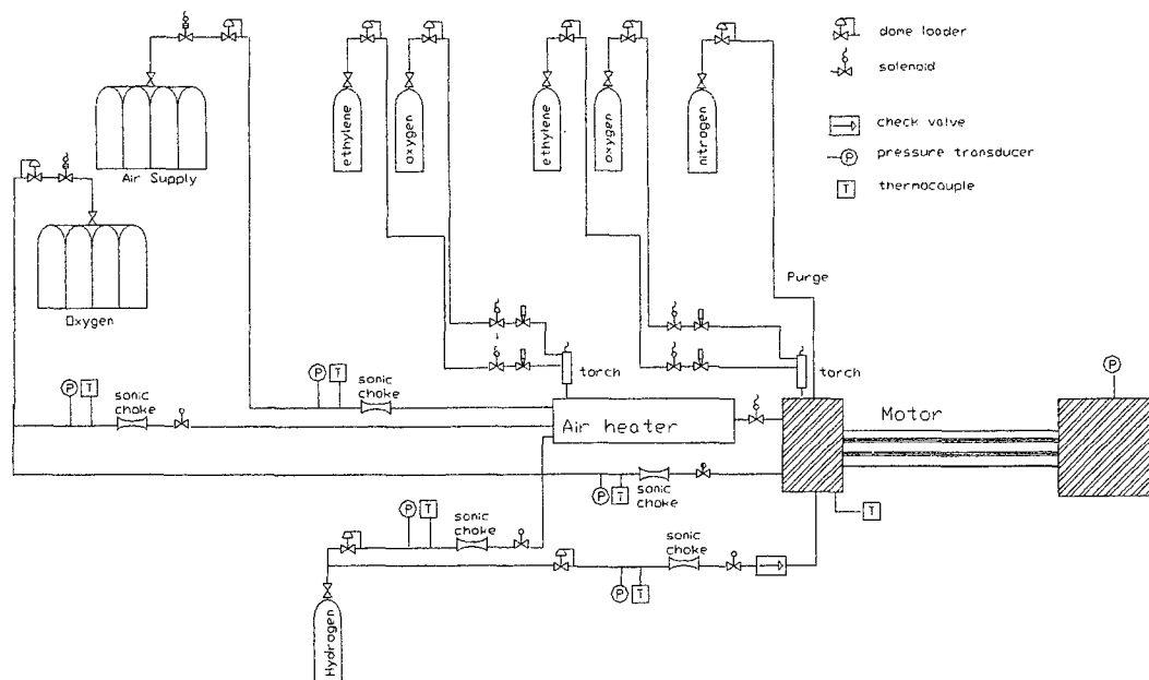
Figure 4.1 Schematic of Test Apparatus
