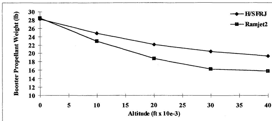
Figure 3.5 Booster Weight Comparison of H/SFRJ and IRR
