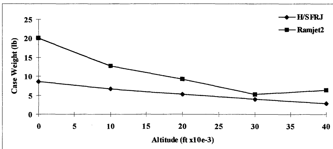
Figure 3.9 H/SFRJ and IRR Case Weight Comparison
