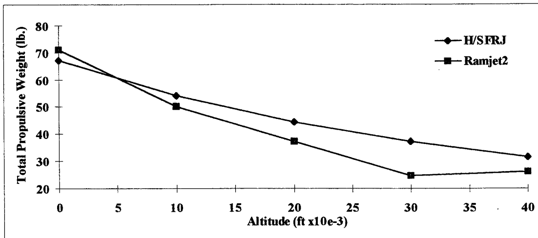
Figure 3.10 Total Propulsive Weight Comparison IRR vs. H/SFRJ
