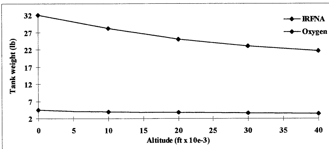
Figure 3.6 Tankage Weight for H/SFRJ
