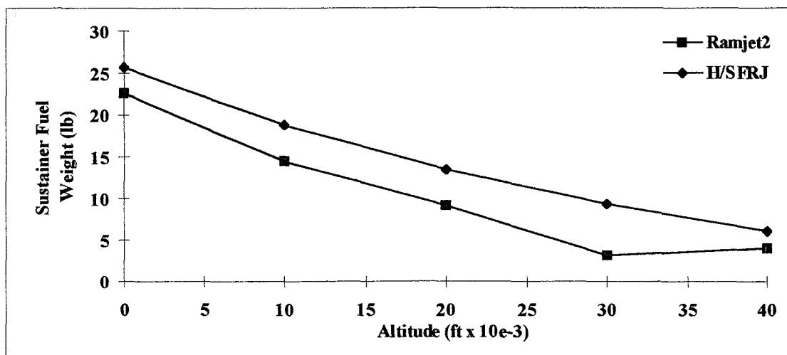
Figure 3.8 Sustainer Fuel Weight H/SFRJ vs. IRR
