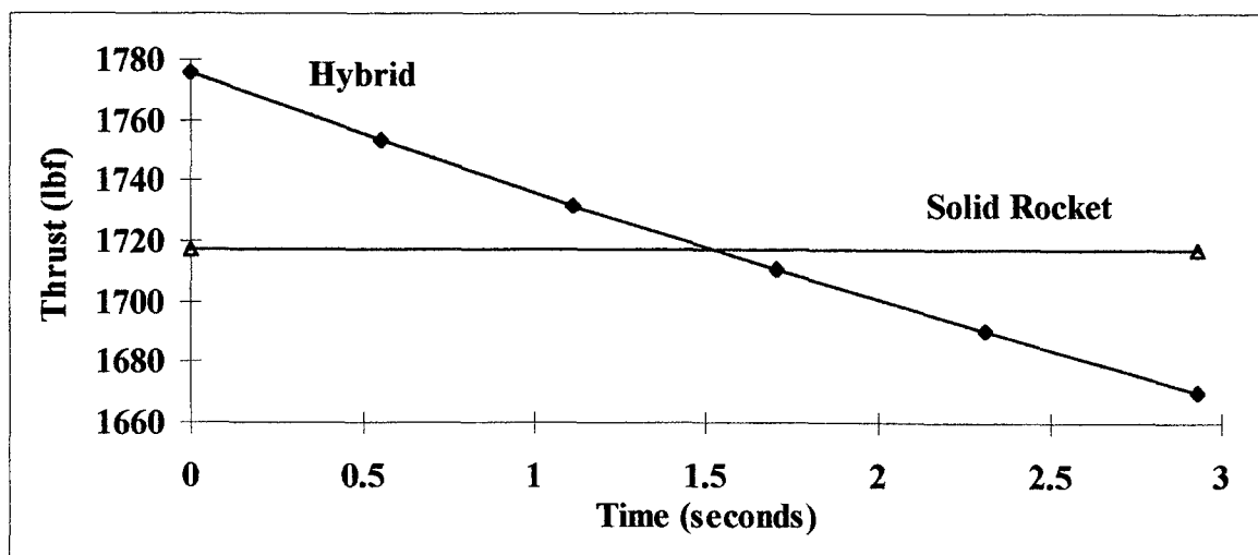
Figure 3.11 Thrust-Time Profile: Fixed Area Nozzle
