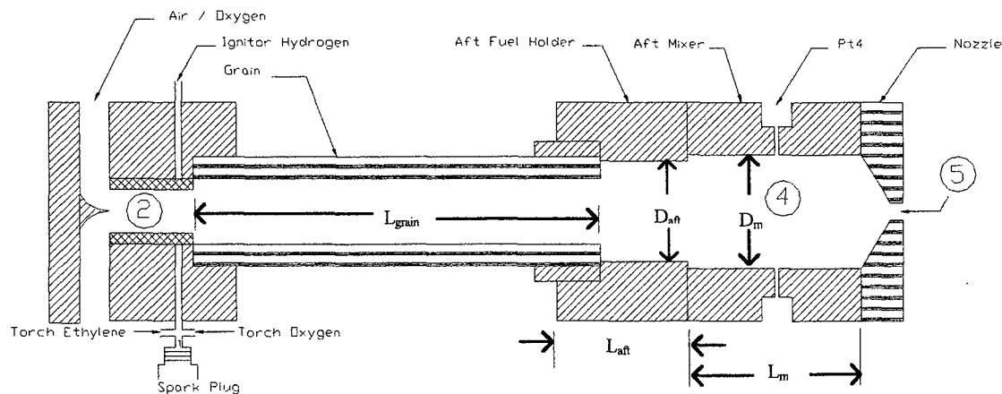
Figure 4.2 Hybrid / Solid-Fuel Ramjet Motor
