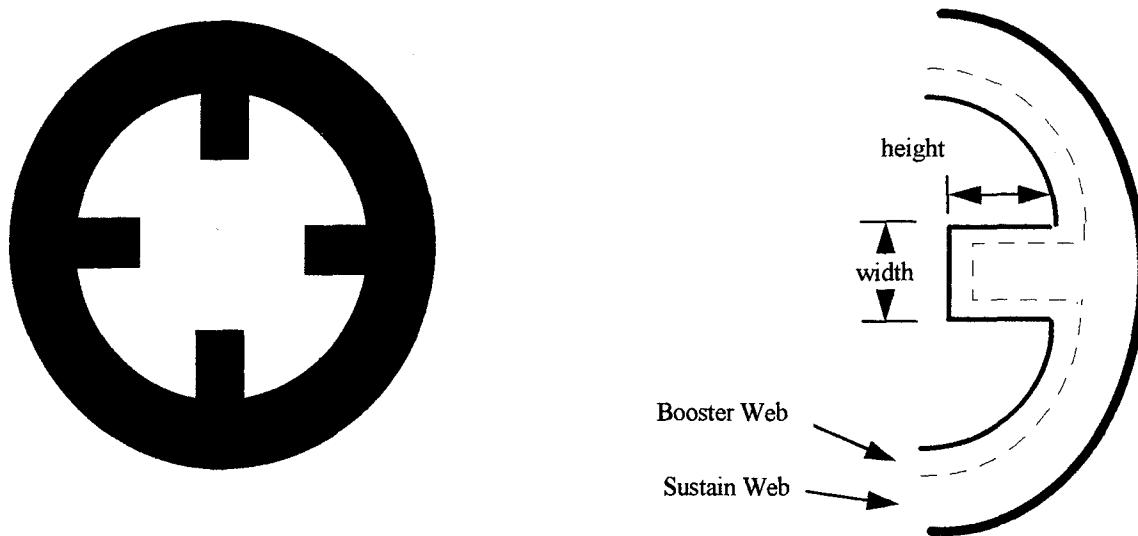
Figure 2.5 Final Configuration
