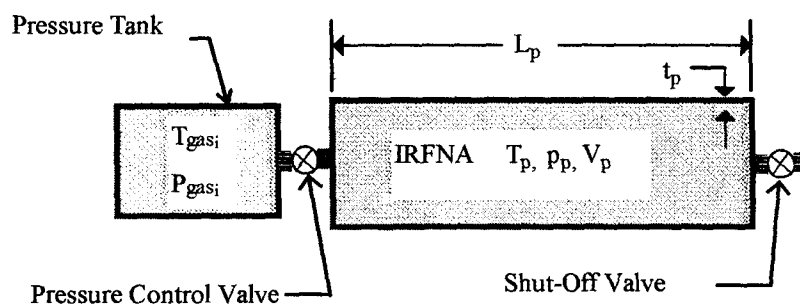
Figure 2.1 Pressure-Regulated Feed
