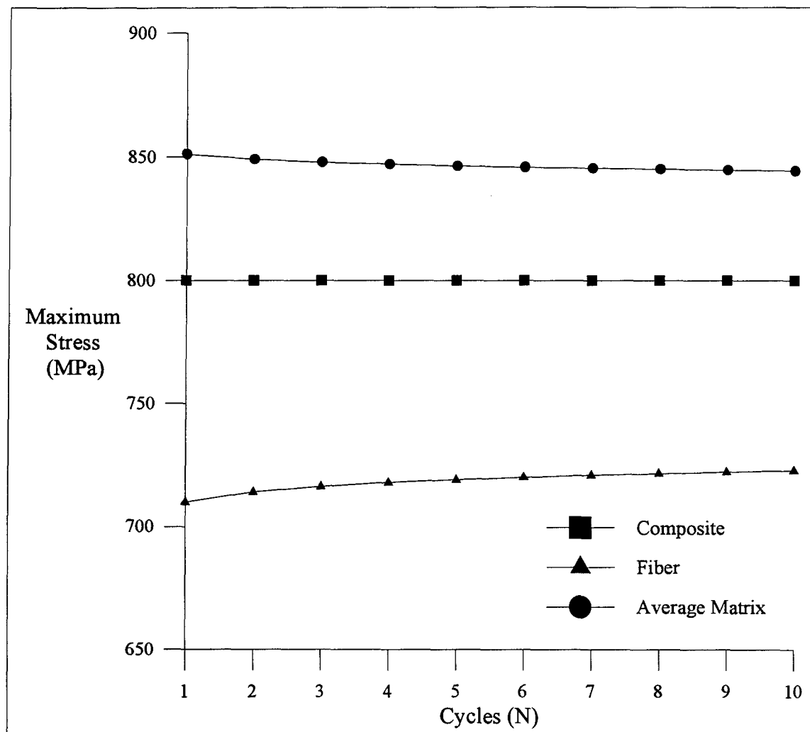
Figure B.1 Microstresses (10 Hz, 800 MPa, 427°C)
