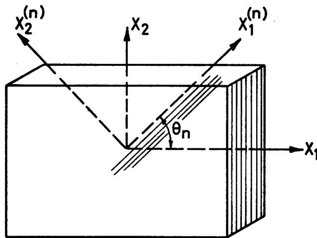
FIG. 2 LAMINATE
