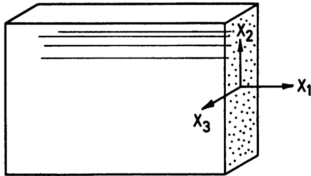
FIG. 1 UNIAXIALLY FIBER REINFORCED MATERIAL
