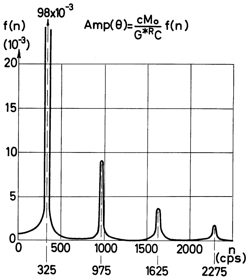
FIG. 3 AMPLITUDE OF ANGLE OF TWIST
