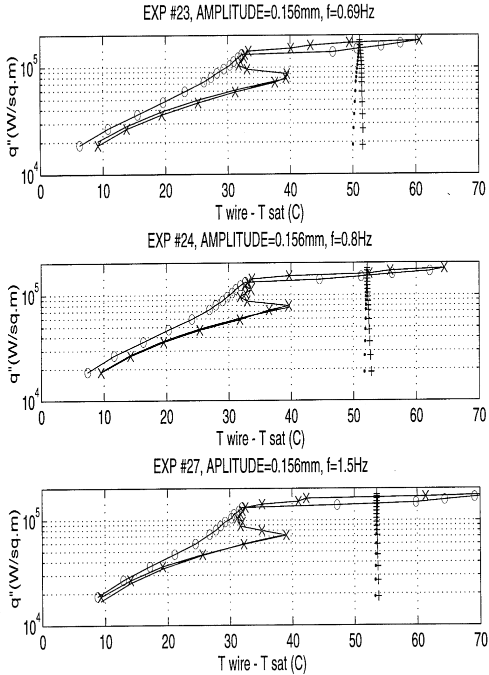
Figure 14b. Top Plot in Figure 14a is the Boiling Curve of FC-72. Other Five Plots in Figures 14a and 14b are the Boiling Curves with an Oscillation of Amplitude 0.156mm and Five Different Frequencies.
