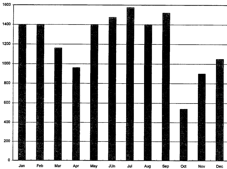
Figure 5. Temporal Distribution of MOODS Data for 1968
