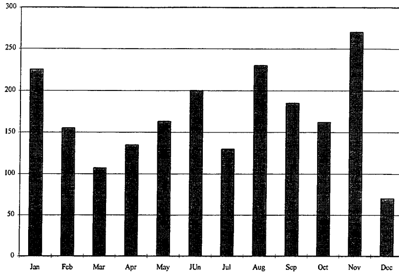
Figure 6. Temporal Distribution of MOODS Data for 1984
