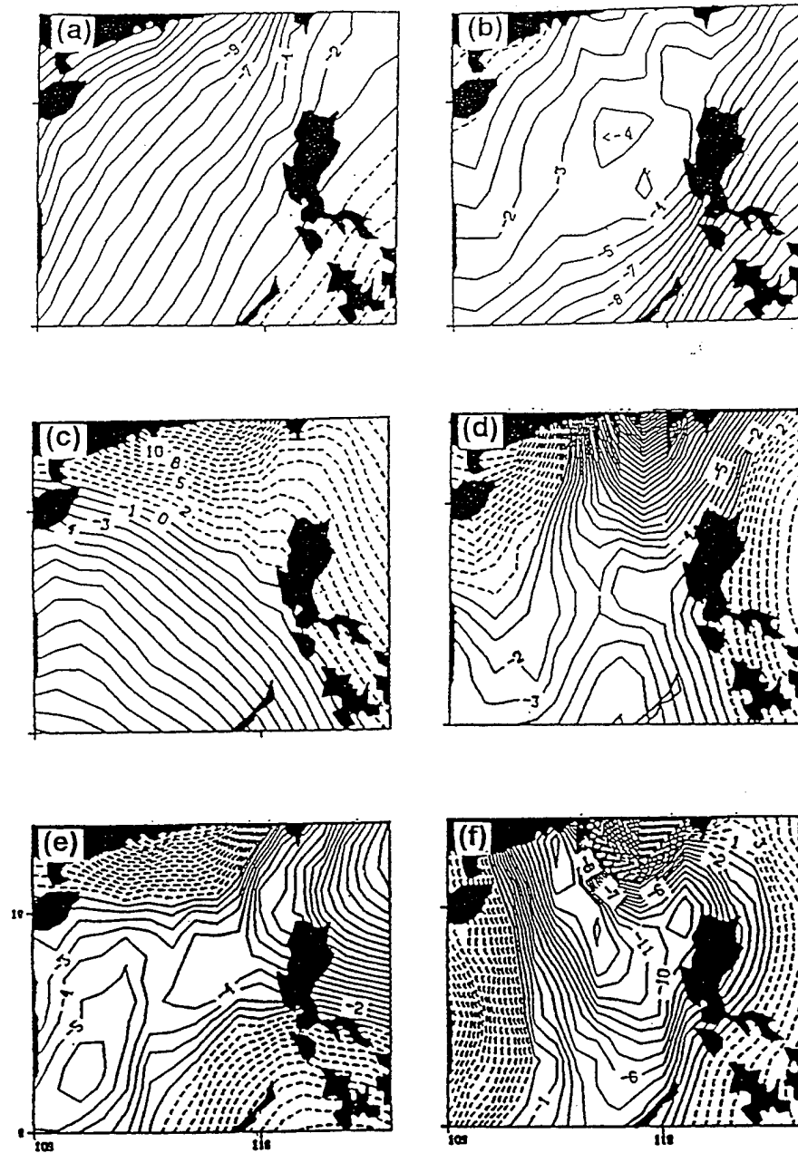
Figure 11. The First Six EOF Modes for the SST Anomalies ( ^{\circ} C) Computed From December-May During 1964-84; (a) EOF1, (b) EOF2, (c) EOF3, (d) EOF4, (e) EOF5, (f) EOF6. The EOF Model Values have been Multiplied by 10.
