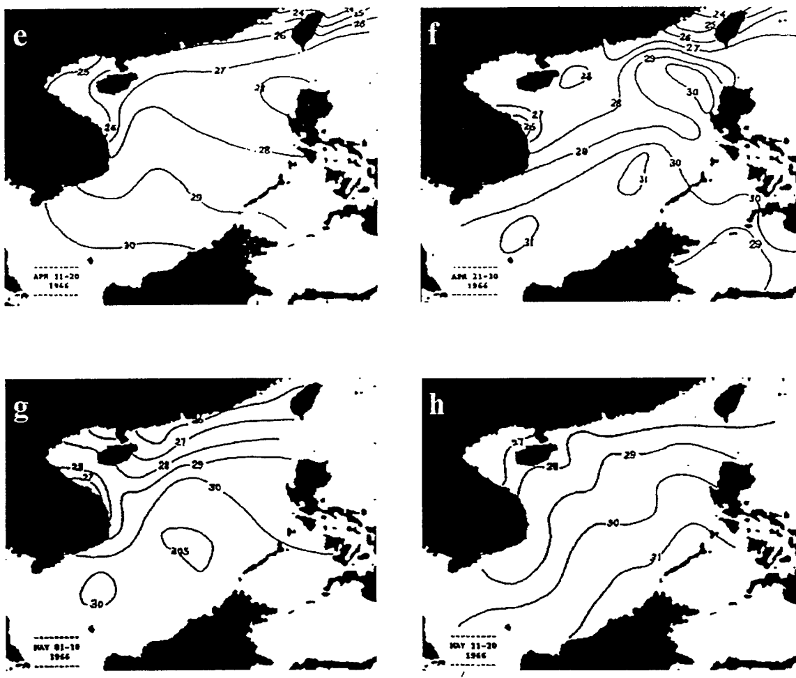
Figure 8. South China Sea SST Evolution in 1966: (e) April 11-20, (f) April 21-30, (g) May 1-10, (h) May 11-20 (From Chu and Chang, 1995).
