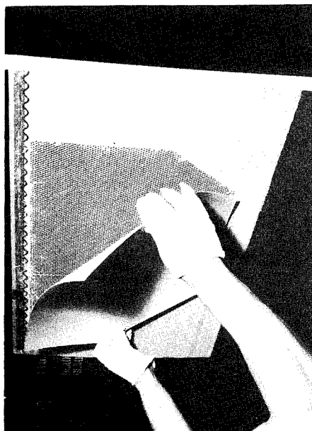
Figure 65. Apply Adhesive & Position Patch.
