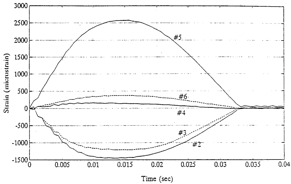
Figure 4. Experimental GRP Normal Strain. From Ref. [1]
