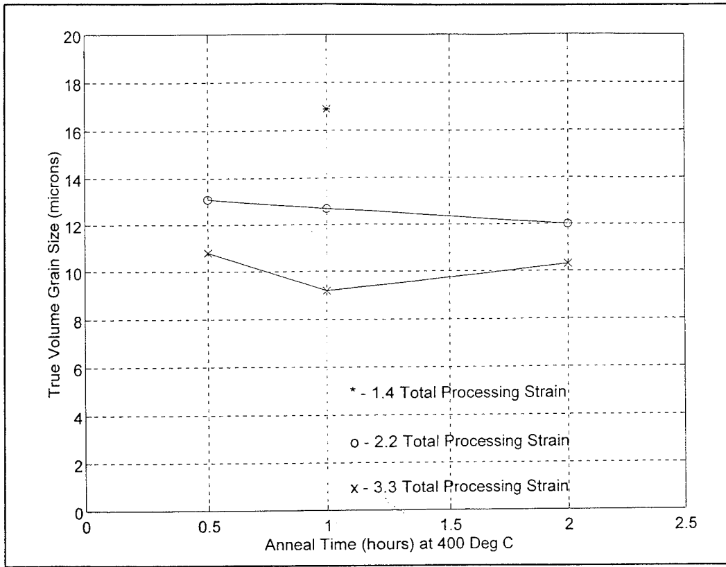
Figure 4.9: Graphical Representation of Table 4.2
