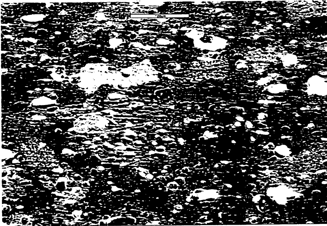
Figure 4.6: Microstructure for 1.4 Total Processing Strain
