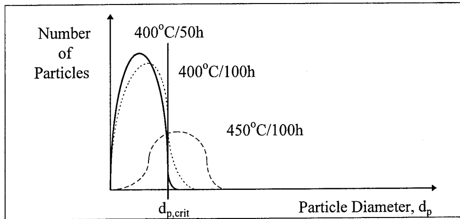
Figure 4.5: Precipitate Particle Size Distribution
