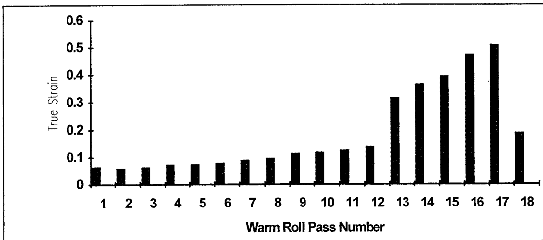
Figure 3.2: True Strain ( \epsilon ) vs. Warm Rolling Pass
