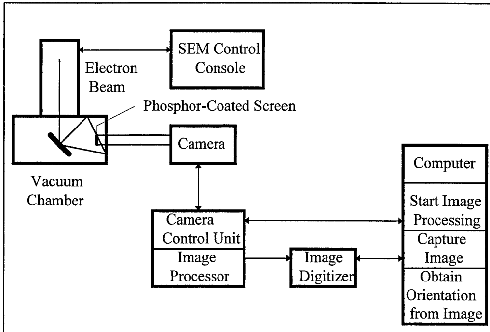
Figure 2.3: Equipment Configuration for Generating BKD Patterns
