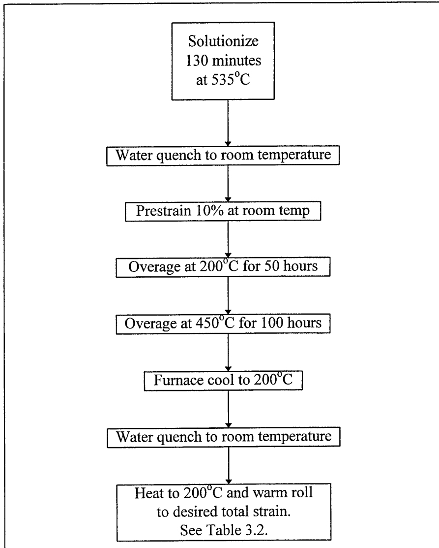
Figure 3.1: Thermomechanical Processing Steps
