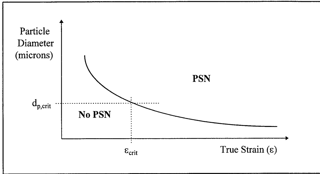
Figure 2.2: Particle Size and True Strain Relationship Necessary for PSN
