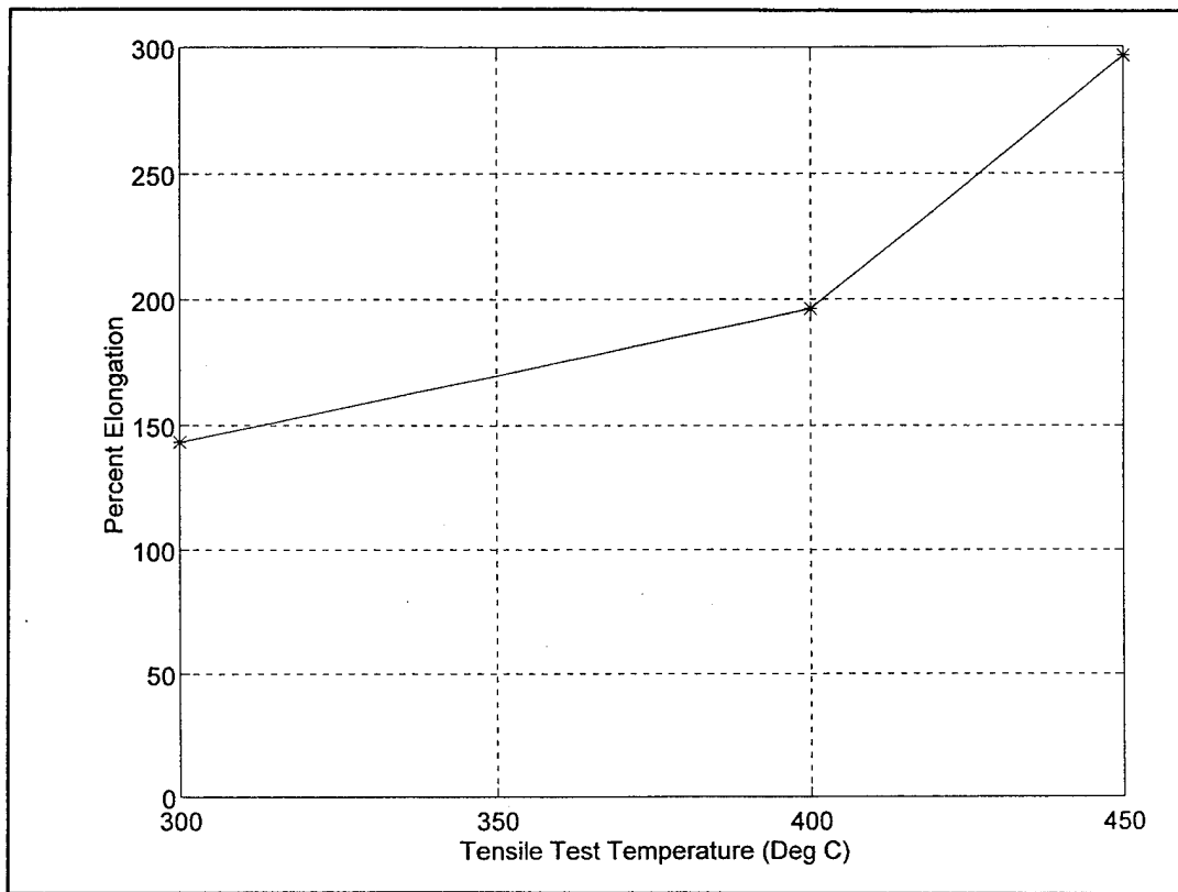
Figure 4.2: Ductility vs. Test Temperature
