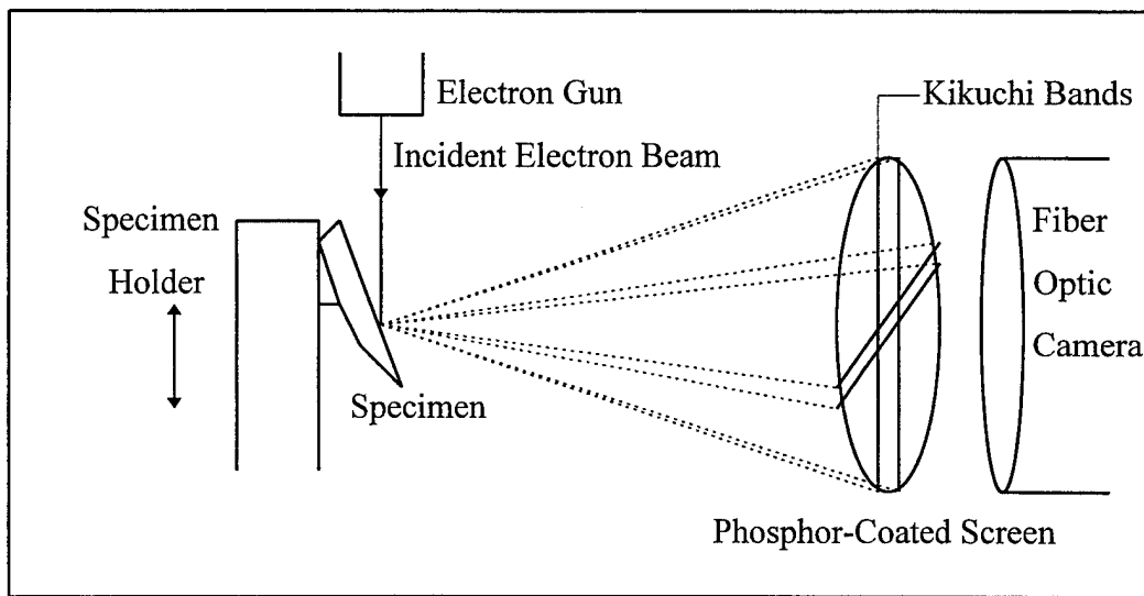
Figure 3.3: SEM Setup to Collect BKD Patterns
