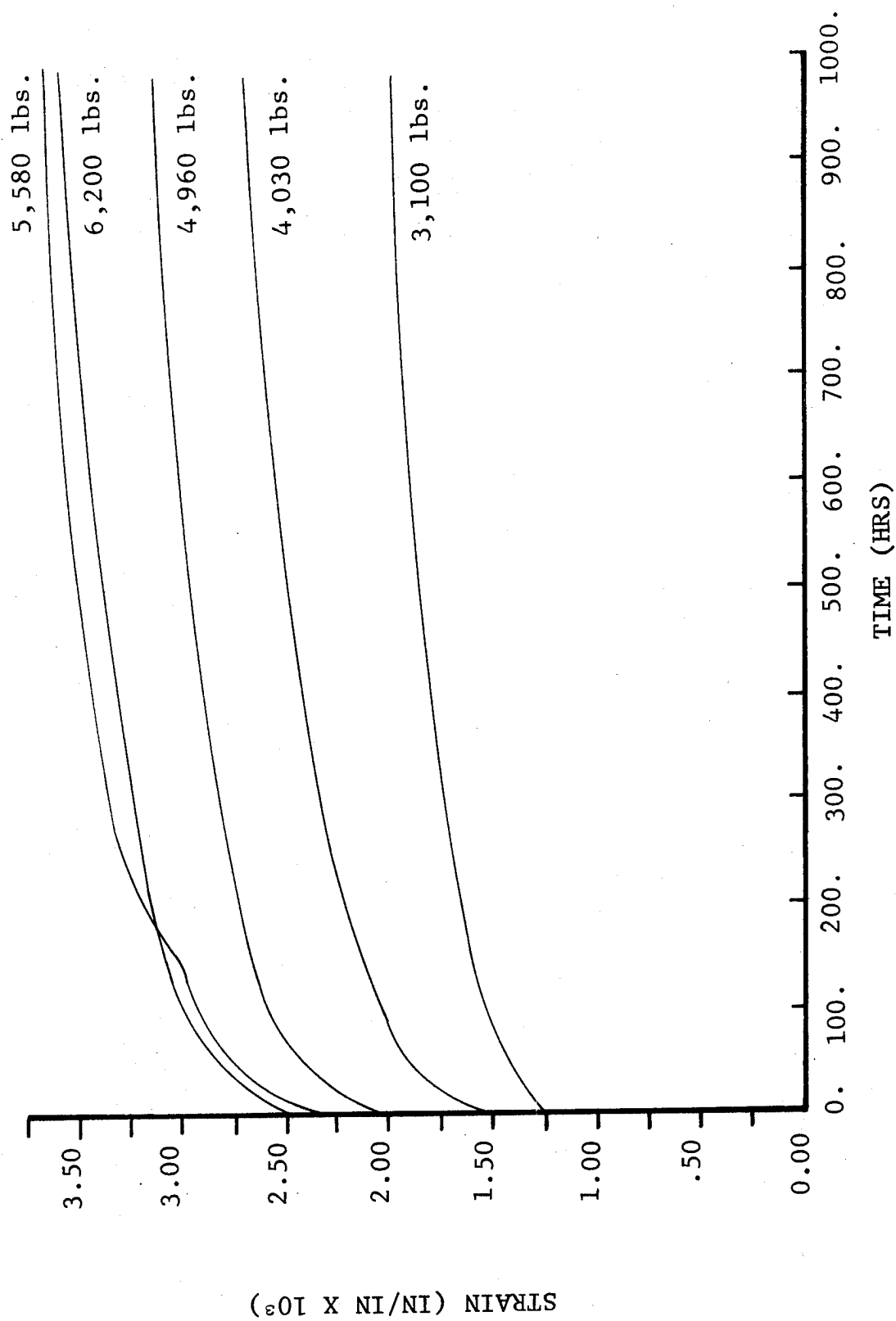
Figure 56. Creep Test Giba 4-inch Specimens
