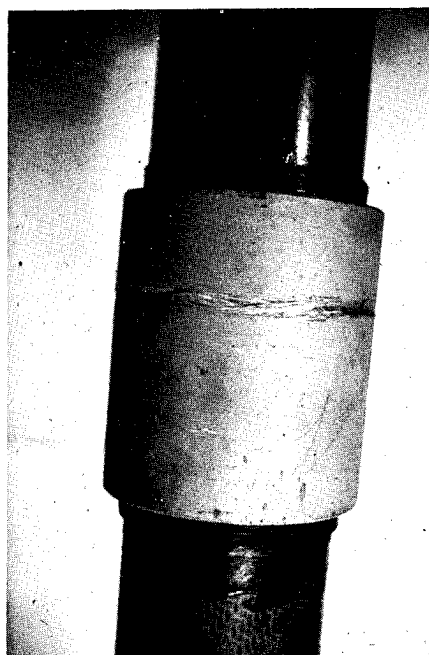
Figure 35. Coupling Failure
