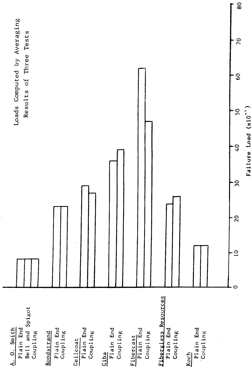
Figure 28. Results Of Tension Test On 4-inch Connections As Compared To Pipe Strength
