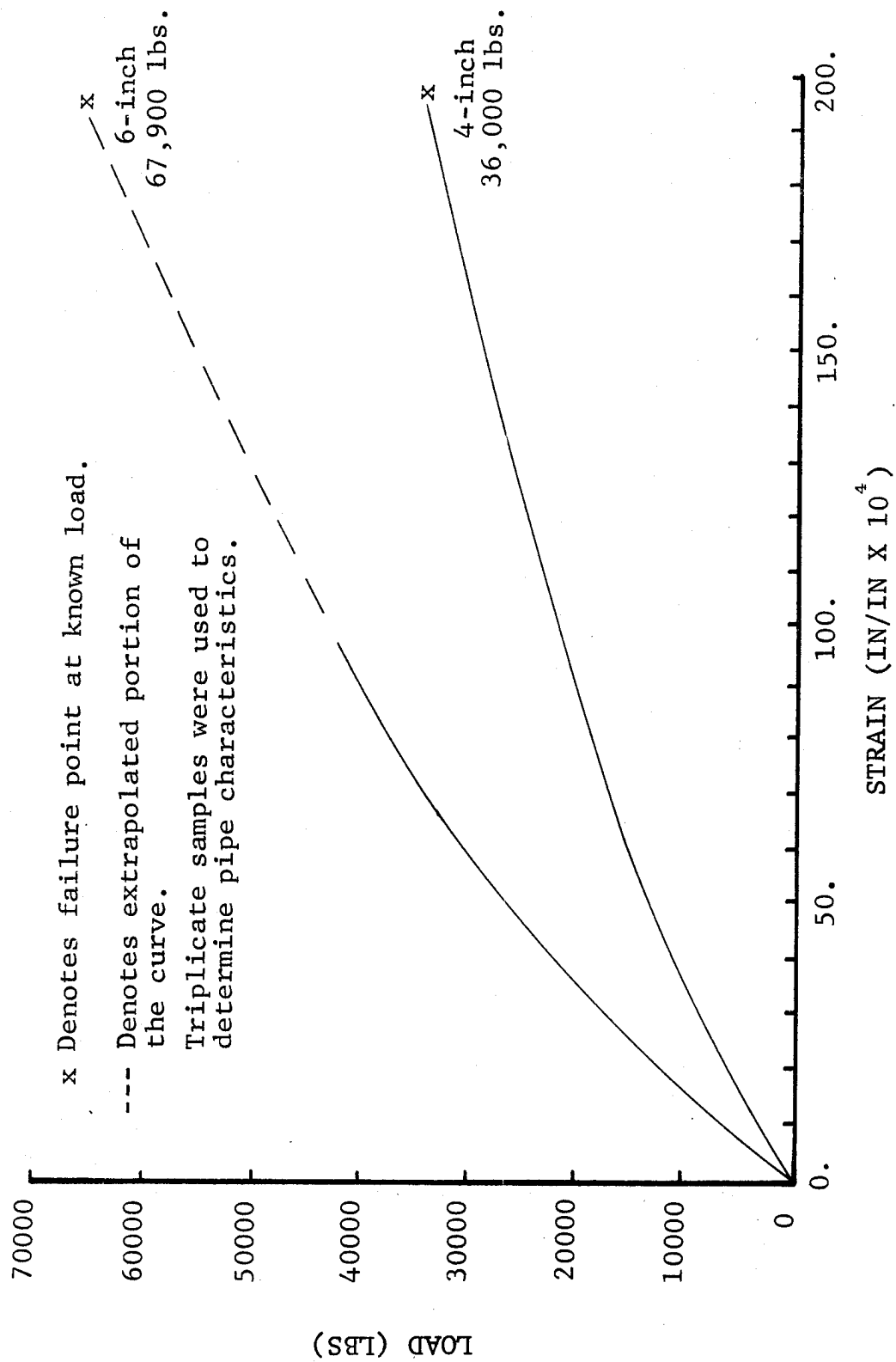
Figure 19. Tension Test Ciba
