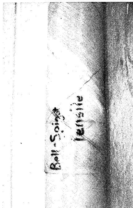
Figure 33. Example Of A Successful Bell And Spigot
