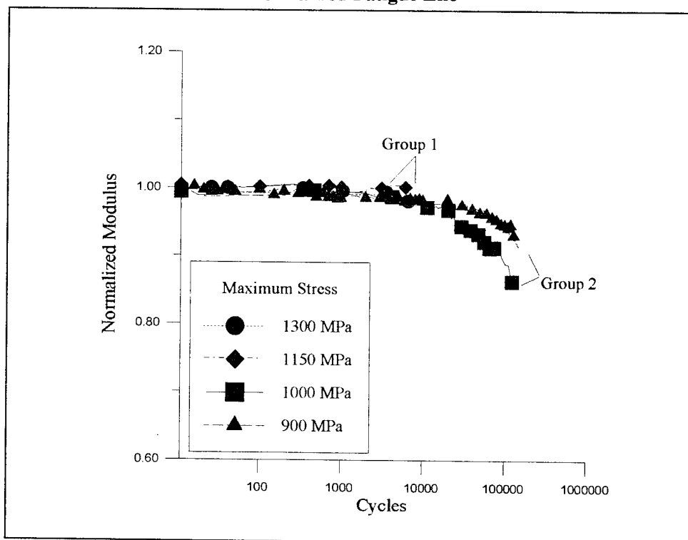
Figure 29b. Tension-Tension ( R_\sigma = 0.5 ) Modulus Histories: Cycles
