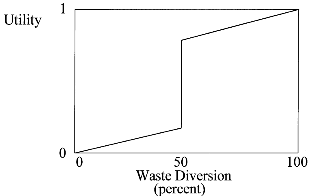
Figure 2. Utility Function for Waste Diversion
