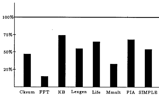
Figure 10: TIL Physical Memory Used Relative to SML/NJ
