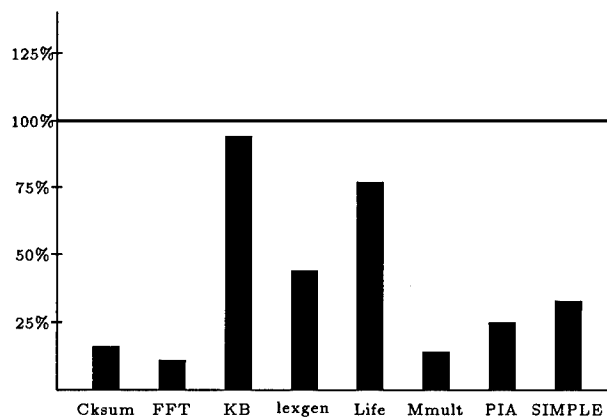
Figure 8: TIL Execution Time Relative to SML/NJ
