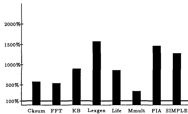
Figure 11: Til Compilation Time Relative to SML/NJ
