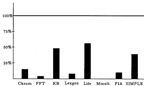
Figure 9: TIL Heap Allocation Relative to SML/NJ
