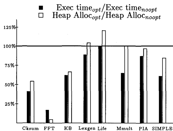
Figure 12: Effects of Loop Optimizations
