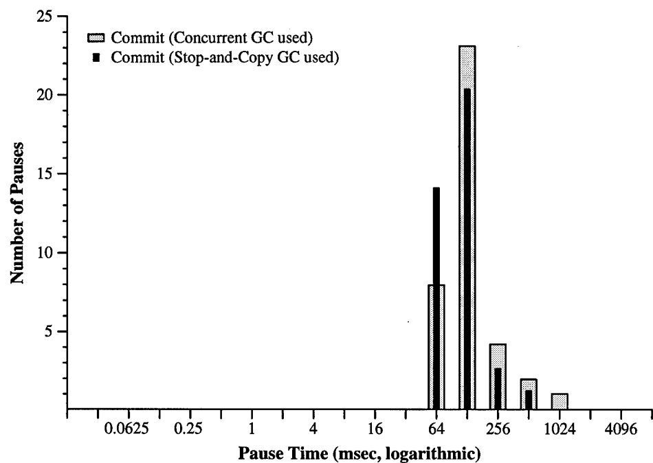
Figure 9.9: Compiler Pause Times (uniprocessor)
