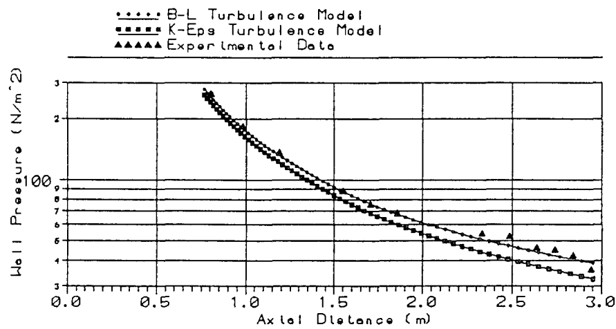
Fig. 57 Comparison of Static Wall Pressure for WL Mach 12 Nozzle
