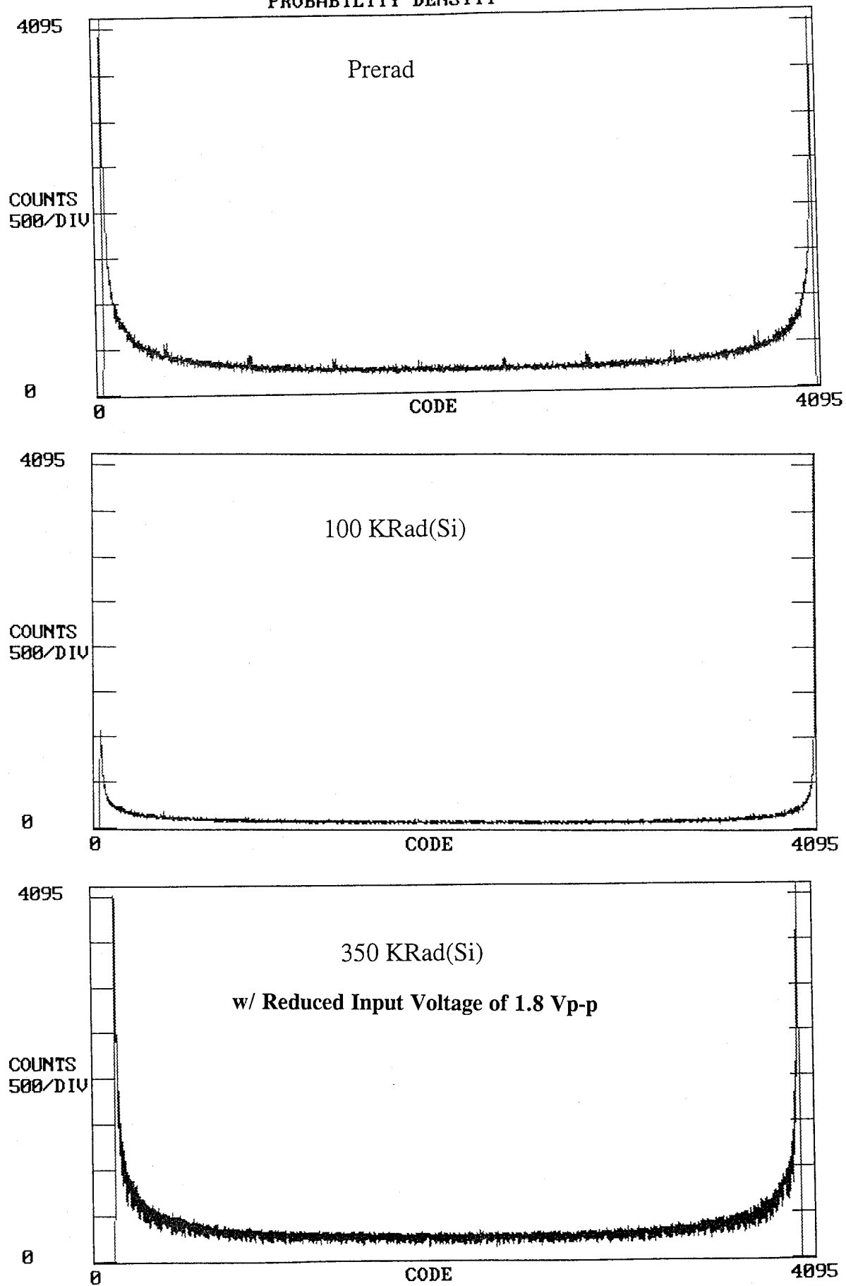
Figure 9. AD07 Histograms/(Using Internal Voltage Reference)
