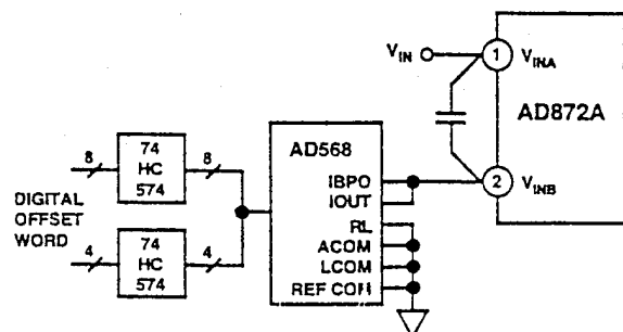
Figure 32. Offset Correction Using the AD568
