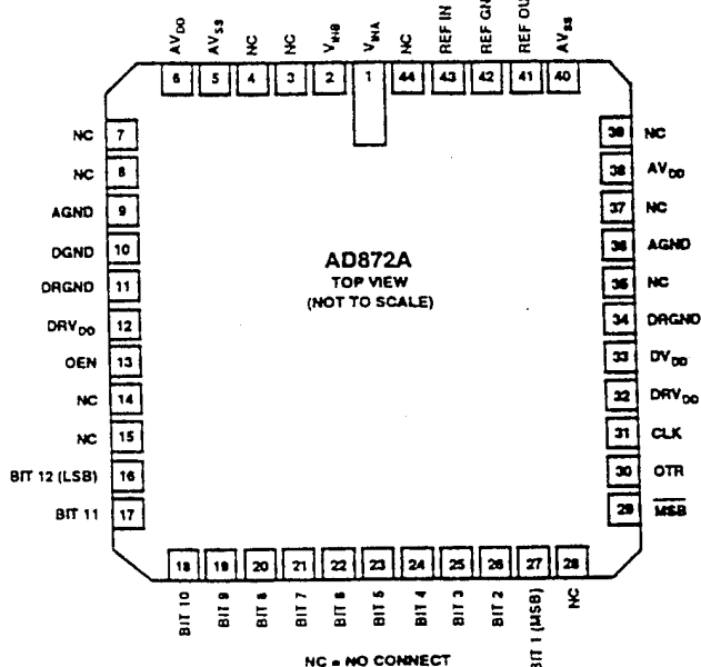
44-Pin LCC
