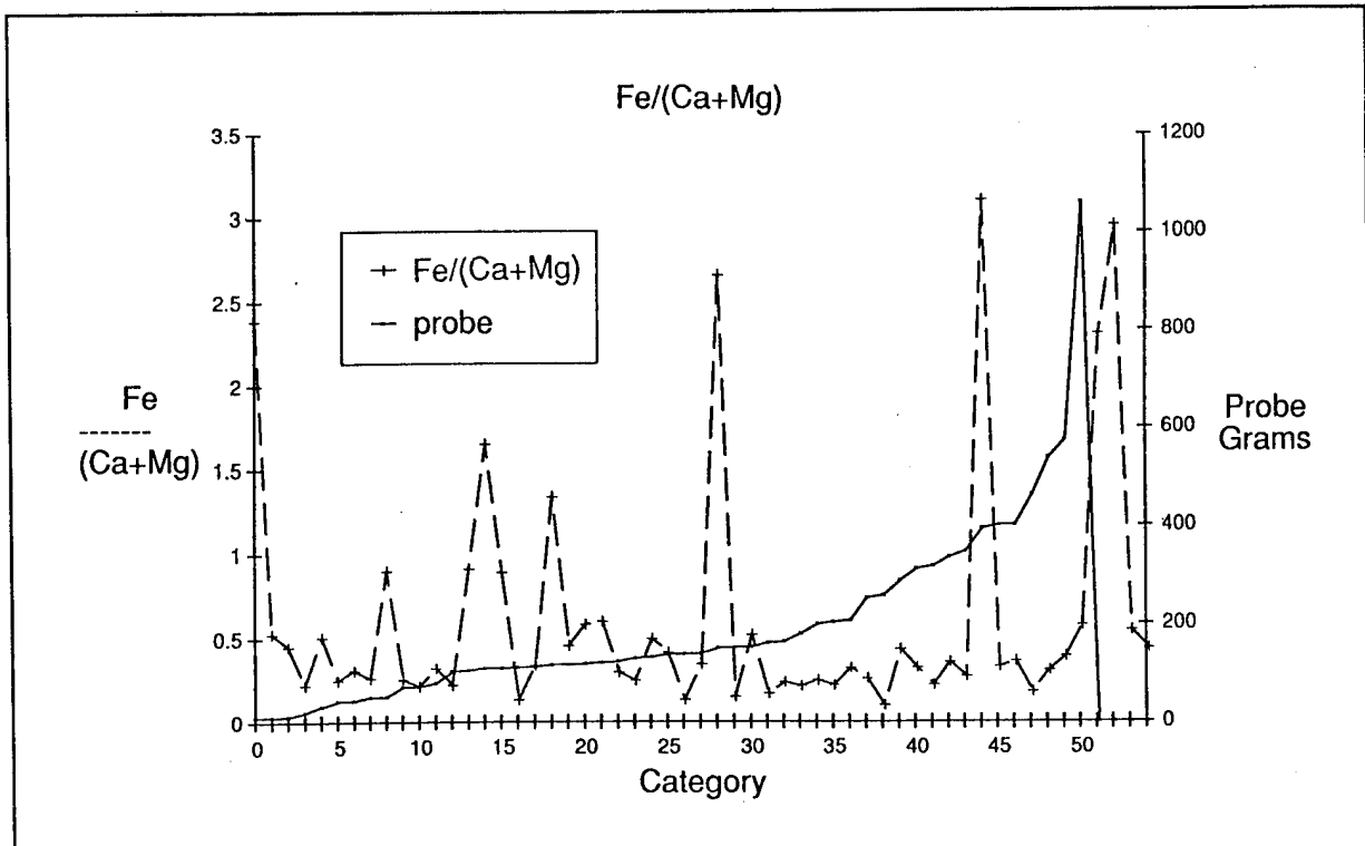
Figure 31. Correlation between the Fe 2 O 3 /(CaO + MgO) and probe weight.
