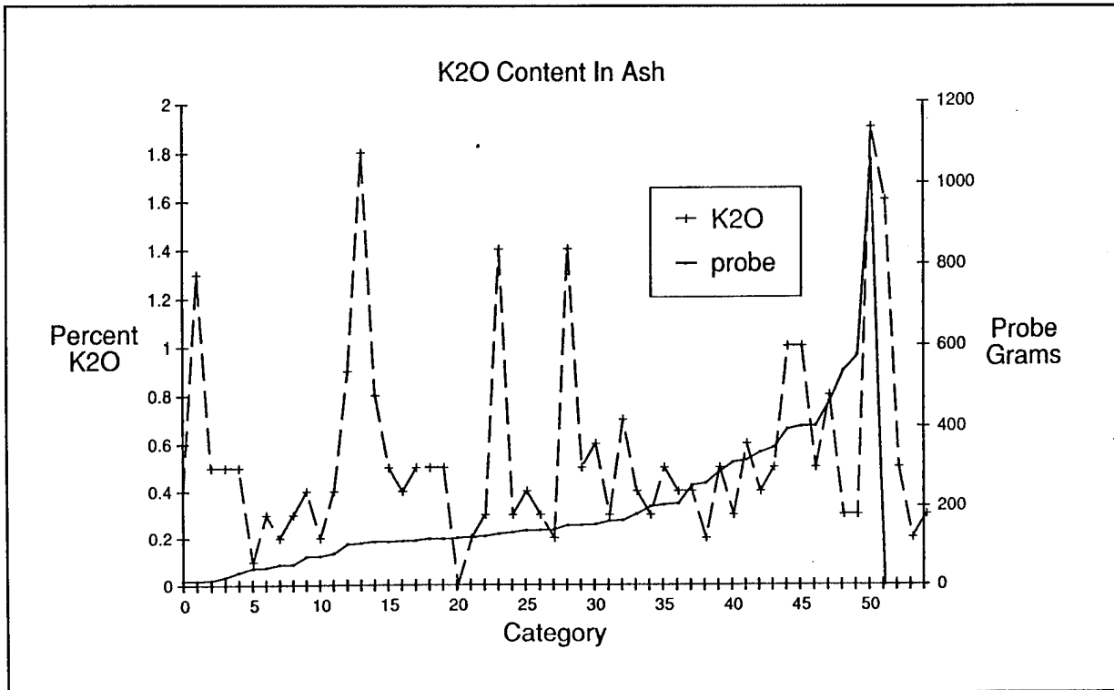
Figure 27. Correlation between fouling and K 2 O content in ash.
