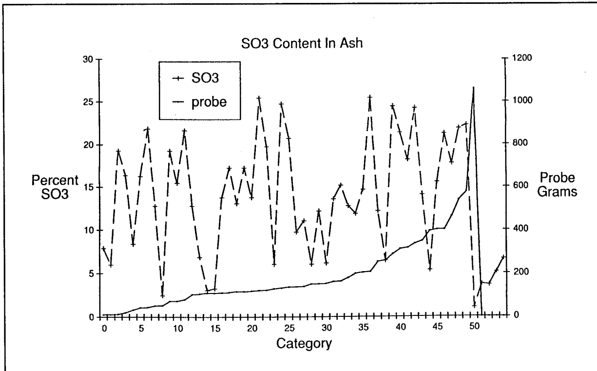
Figure 28. Correlation between fouling and SO 3 content in ash.
