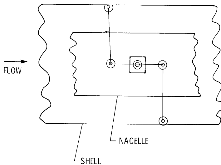
Figure 4.- Watts linkage.
