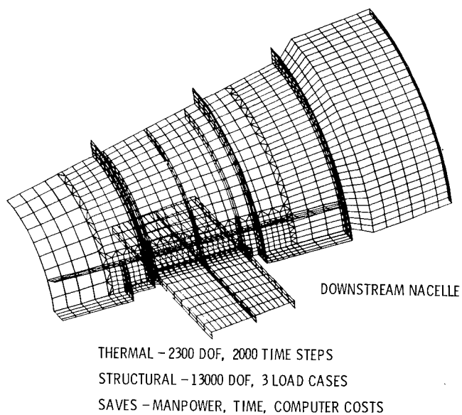
Figure 4.- SPAR integrated thermal-structural analysis key factor in NTF design.
