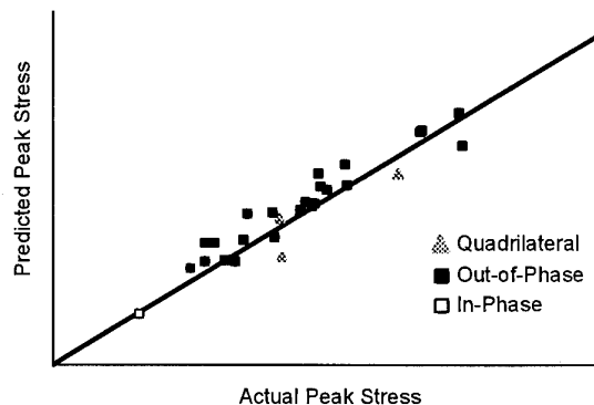
Figure 11. The simplified constitutive model predicted the peak stress of TMF cycles of strain controlled TMF specimens [3].
