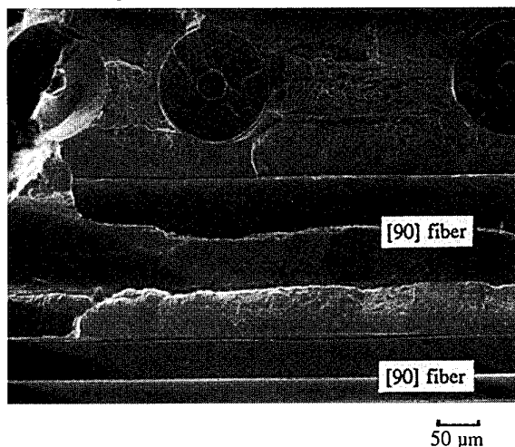
Fig. 12-SEM fractograph from [0/90] SiC-TMC under OP TMF: \Delta T=150\text{-}650^\circ\text{C} , S_{\text{max}}=300 MPa.
