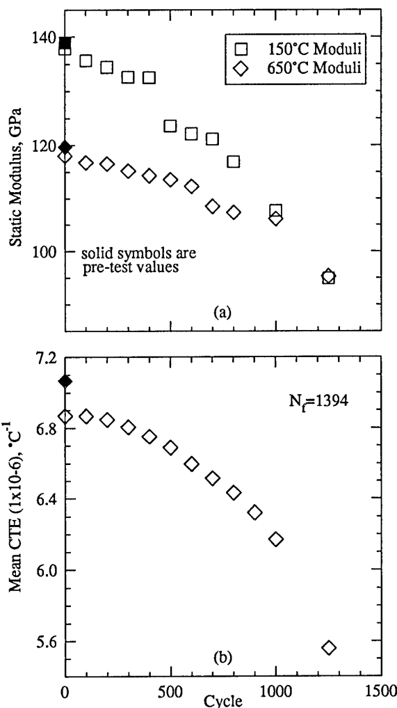
Fig. 13-Degradation of a) E and b) mean CTE during OP TMF of a [0/90] SiC-TMC: \Delta T=150\text{-}650^\circ\text{C} , S_{\text{max}}=300 MPa.
