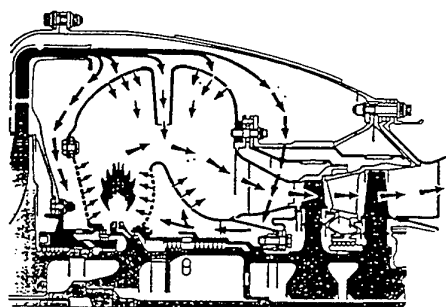
Figure 2 : a) Combustion chamber of an Arriel Engine (Centrifugal injection)
