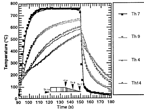
Figure 7 : Experimental and computed temperature profiles for FT-S geometry and aerospace thermal cycle.
